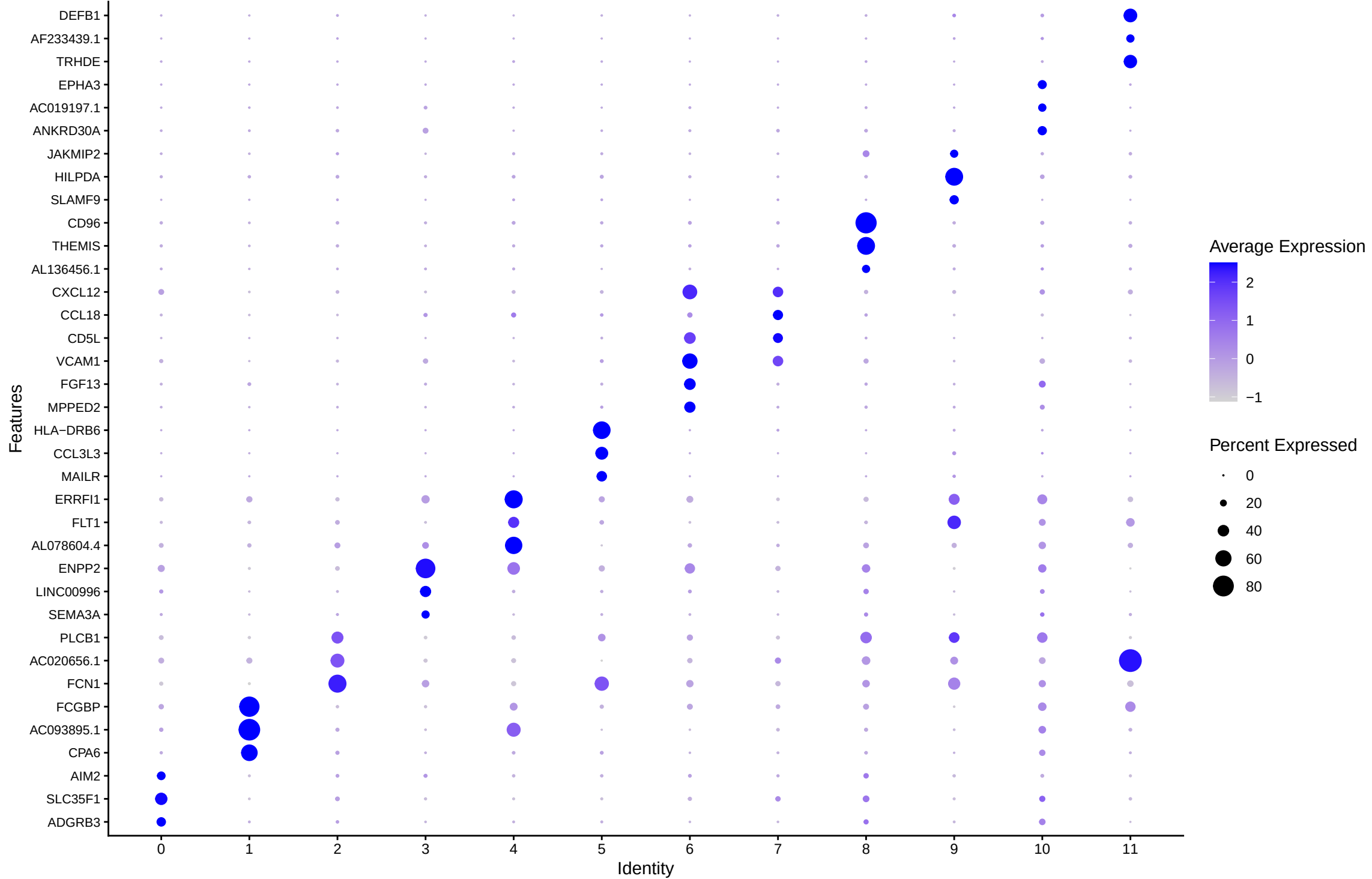
Top 3 DEGs per macrophage sub-cluster
