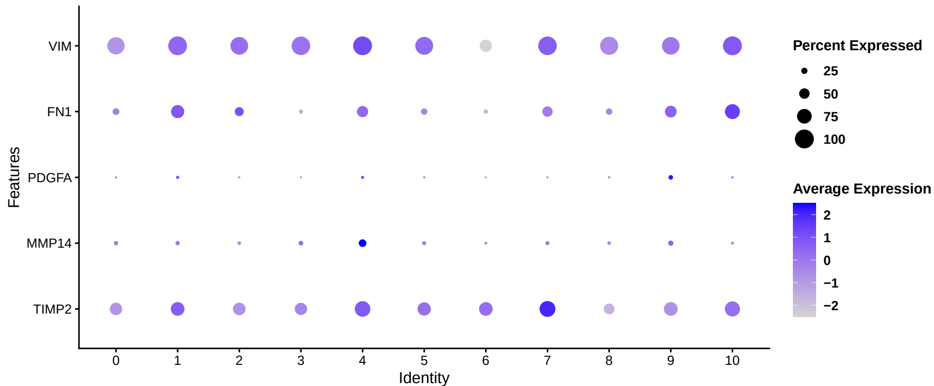
TIMP2/MMP14/PDGFA/FN1/VIM across macrophage sub-clusters
