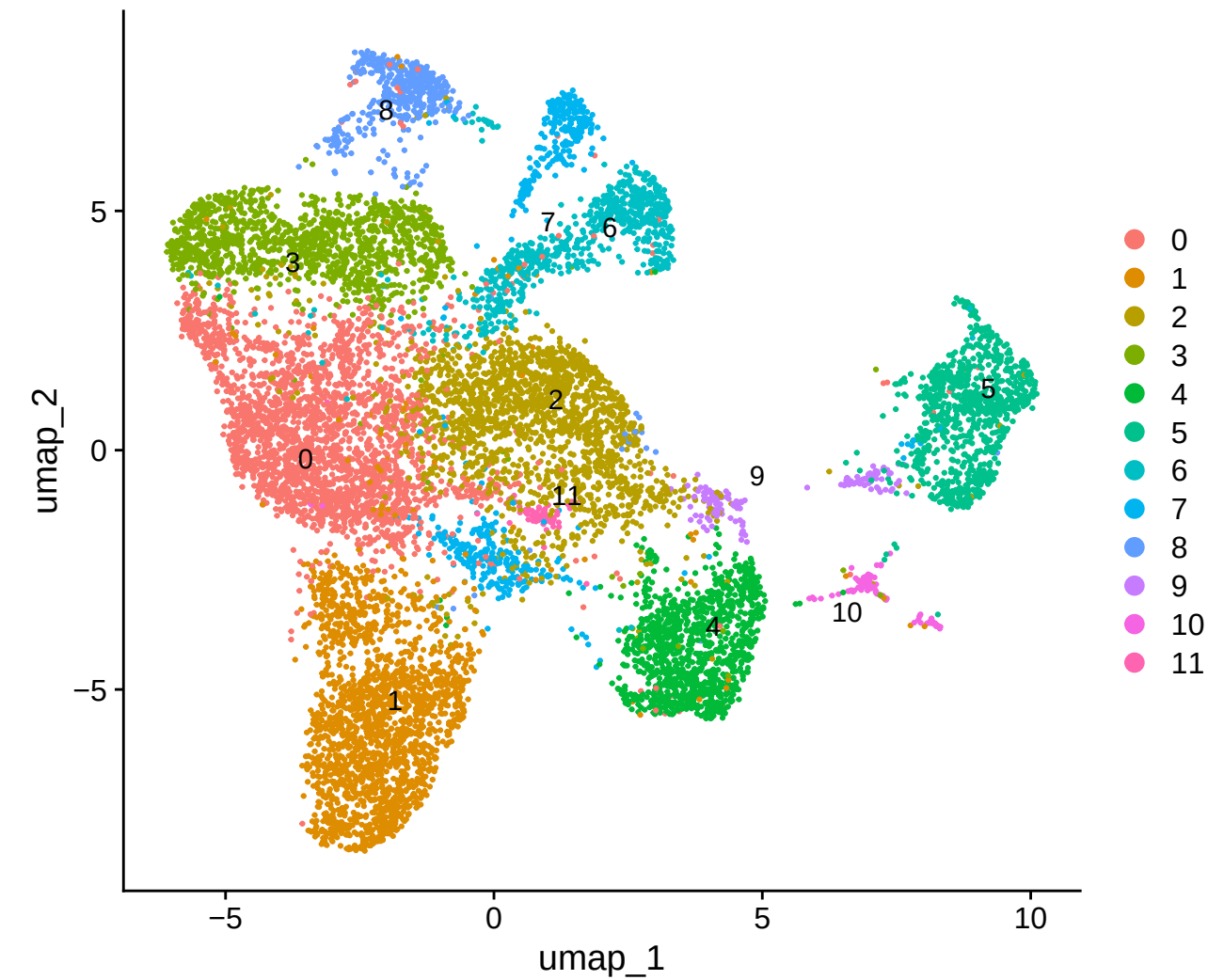
Macrophage sub-clusters (recomputed)
