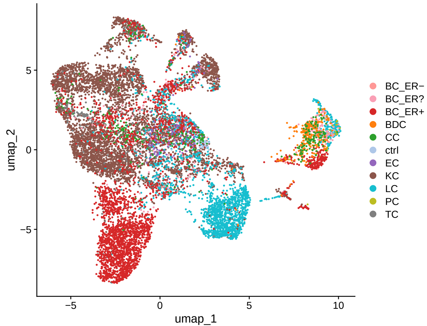
Cancer type (BC split by ER status from metadata)
