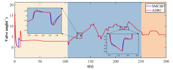
(a) Valve opening V_{\theta,1}
