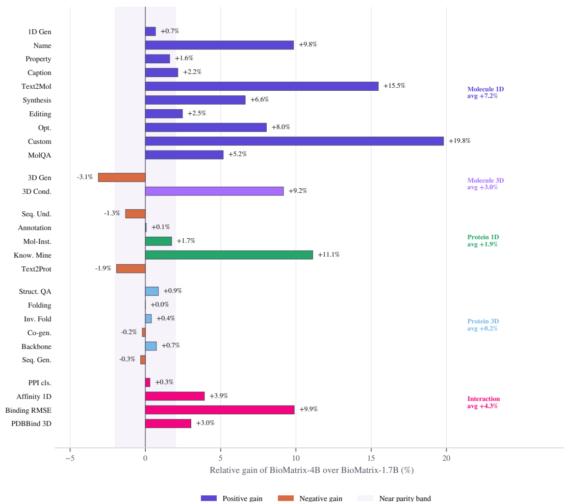
Figure 4: Relative gain from scaling BioMatrix from 1.7B to 4B. The score compares only the two BioMatrix scales: higher-is-better metrics use the relative score increase over BioMatrix-1.7B, while lower-is-better metrics use the corresponding relative error reduction.
