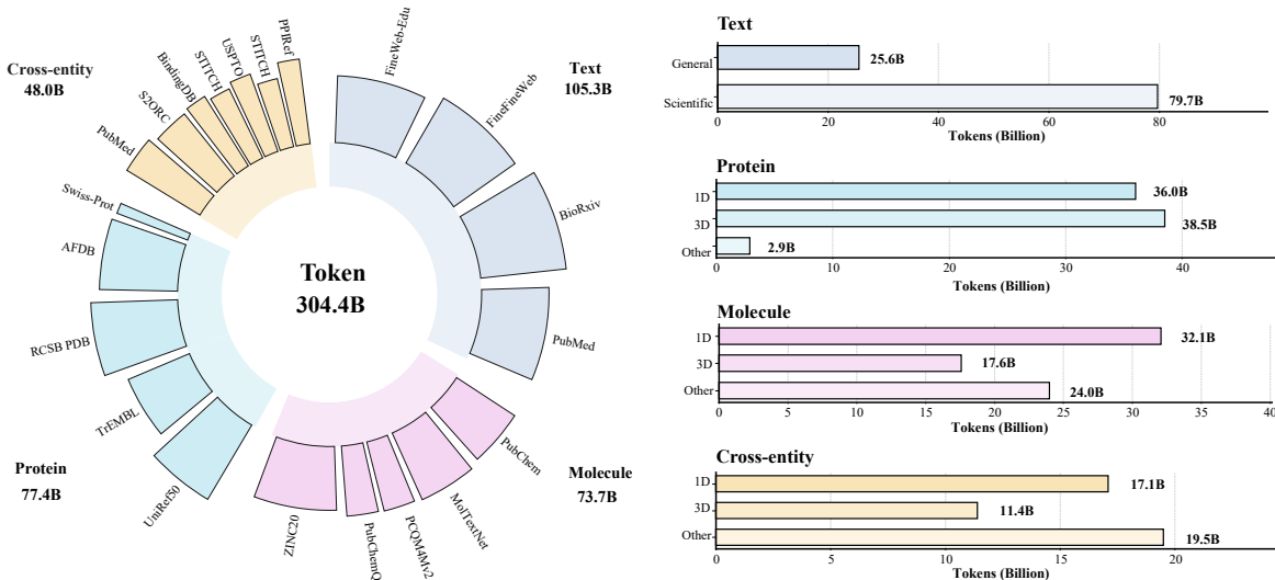
Figure 2: Overview of the continual pretraining corpus composition. Token budget distribution across four data categories — general and scientific text, molecule-centric data, protein-centric data, and cross-entity/interleaved data — spanning 1D, 3D, and textual modalities, totaling 304.4 billion tokens.
