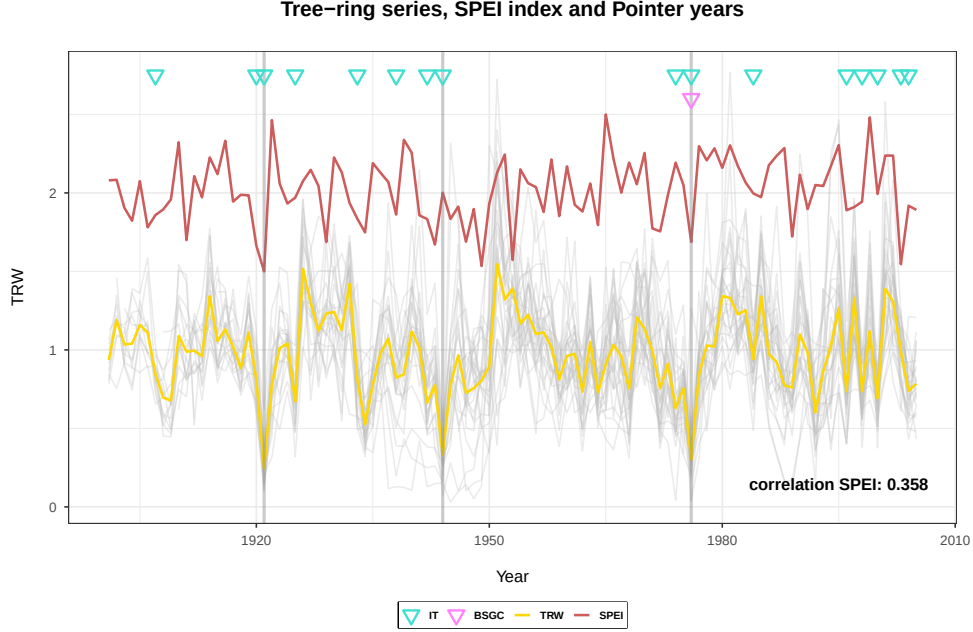
Figure 1: Dendrochronological site series showing individual detrended growth series (gray), the site master chronology (yellow), the annual aggregation of the SPEI1 climatic index (red), and the detected pointer years using the Interval Trend method (turquoise) and BSGC (pink).
