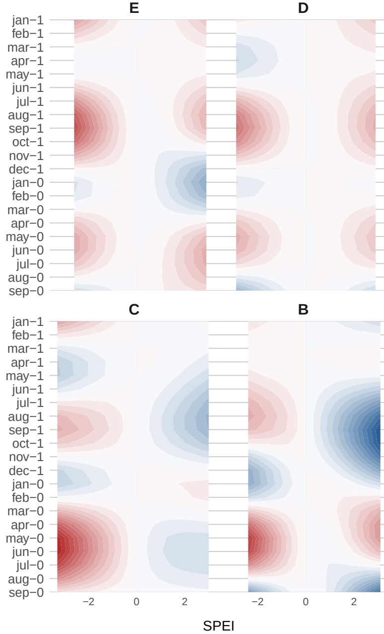
Figure 10: Estimated coefficient surfaces from the cross-basis matrix of the SPEI index across different monthly lags relative to growth for each considered geographical macro-area for the genus Pinus . Brighter colors represent a higher coefficient value. Red indicates a negative effect, while blue represents a positive effect on radial growth.
