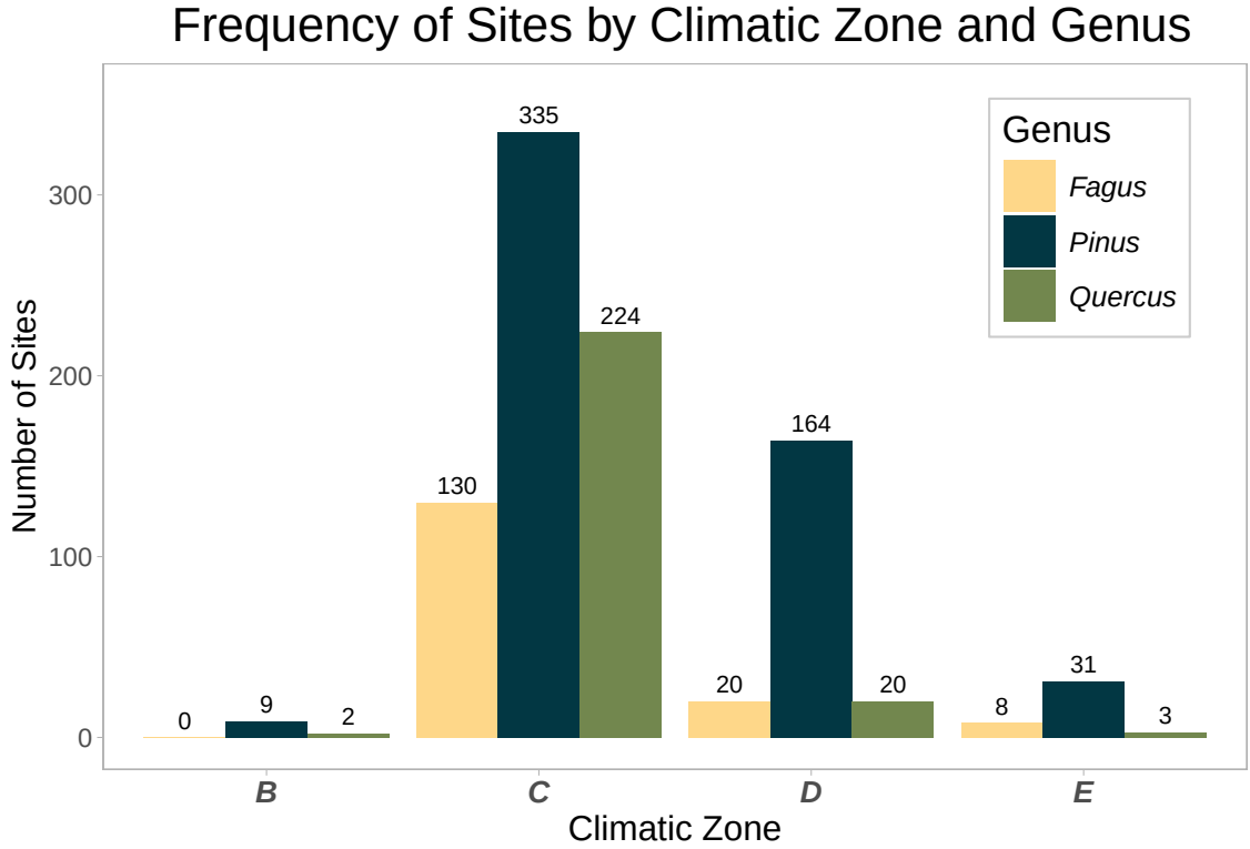
Figure 4: Sample frequency: Number of sites per genus Pinus spp., Quercus spp., and Fagus sylvatica and per climate zone: arid zone (B), temperate zones (C), continental zone (D), and polar zone (E).
