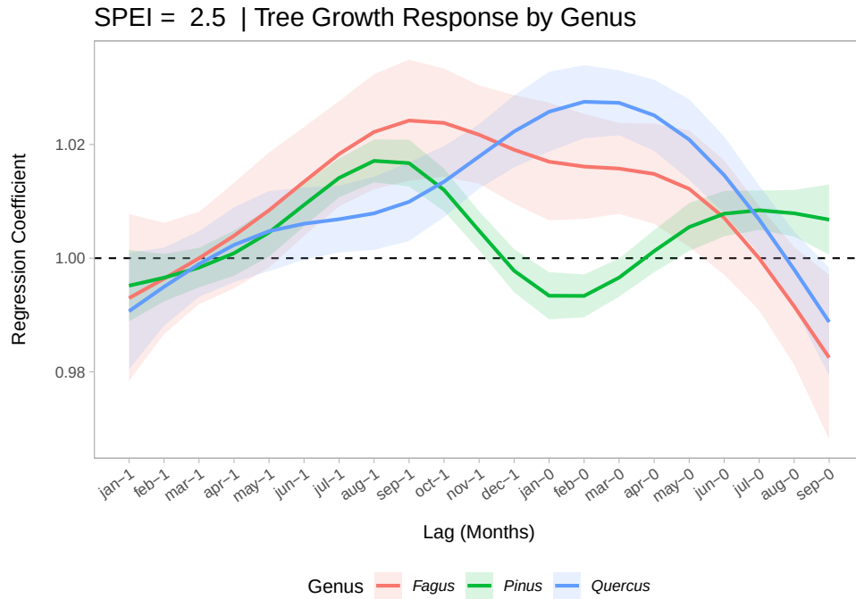
Figure 9: Lag-response curves representing two-dimensional slices of the response surface at a fixed SPEI value of +2.5 (water abundance) with 95% confidence intervals, stratified by tree genus.
