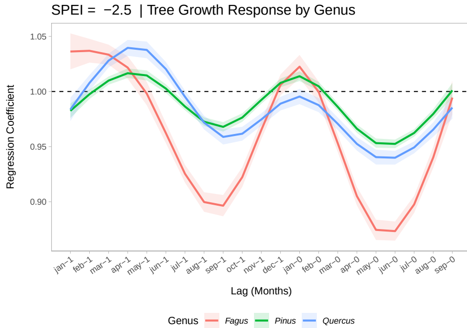
Figure 8: Lag-response curves representing two-dimensional slices of the response surface at a fixed SPEI value of -2.5 (extreme drought) with 95% confidence intervals, stratified by tree genus.
