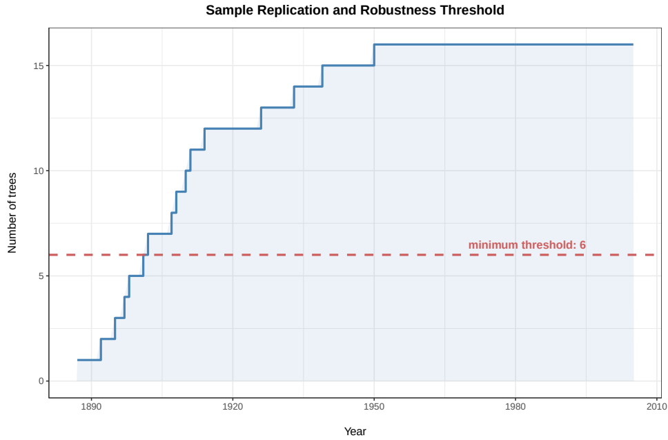
Figure 2: Sample depth graph of the series for the site represented in ???. The plot shows the years in which all series from the site present a radial growth value. The red dashed line indicates when the sample reaches the threshold of 6 trees (corresponding to 12 series) with concurrent observations.
