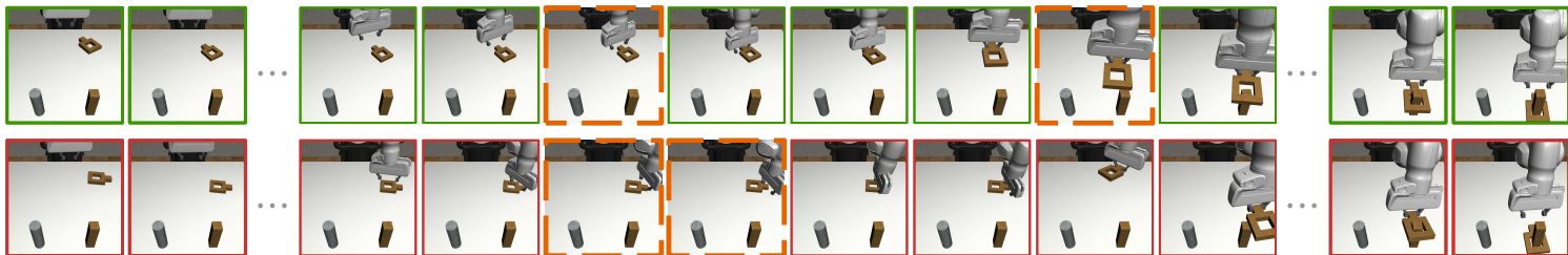
Square
