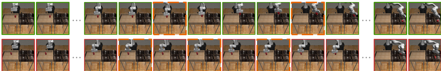
Can
