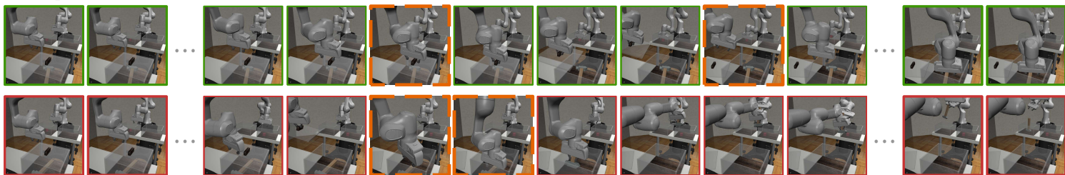
Transport
