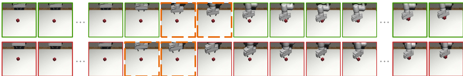
Lift
