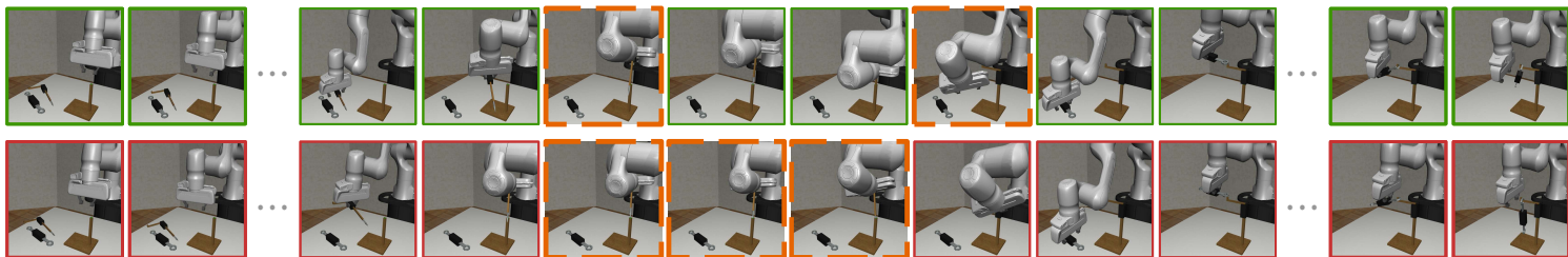
Tool Hang
