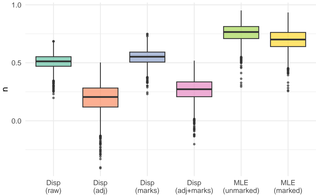
Branching Ratio ( n ) Across Methods
