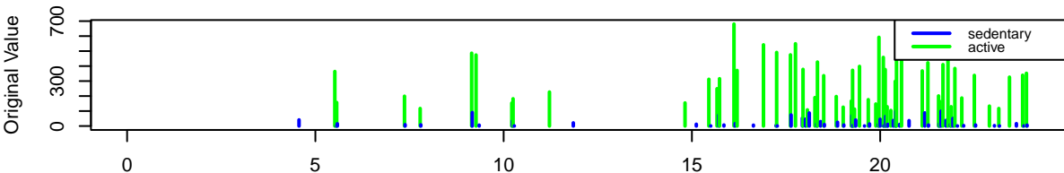
Subject 40583 – Weekday Sun – Marked Hawkes Events
