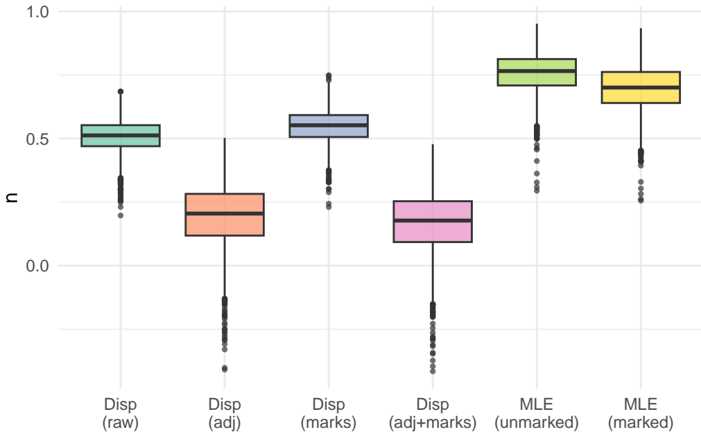
Branching Ratio (n) Across Methods
