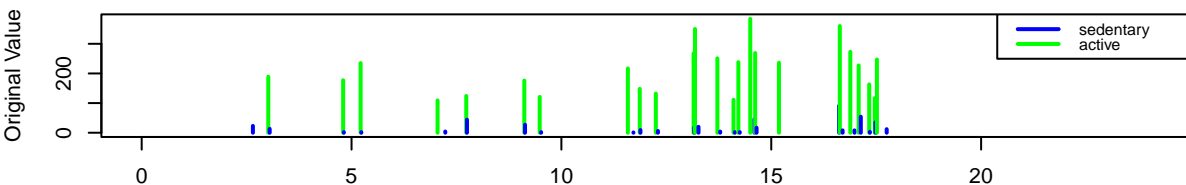
Subject 40583 – Weekday Sat – Marked Hawkes Events
