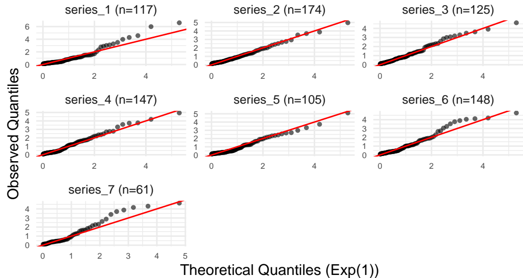
Q-Q Plots by Series
