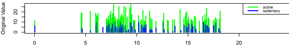
Subject 64161 – Weekday Wed – Marked Hawkes Events
