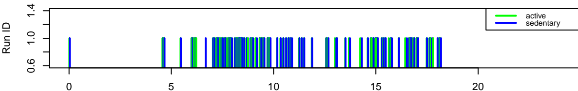
Subject 64161 – Weekday Wed – Event Types (Categories)
