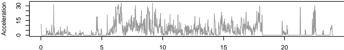
Subject 64161 – Weekday Wed – Raw Activity Data
