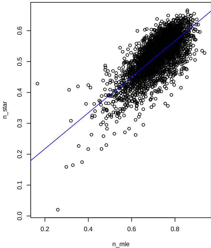
n ( r=0.742 )
