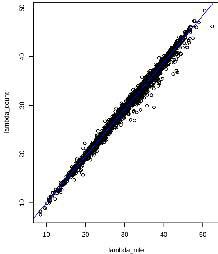
lambda ( r=0.995 )
