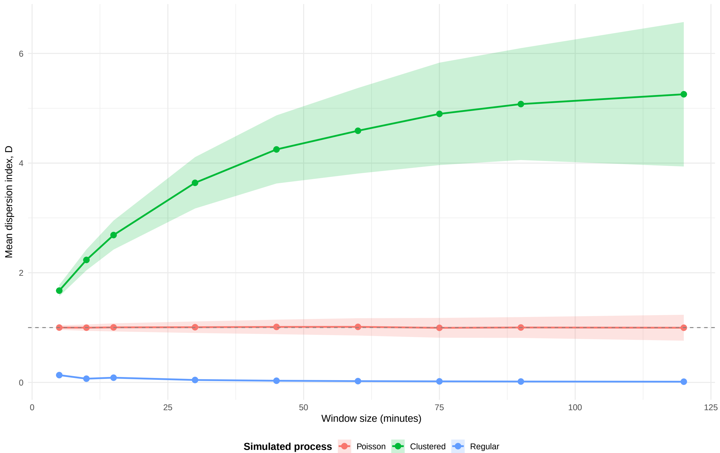
Dispersion Index Across Simulated Process Types
