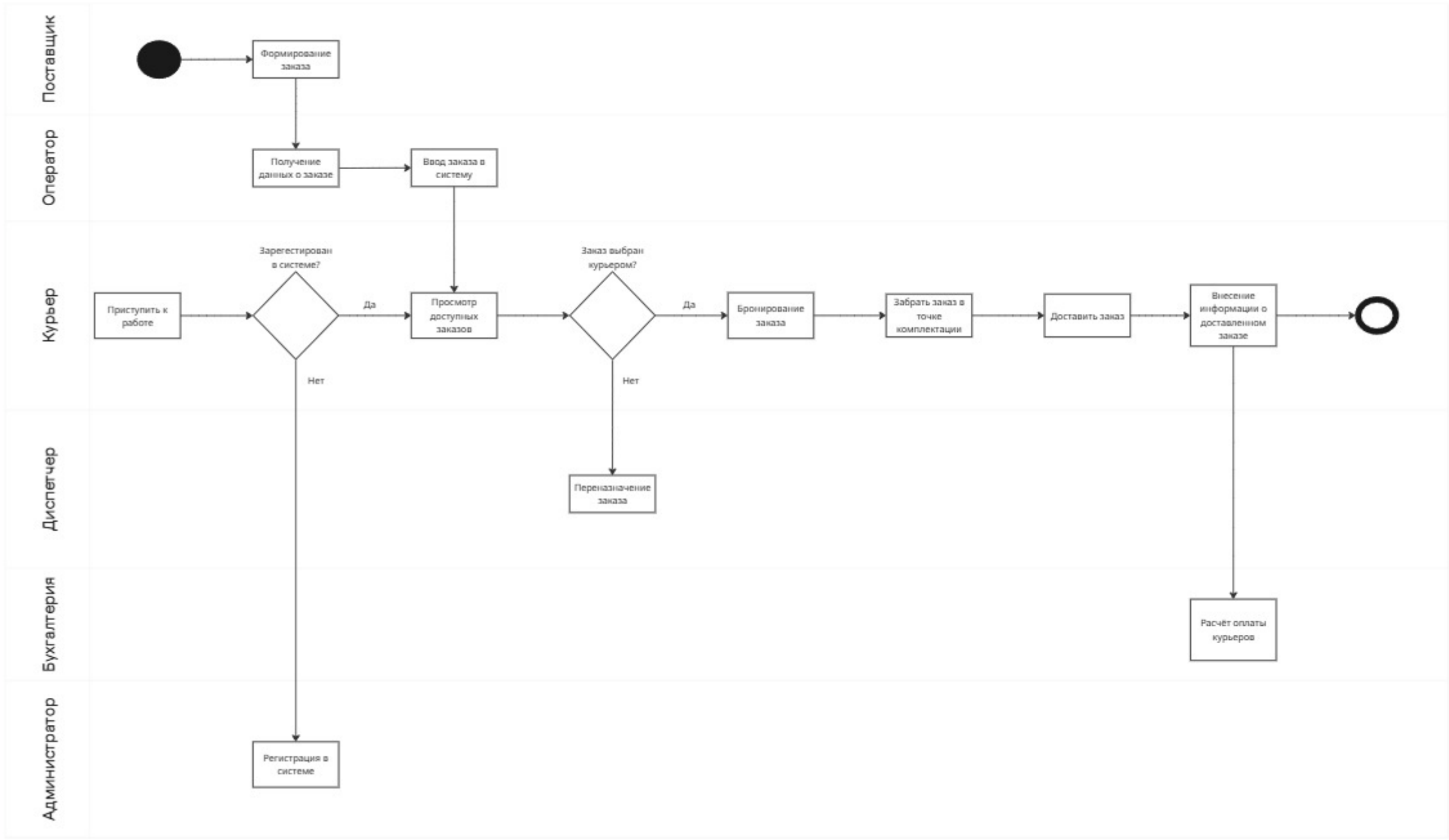
Swimlane diagram
