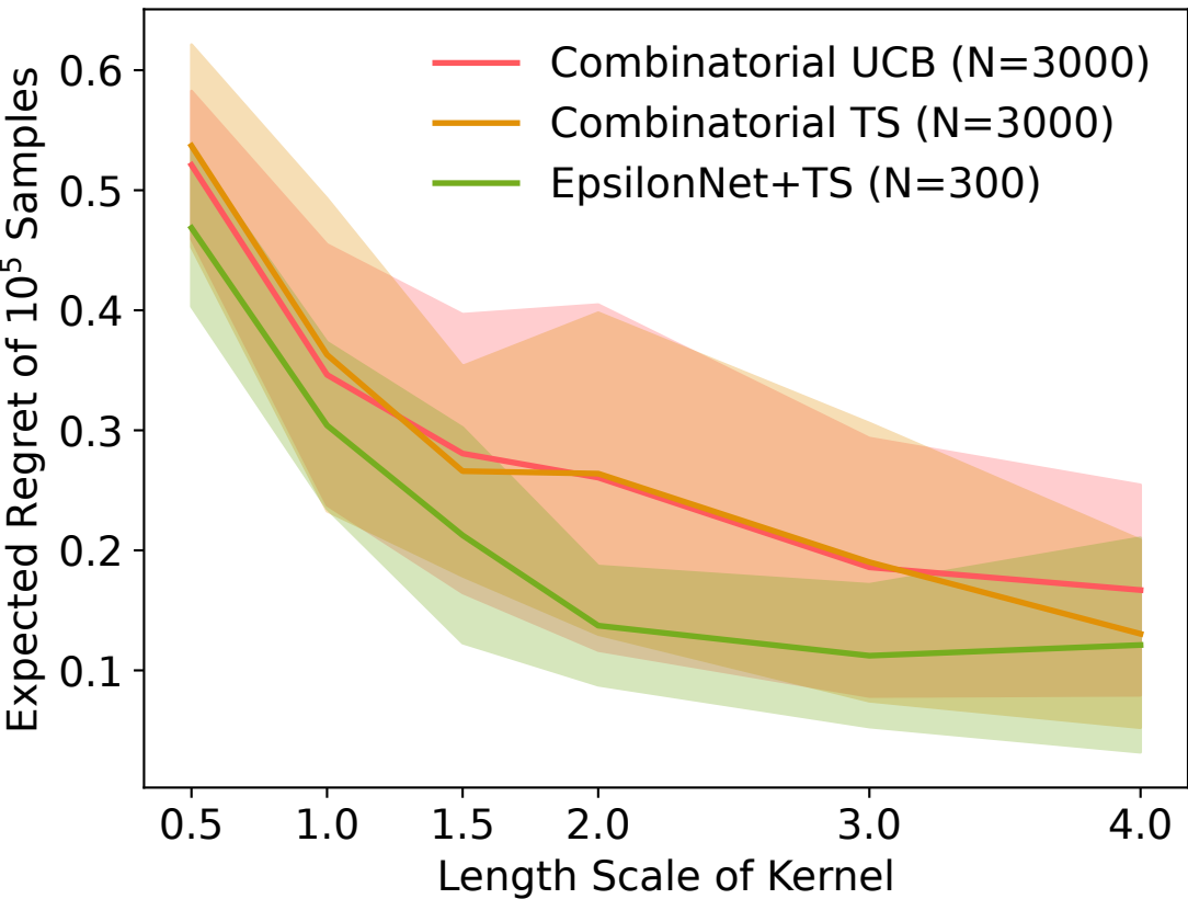
Performance of K=10 out of 500 Actions
