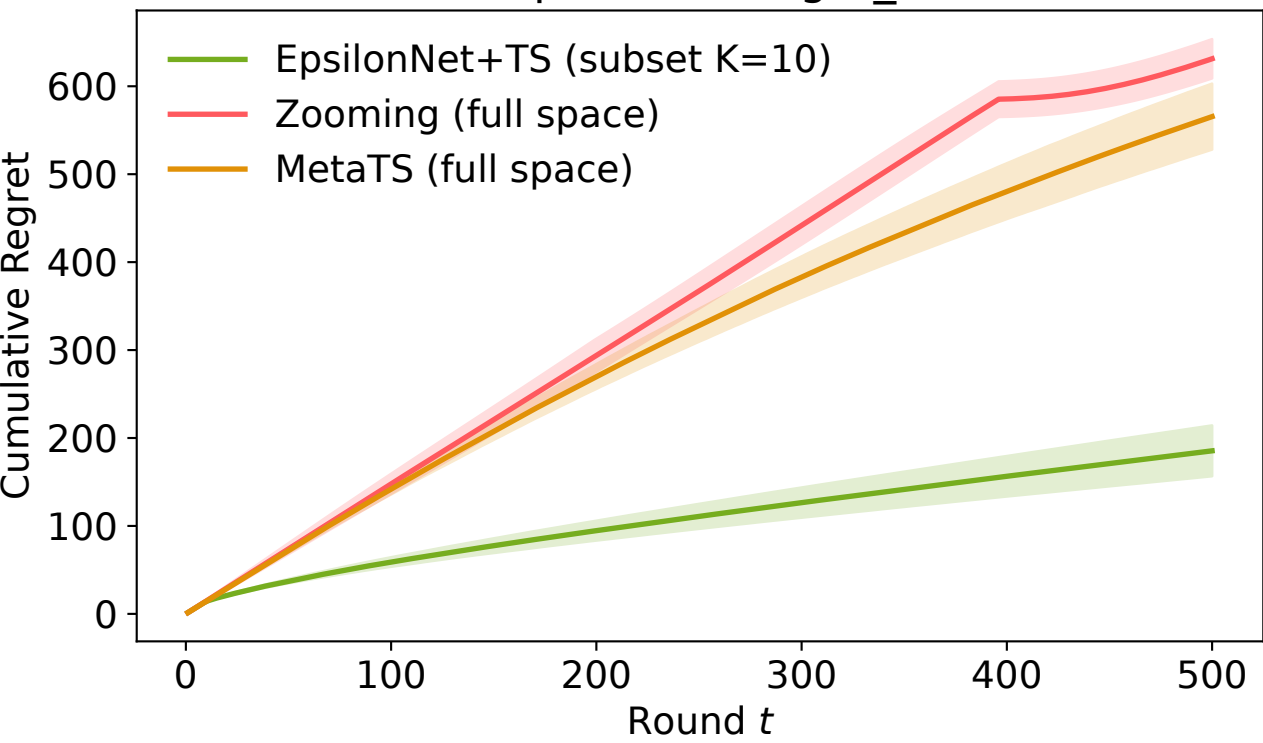
Online Bandit Comparison (length_scale=1.0, K=10)
