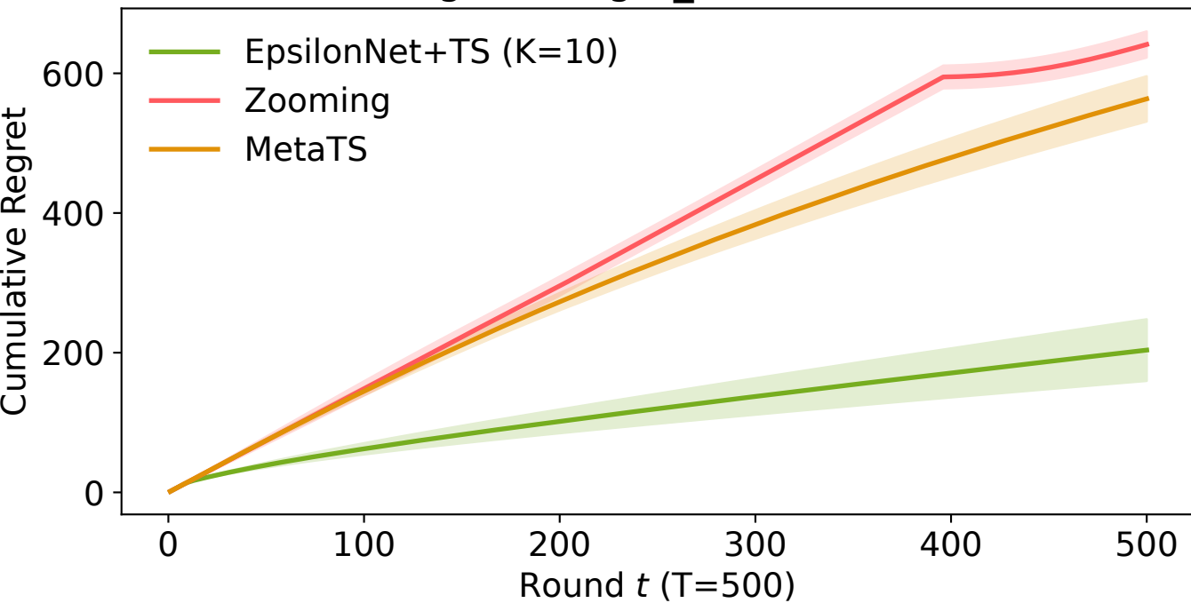
Online Regret (length_scale=1.0, N=500)
