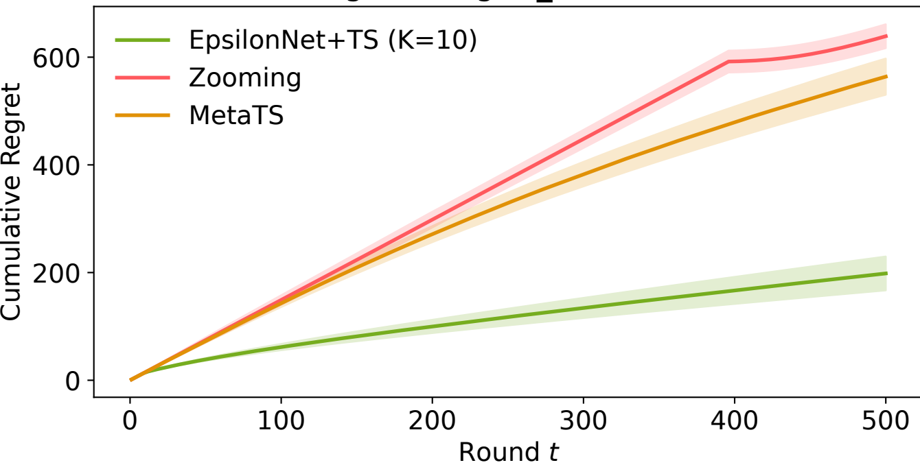
Online Regret (length\_scale=1.0, K=10)
