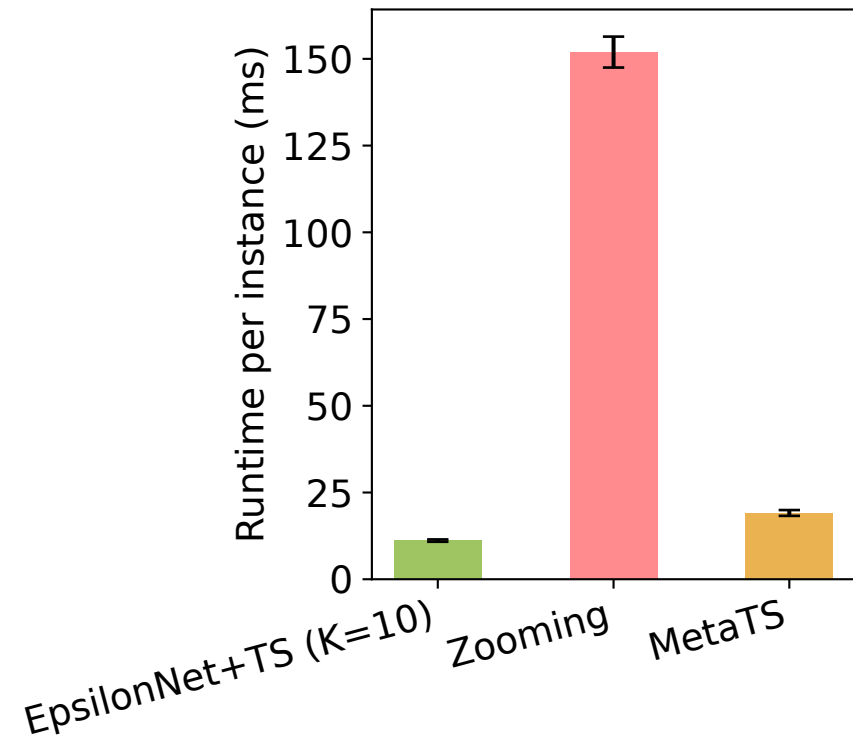
Downstream Runtime (T=500)
