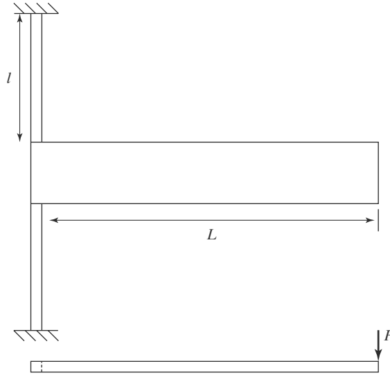
FIGURE 3.23 A torsional supported cantilever.
