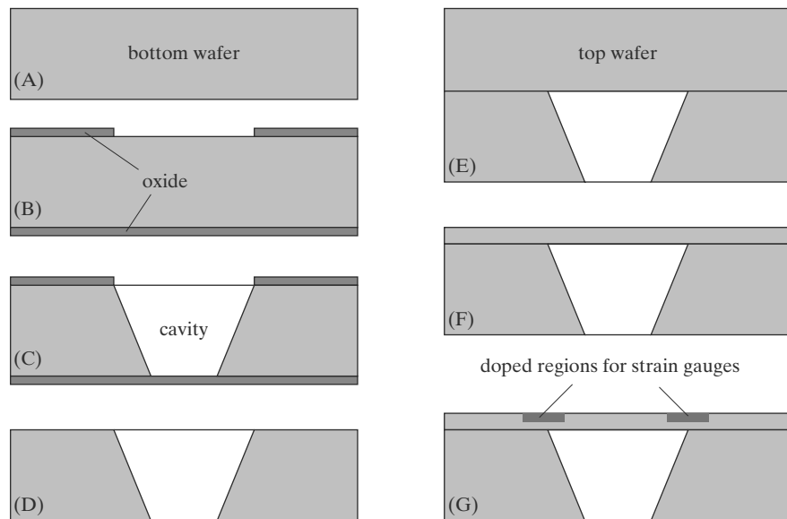
FIGURE 2.21 Pressure sensor fabrication process.
