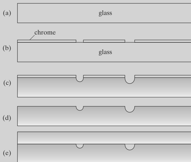
FIGURE 14.10 Microfabrication technique.
