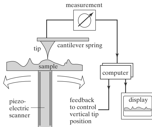
FIGURE 12.12 A generic diagram of an SPM.
