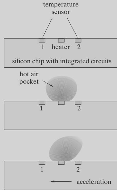
FIGURE 5.13 Principle of thermal-transfer based accelerometer.
