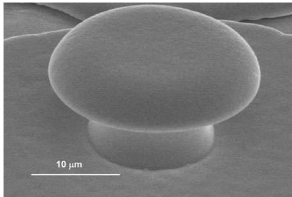
FIGURE 8.7 Mushroom shaped electroplated metal, revealed after the electroplating mold is removed.
