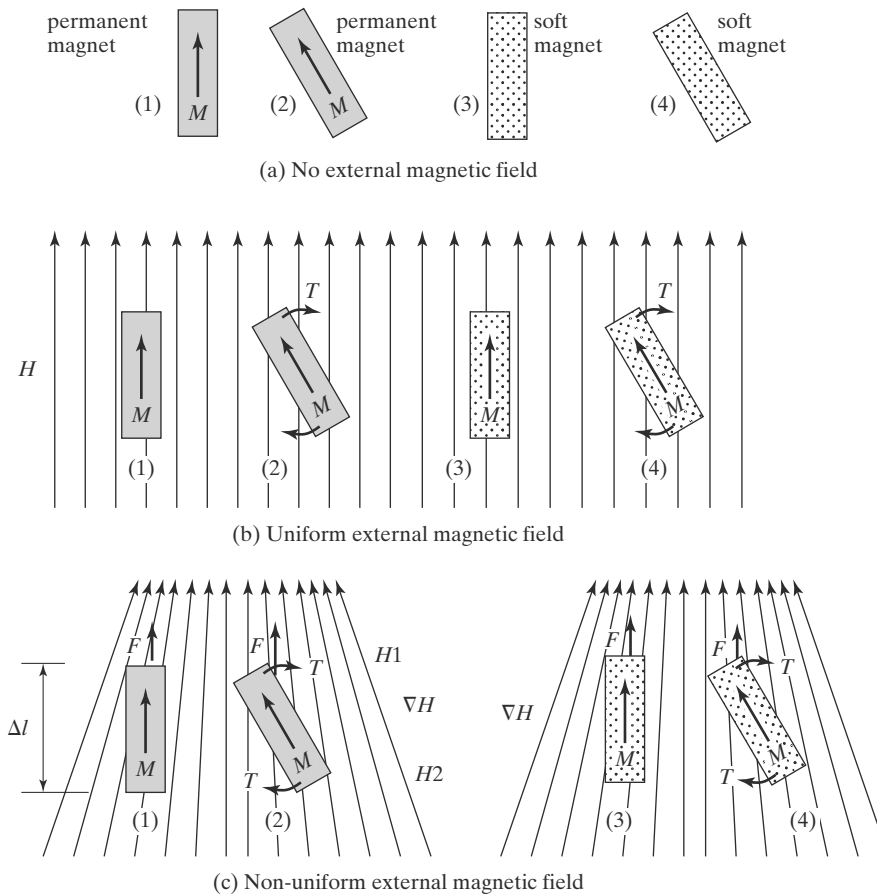
FIGURE 8.5 Magnetization states and force states in magnetic fields. Net magnetic forces ( F ) and moment ( T ) are indicated for each piece under each biasing case.
