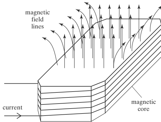
FIGURE 8.8 Magnetic field line distribution of a solenoid magnet.
