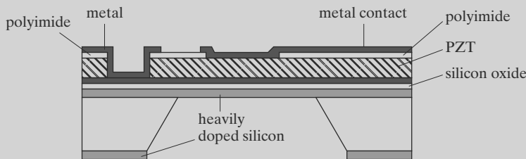
FIGURE 7.7 Schematic diagram of a piezoelectric microphone.
