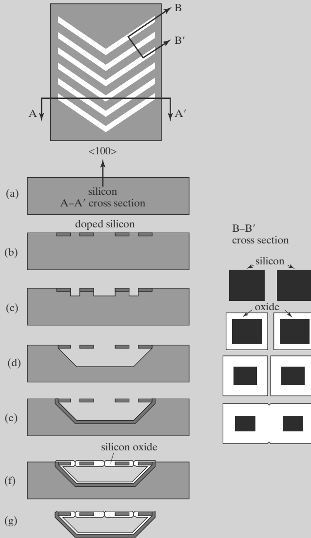
FIGURE 14.11 Fabrication process of embedded micro channels.
