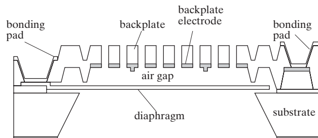
FIGURE 15.6 Sideview of a MEMS chip in the Knowles microphone.
