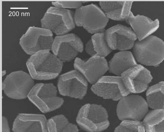
FIGURE 10.26 SEM micrograph of loose micro pyramids. (Courtesy: Prof. Teri Odom, Northwestern University)
