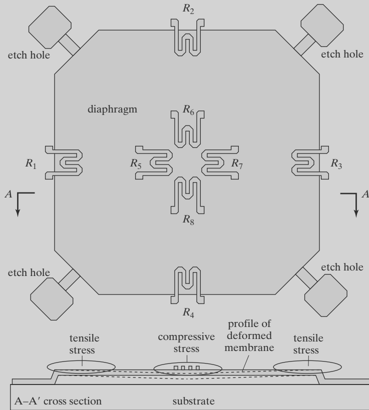
FIGURE 6.14 Top and cross-sectional view of a surface micromachined pressure sensor.
