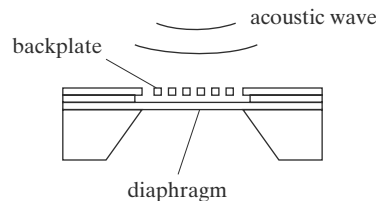
FIGURE 15.4 Schematic diagram of a condenser microphone.
