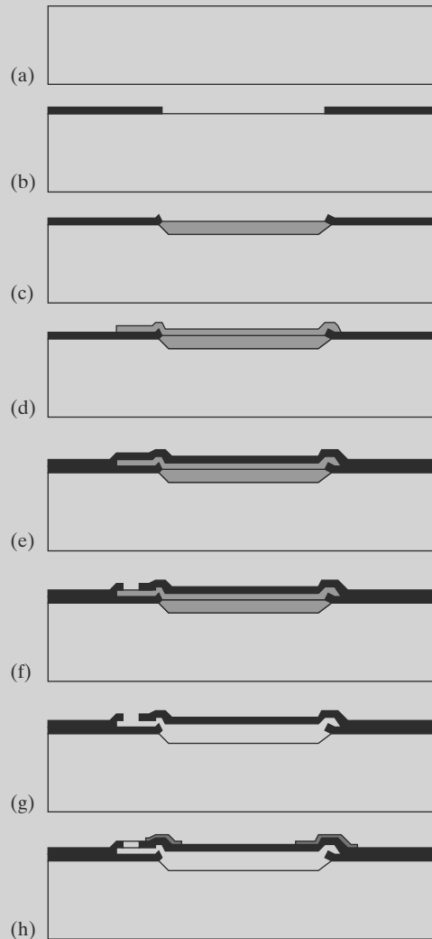
FIGURE 6.15 Fabrication process for surface micromachined sensor.
