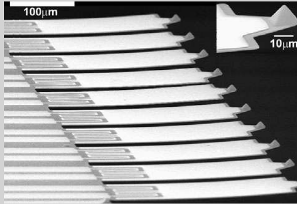
FIGURE 12.26 SEM micrograph of an active DPN array.
