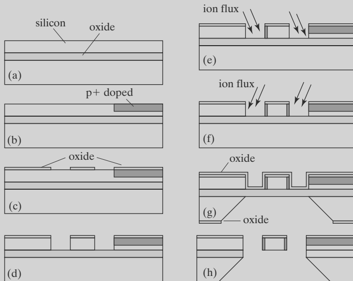
FIGURE 6.13 Fabrication process along A-A' cross section of Figure 6.12.
