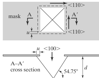
FIGURE 10.7 Cross-sectional view of etched cavity.
