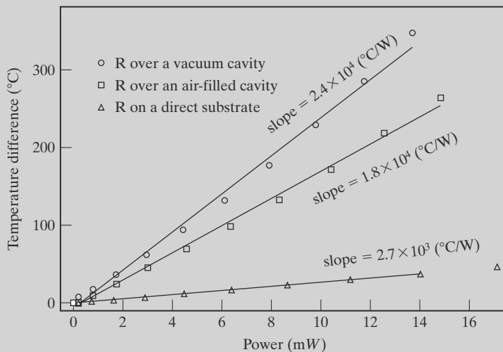
FIGURE 5.27 Temperature vs. input power.
