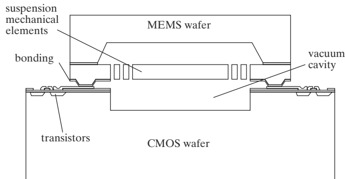
FIGURE 15.16 Gyroscope configuration.
