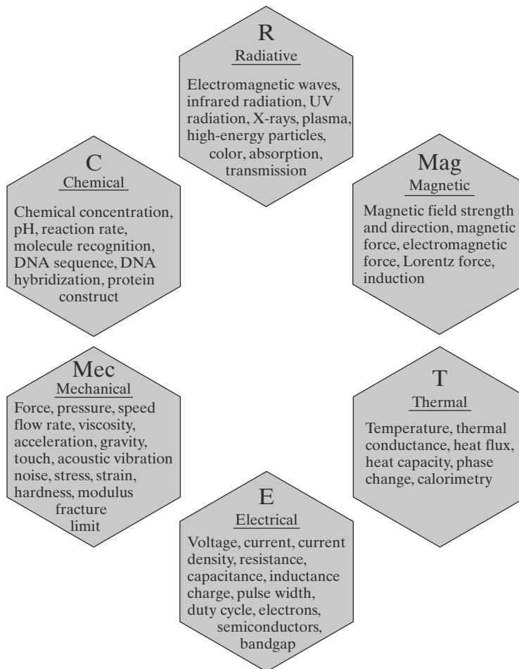
FIGURE 1.7 Major energy domains.
