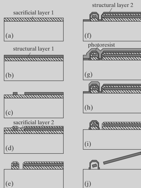
FIGURE 11.5 The fabrication process for a three-dimensional hinge.
