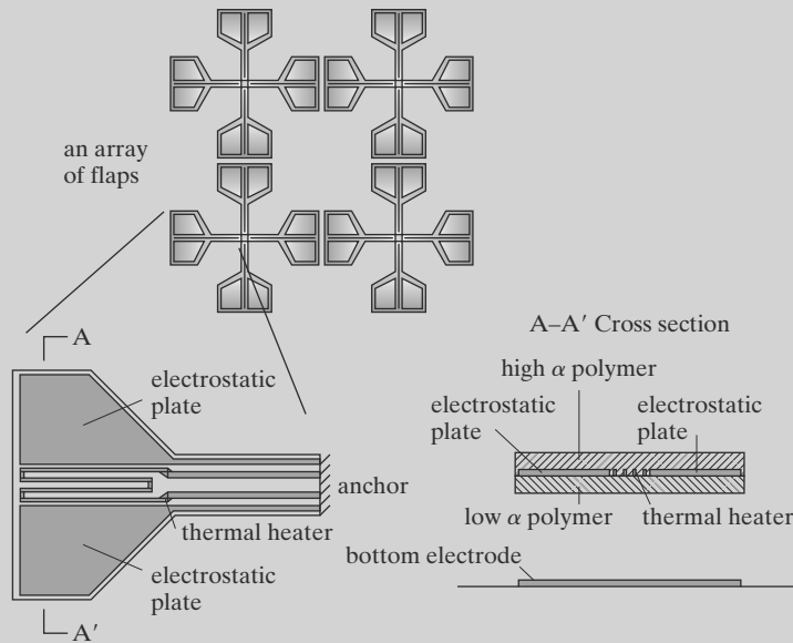
FIGURE 5.7 Polyimide thermal actuator.
