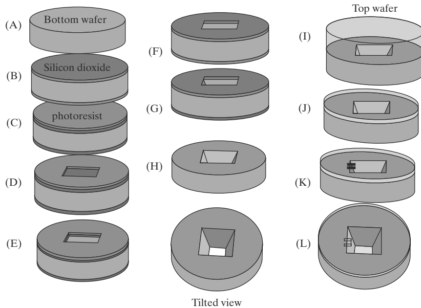
FIGURE 2.20 Process for a micromachined pressure sensor.
