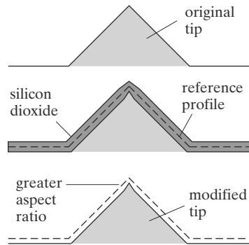
FIGURE 12.16 Tip sharpening process.
