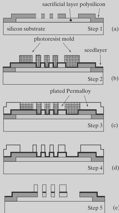
FIGURE 8.15 Fabrication process.
