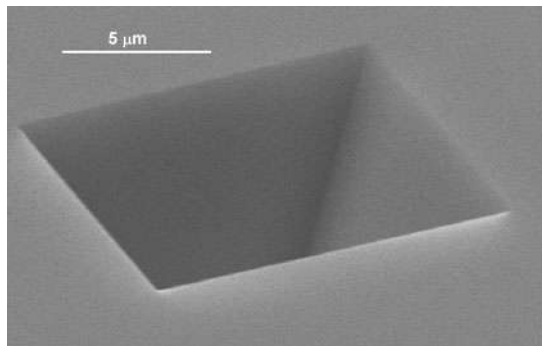
FIGURE 10.2 SEM micrograph of an inverted cavity.
