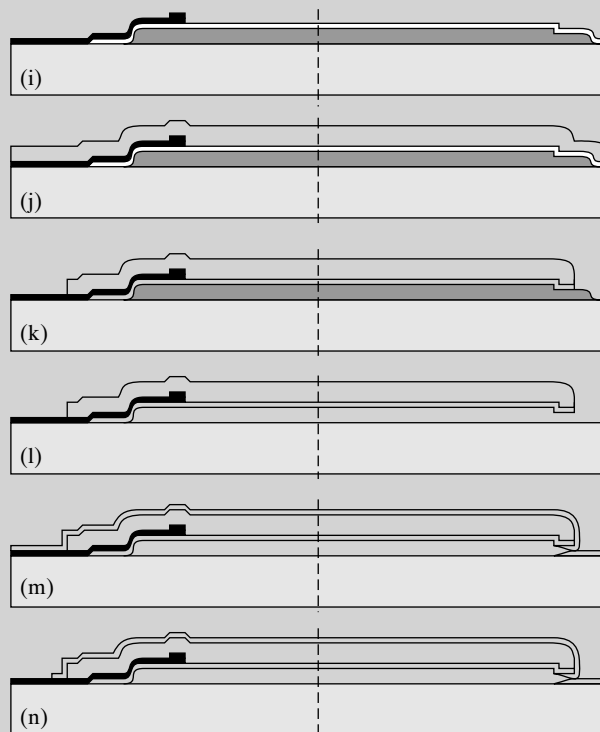
FIGURE 13.7 Final six steps (i through n) in the fabrication process of Parylene membrane.
