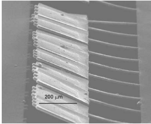
FIGURE 3.24 Microscale devices bent under intrinsic stress.
