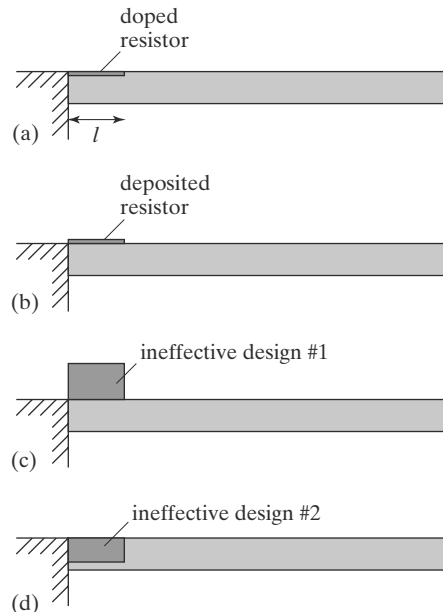
FIGURE 6.6 Designs of cantilevers with piezoresistor.
