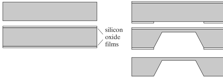
FIGURE 12.8 Method for forming silicon diaphragm.
