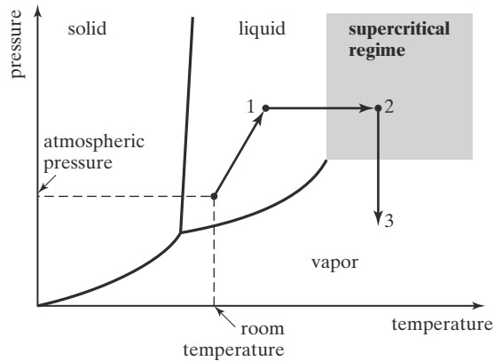
FIGURE 11.10 Carbon dioxide super critical drying.
