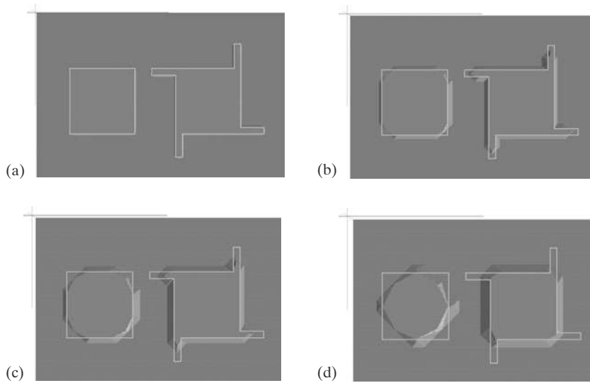
FIGURE 10.16 Progression of mesas from two mask patterns. Frames (a) through (d) correspond to etch pro- files at 5, 20, 30, and 39 minutes.
