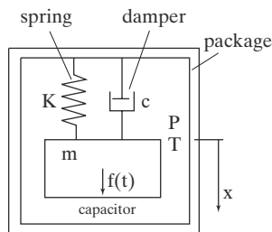
FIGURE 3.29 A mass-spring-damper system.
