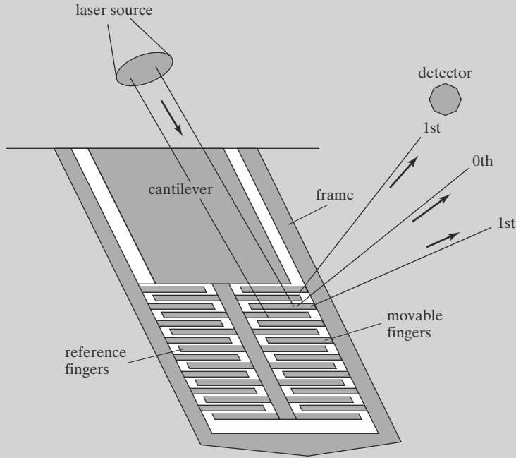
FIGURE 9.6 Interdigitated cantilever.
