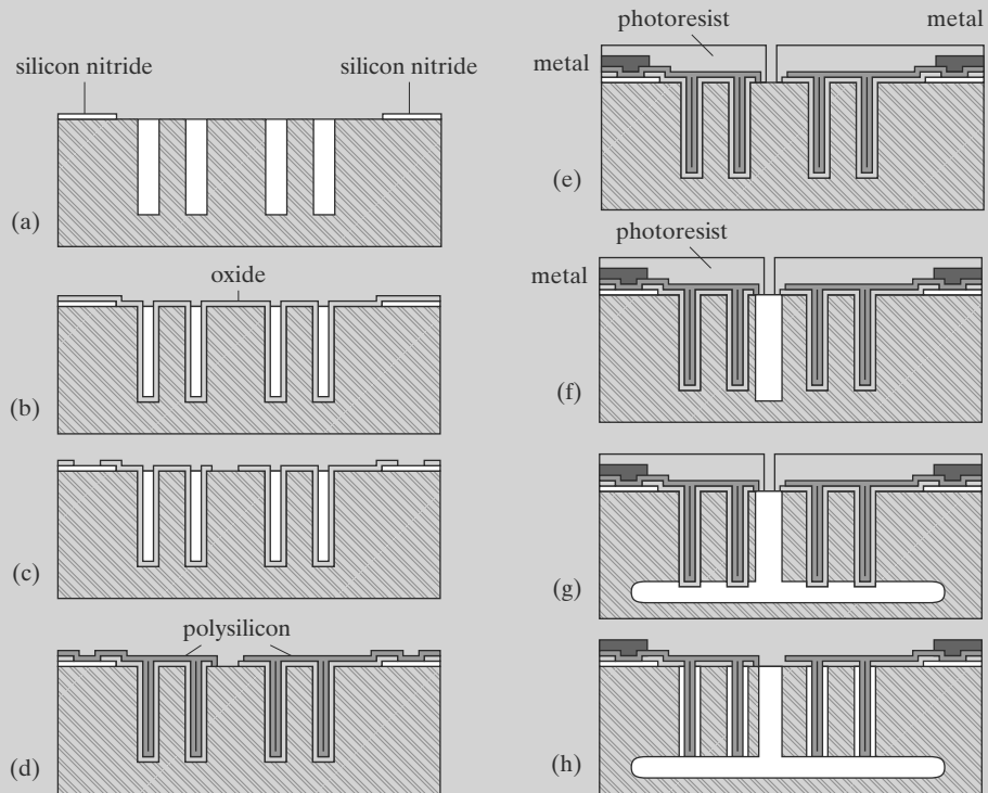
FIGURE 12.4 HARPSS process flow.
