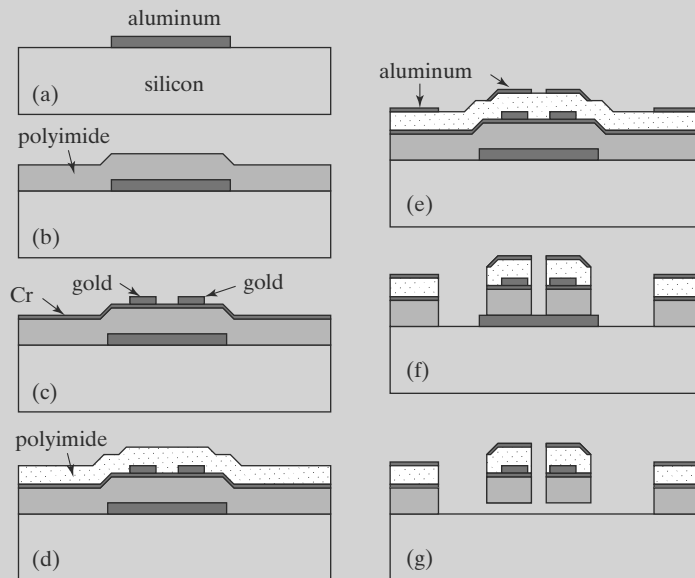
FIGURE 5.6 Fabrication process depicted in the A-A' cross section.
