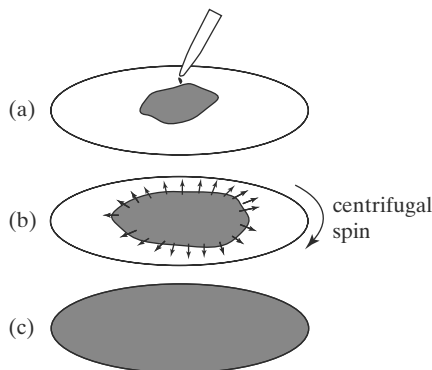
FIGURE 2.6 Process steps of photoresist spin coating.
