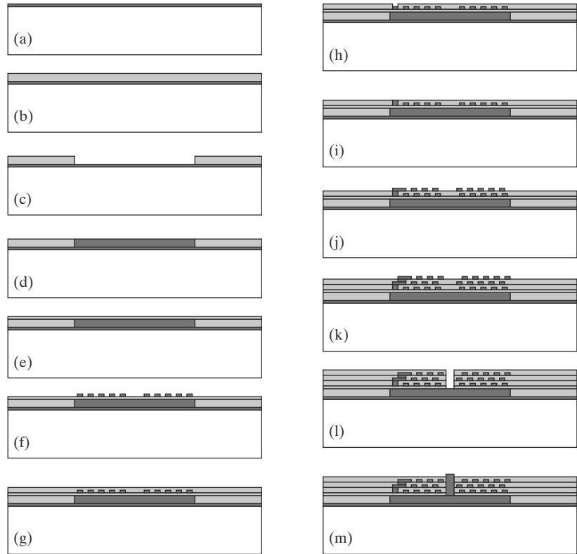
FIGURE 8.10 Process flow for multiple layer planar coil.
