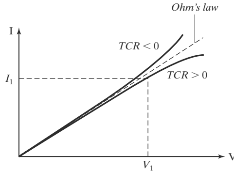
FIGURE 5.11 I-V characteristic of a thermal resistor.
