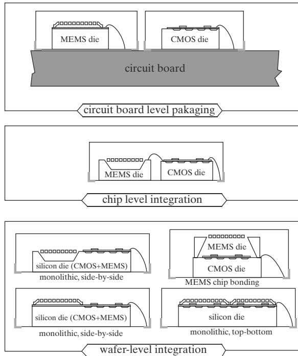
FIGURE 2.24 Options for integrating micromechanical and circuit elements.
