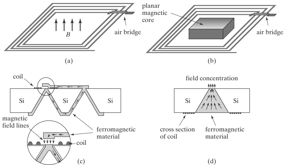
FIGURE 8.9 A planar magnetic inductor.
