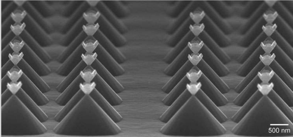
FIGURE 10.25 Photo of pyramids on mesa structures before release. (Courtesy: Prof. Teri Odom, Northwestern University).
