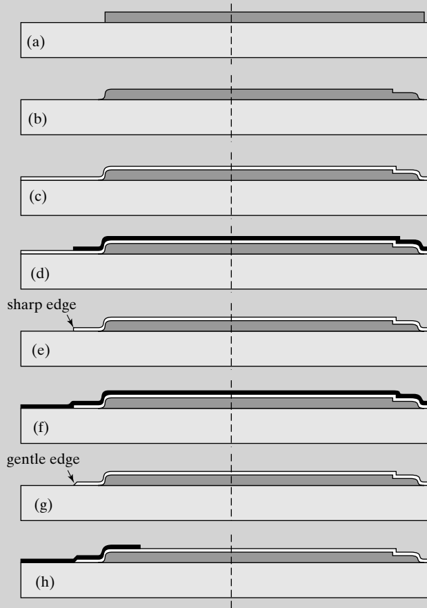
FIGURE 13.6 First eight major steps (a through h) in the Parylene membrane fabrication process.
