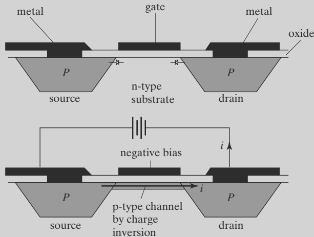
FIGURE 9.8 Operation principle of a regular transistor.
