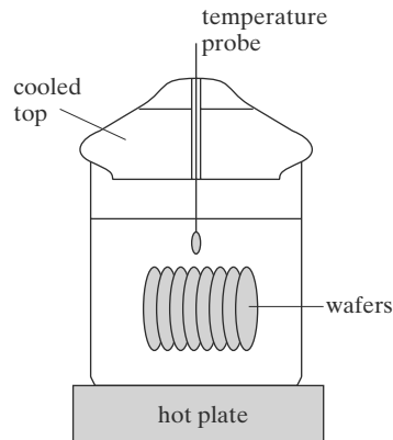
FIGURE 10.19 Wet anisotropic etching reflux system.
