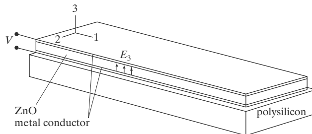
FIGURE 7.3 Bimorph piezoelectric actuator.
