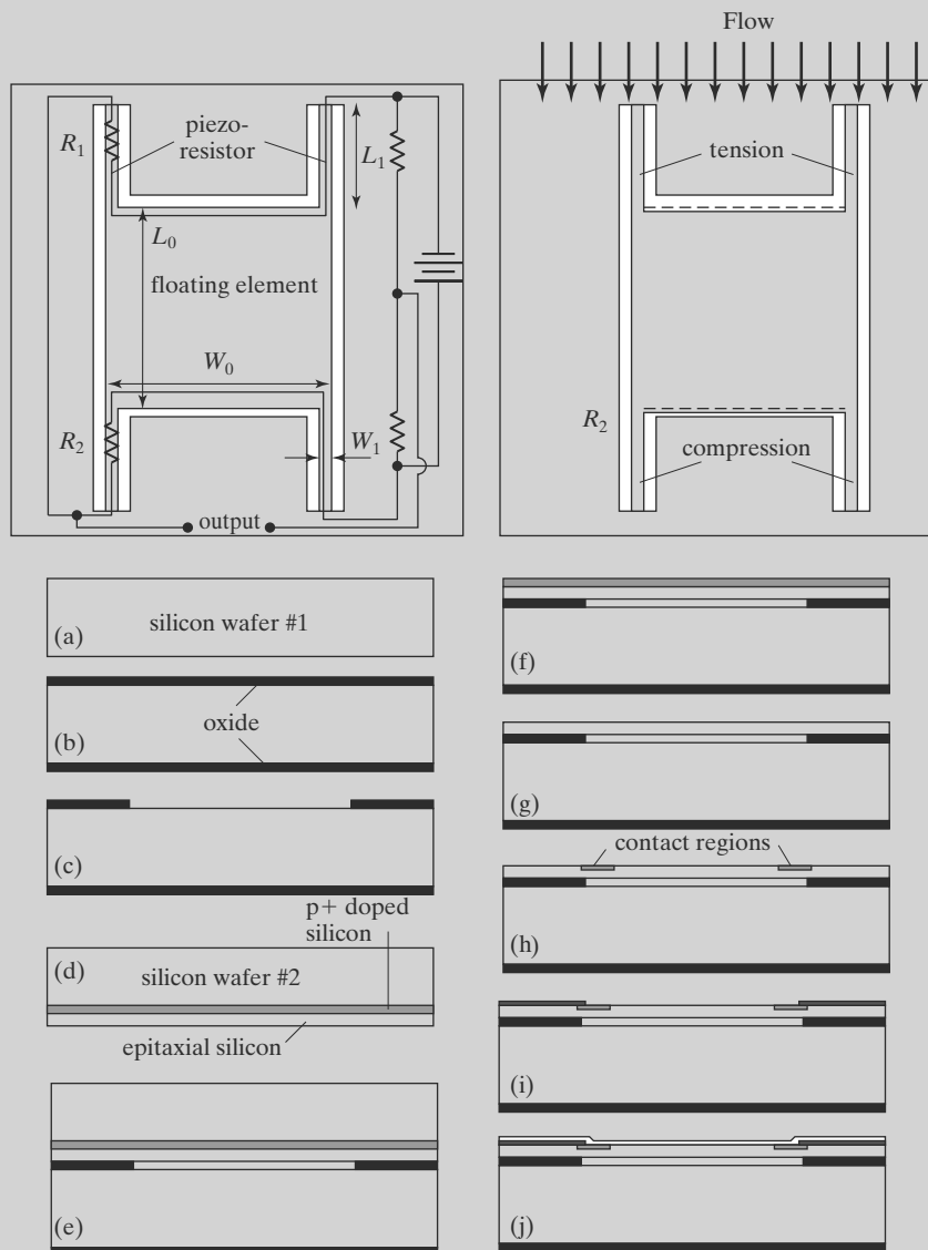
FIGURE 6.17 Piezoresistive shear-stress sensor.
