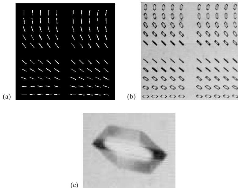
FIGURE 10.23 The etching experiment and simulation for EDP etch rate diagram.
