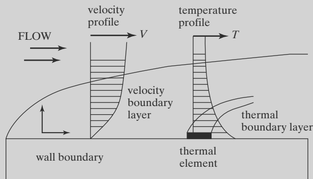
FIGURE 5.17 Velocity and thermal boundary layers.
