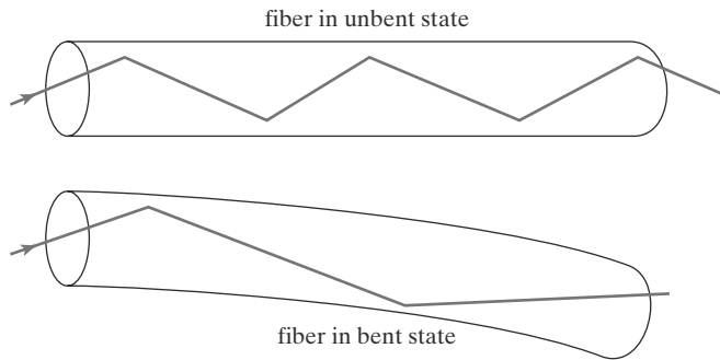
FIGURE 9.3 Optical fiber sensing.
