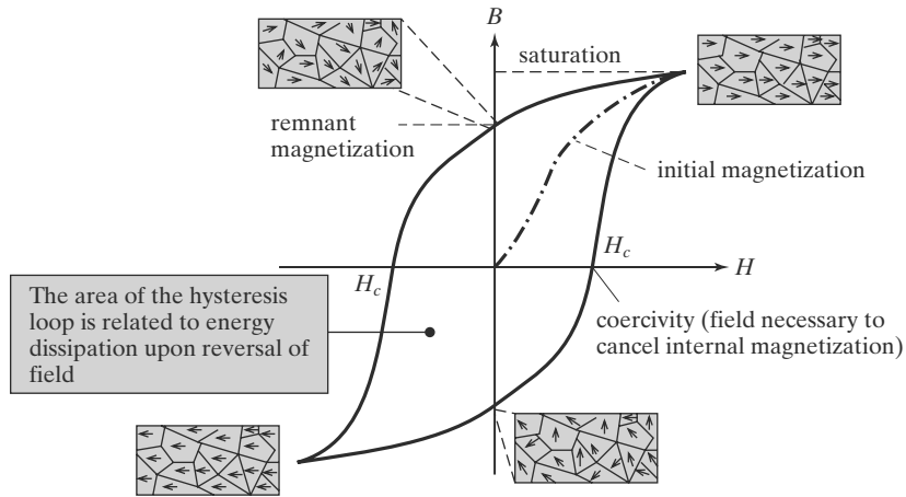
FIGURE 8.1 Magnetization hysteresis curve.
