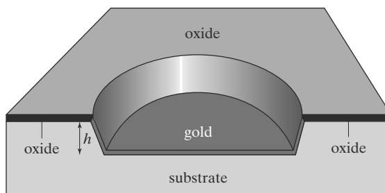
FIGURE 12.27 Diagram of a single pit.
