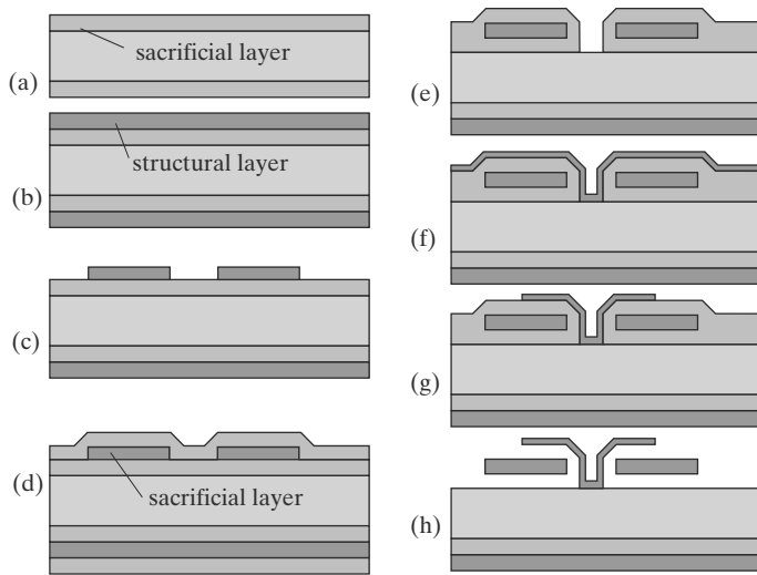
FIGURE 11.1 The fabrication process for a planar electrostatic motor.
