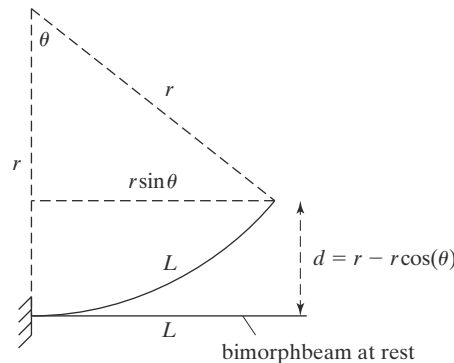
FIGURE 5.4 Geometry of a bent beam.
