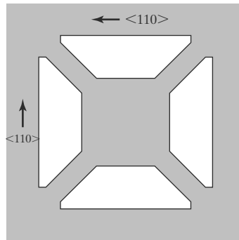
FIGURE 10.28 Etch mask for piezoresistive tactile sensor.
