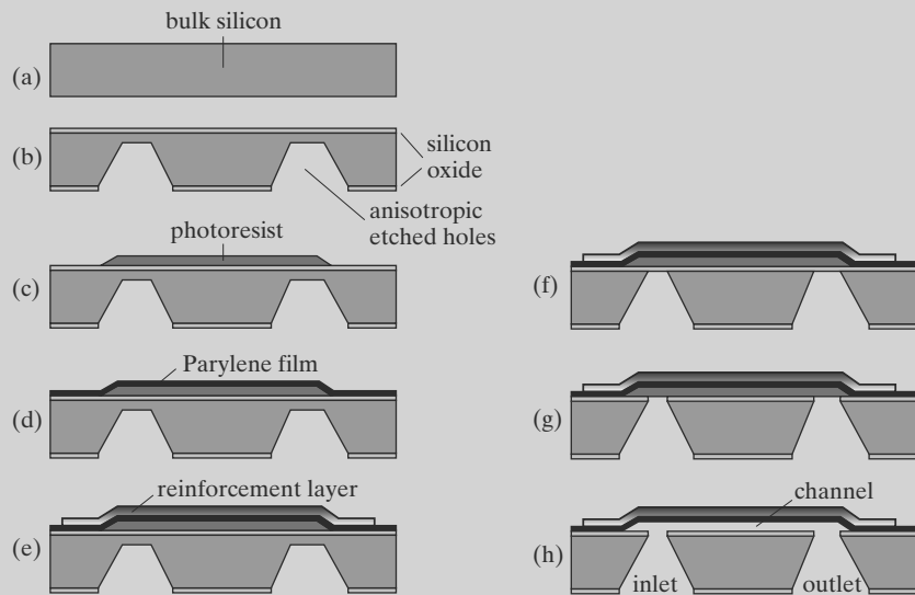
FIGURE 14.14 Fabrication process for a parylene channel.
