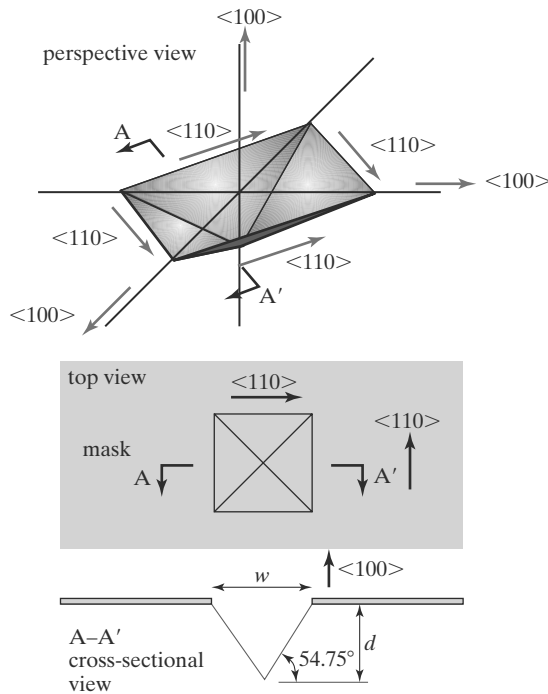
FIGURE 10.6 Cross-sectional profile of an etched cavity.
