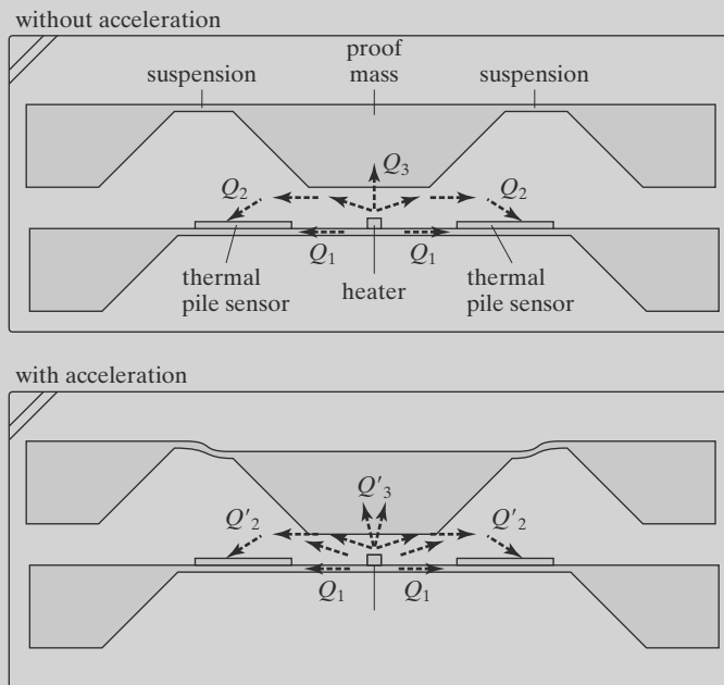
FIGURE 5.12 Principle of thermal accelerometer with moving mass.
