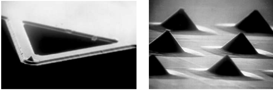
FIGURE 10.3 Cantilever beams formed by anisotropic etching.
