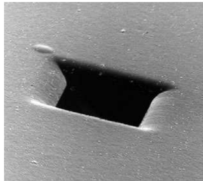
FIGURE 11.8 SEM micrograph of an etch hole.
