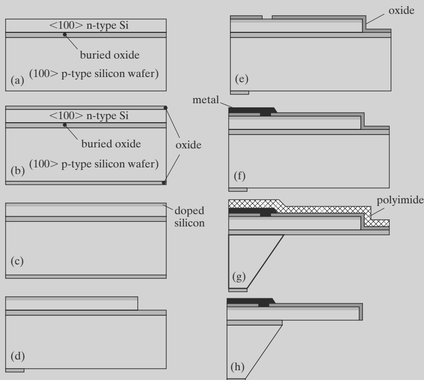
FIGURE 12.20 Fabrication process.
