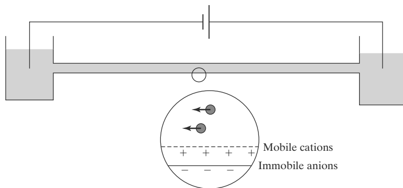
FIGURE 14.3 Electroosmosis (electrokinetic) flow.
