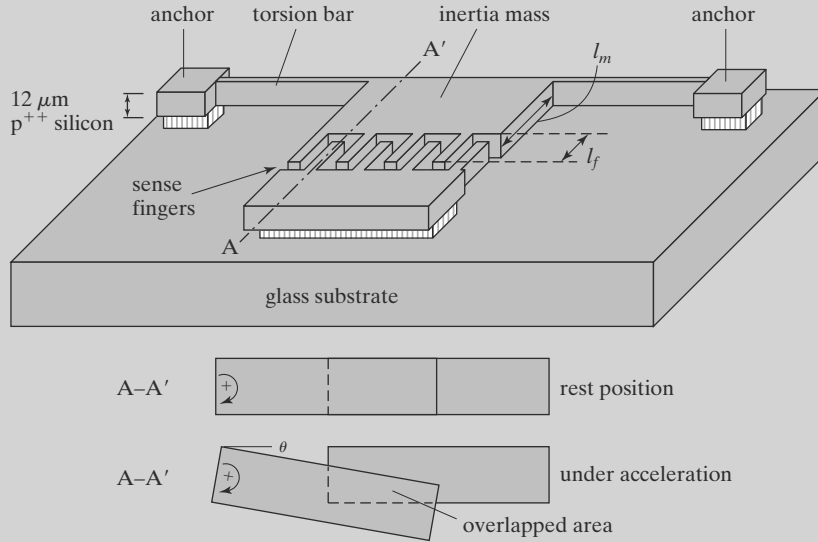
FIGURE 4.21 Torsional acceleration sensor.
