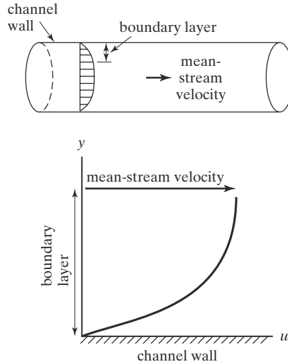
FIGURE 14.2 Velocity profile.
