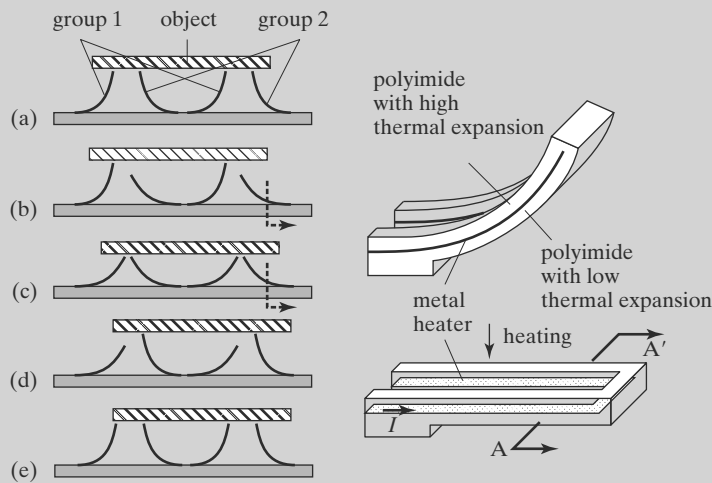
FIGURE 5.5 Artificial cilia array for object transport.
