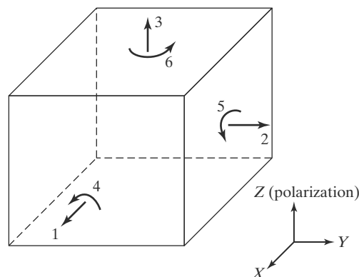
FIGURE 7.1 Schematic illustration of piezoelectric crystal in a rectangular system.
