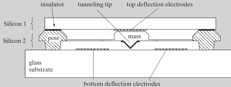
FIGURE 9.2 A tunneling accelerometer.
