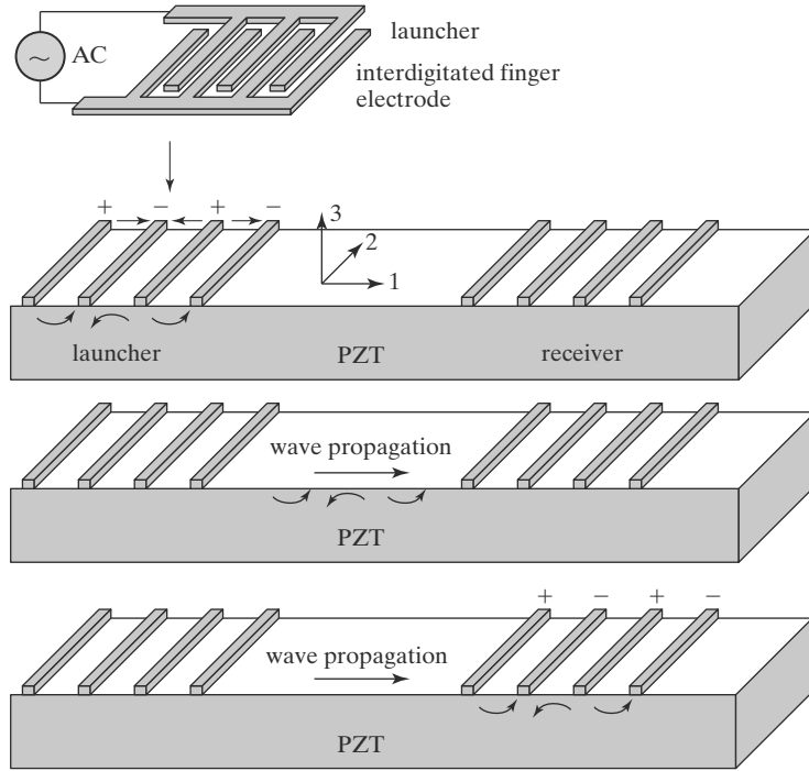
FIGURE 7.13 Launch of SAW wave.
