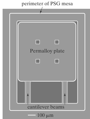
FIGURE 11.7 Surface micromachined magnetic actuator.
