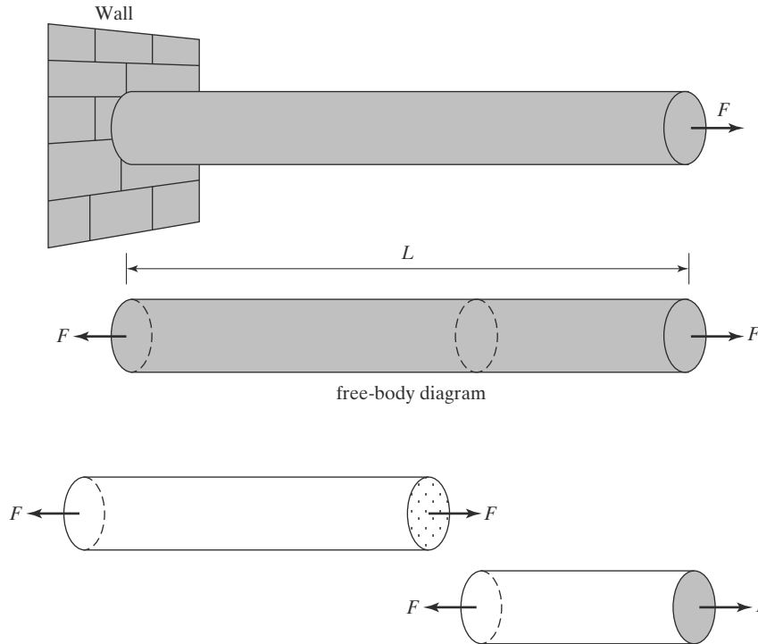
FIGURE 3.8 Force balance analysis
