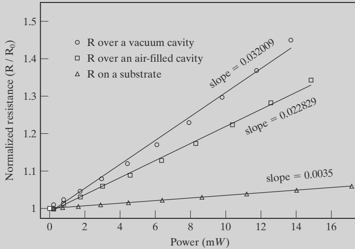
FIGURE 5.26 Resistance vs. power.
