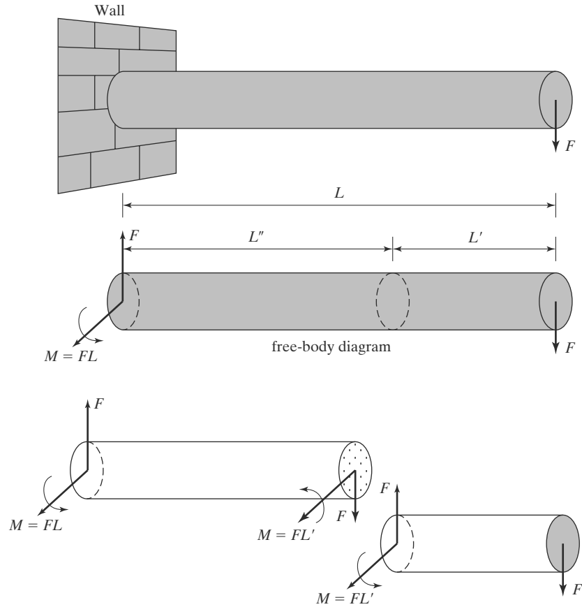
FIGURE 3.9 Force and moment balance analysis.
