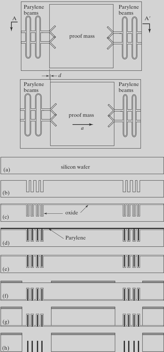
FIGURE 13.4 Parylene accelerometer.
