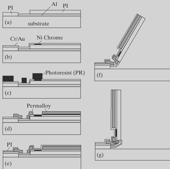
FIGURE 6.19 Schematic of the fabrication process.
