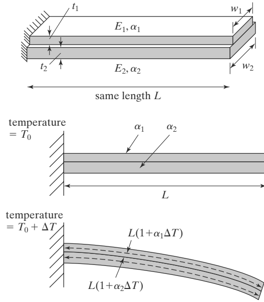
FIGURE 5.3 Thermal bimetallic bending ( \alpha_1 > \alpha_2 ).
