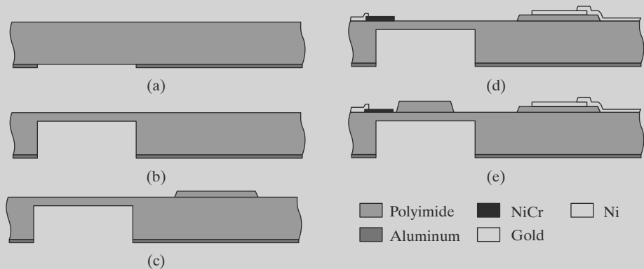
FIGURE 13.13 Schematic diagram of device fabrication.
