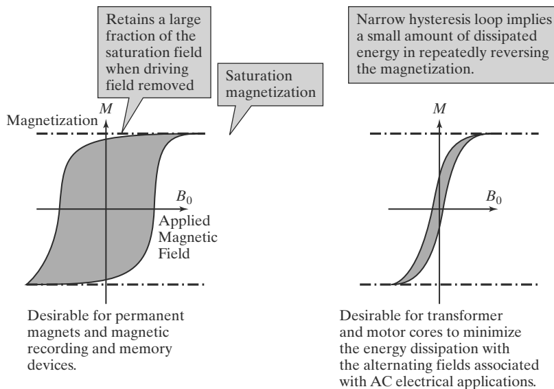
FIGURE 8.2 Representative hysteresis curves for hard and soft magnets.
