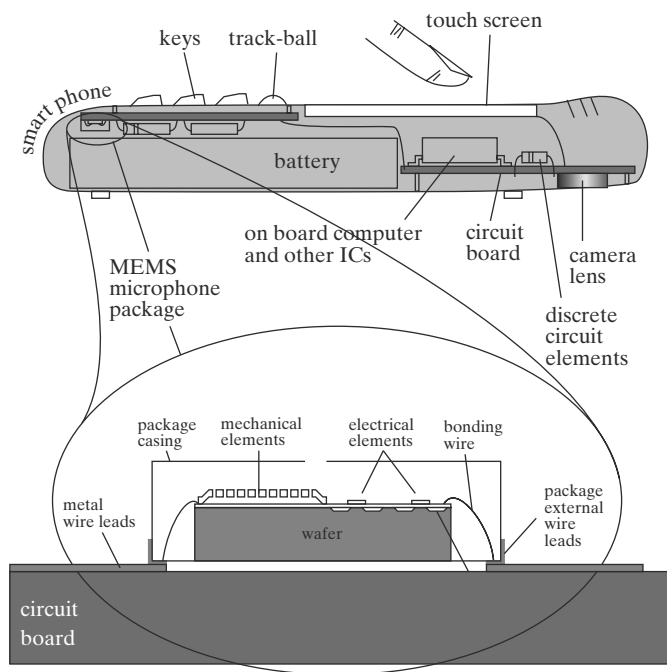
FIGURE 2.4 Diagram showing the interior elements of a smart phone, a packaged sensor chip, and interior components of the chip package.
