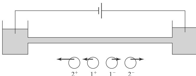
FIGURE 14.5 Capillary electrophoresis.
