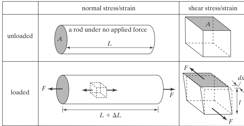
FIGURE 3.10 Normal stress and shear stress.
