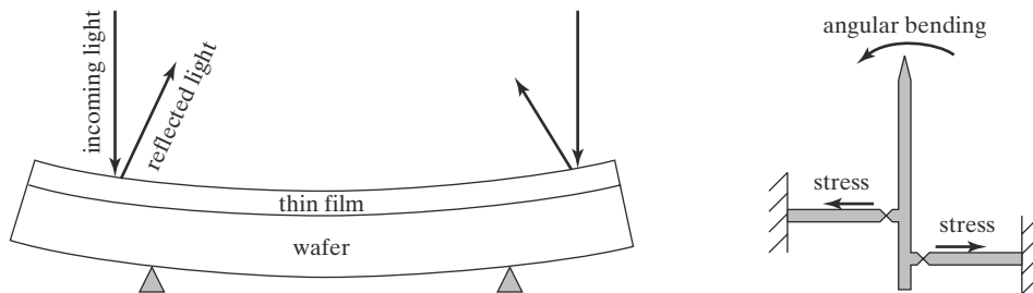
FIGURE 3.28 Experimental methods for measuring intrinsic stress.
