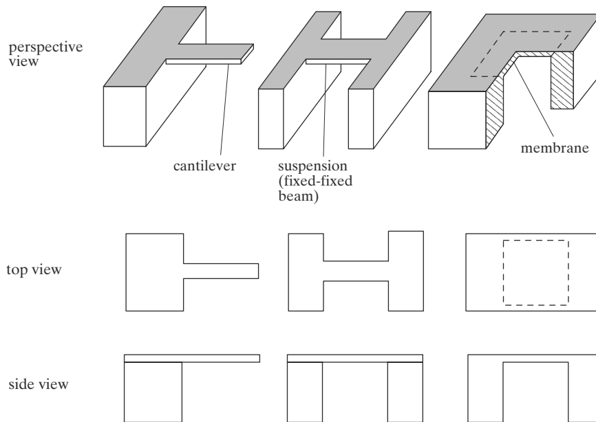
FIGURE 12.1 Cantilever, suspension beam, and membrane.
