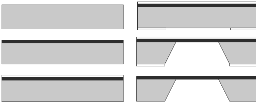
FIGURE 12.9 Method of using heavily doped silicon.
