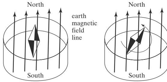
FIGURE 8.4 Magnetostatic actuation of a magnetic compass.
