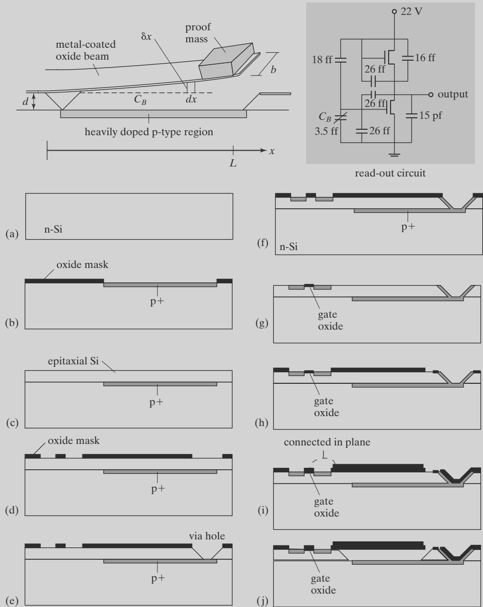
FIGURE 4.8 Capacitive accelerometer.
