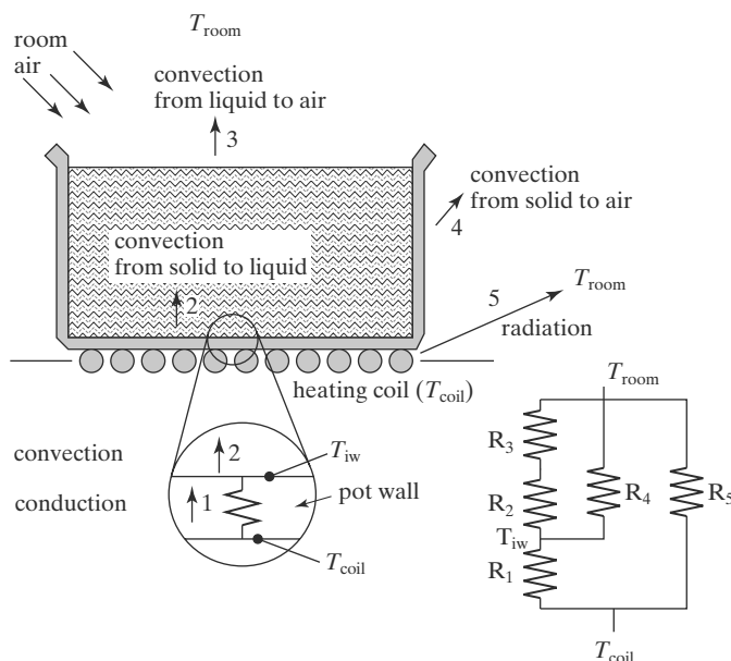
FIGURE 5.2 Heat transfer processes associated with pot heating.
