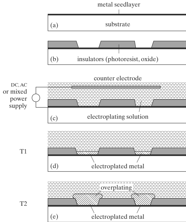
FIGURE 8.6 A process for electroplating of magnetic materials.
