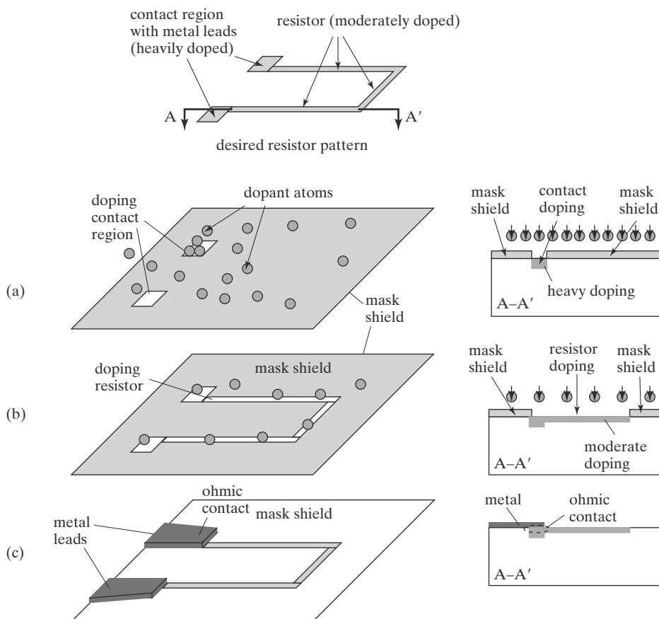
FIGURE 2.16 Two step diffusion doping.
