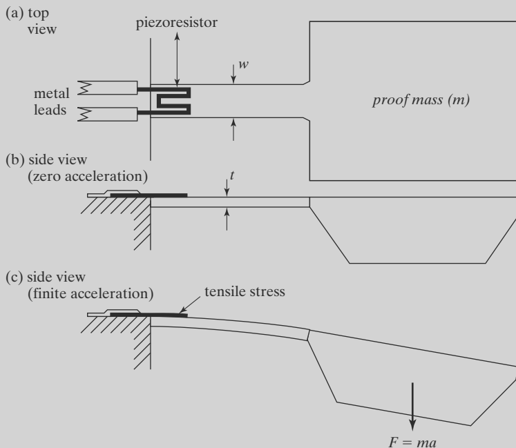
FIGURE 6.10 Piezoresistive accelerometer.
