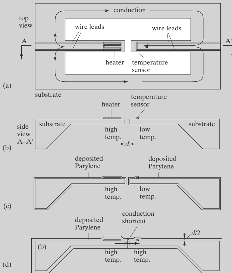
FIGURE 5.31 Schematic diagram of the end-point sensor.
