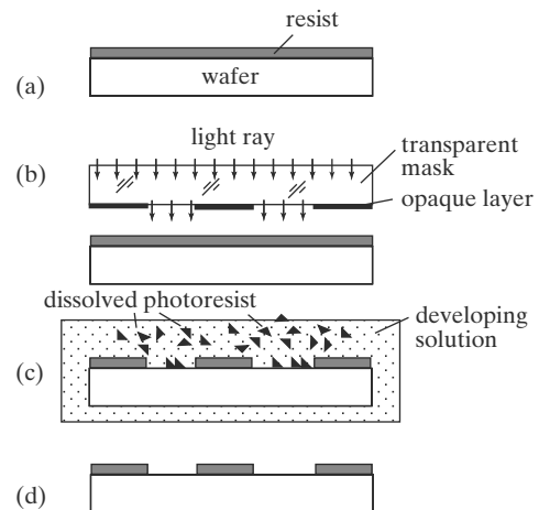
FIGURE 2.7 Process flow for patterning photoresist with a photomask.
