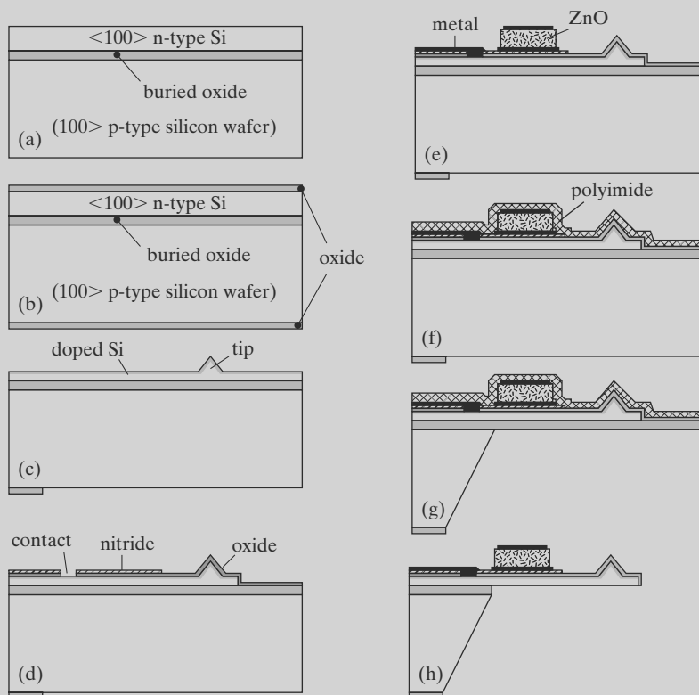
FIGURE 12.23 Fabrication process.
