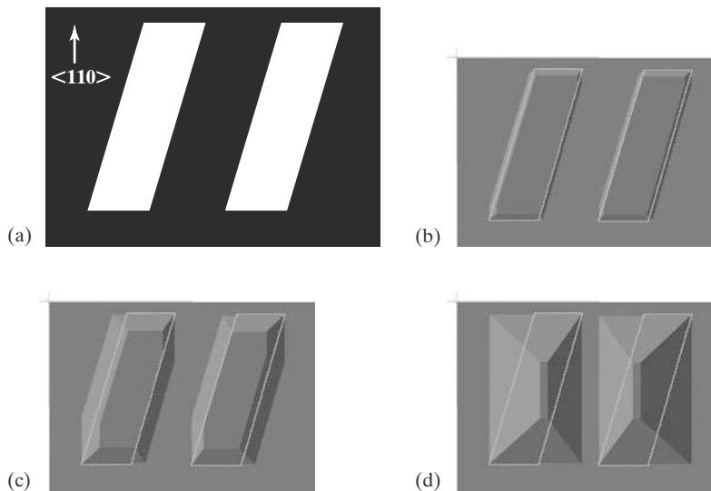
FIGURE 10.17 Progression of etched profile. Frame (a) is the mask. Frames (b) through (d) occur at 10, 60, and 200 minutes into the etching process.
