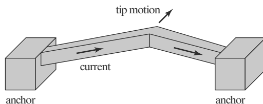
FIGURE 5.8 A bent-beam electrothermal actuator.
