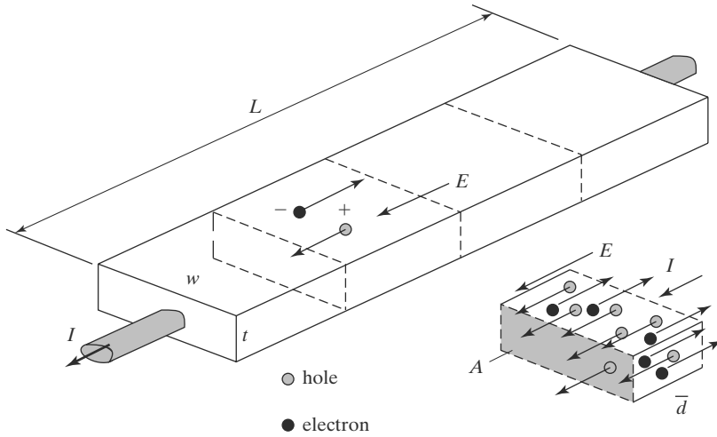
FIGURE 3.1 A semiconductor resistor.
