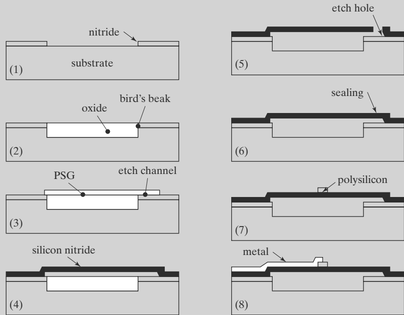
FIGURE 5.19 Fabrication process.
