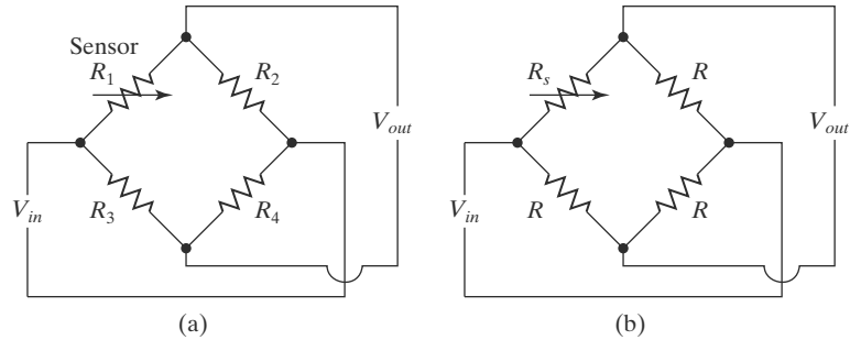
FIGURE 6.3 Wheatstone bridge circuits.
