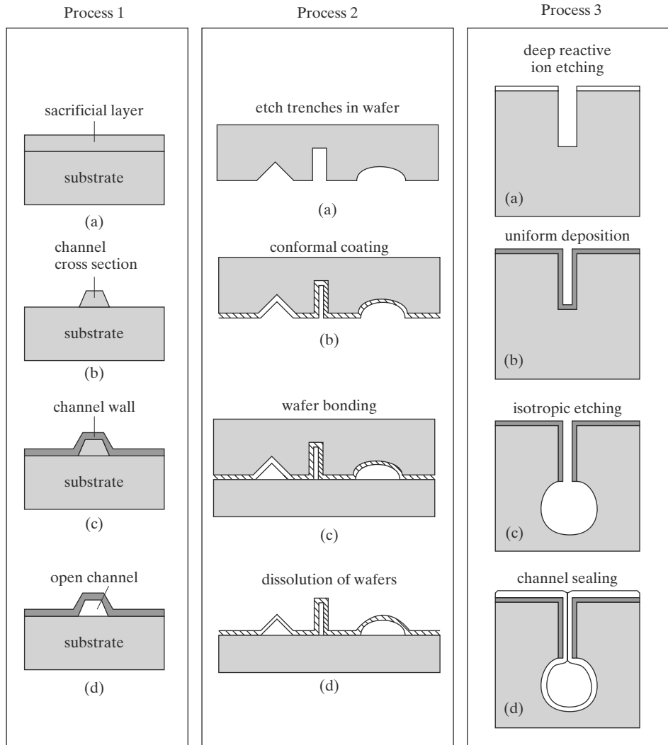
FIGURE 14.6 Representative fabrication processes of channels on silicon substrates.
