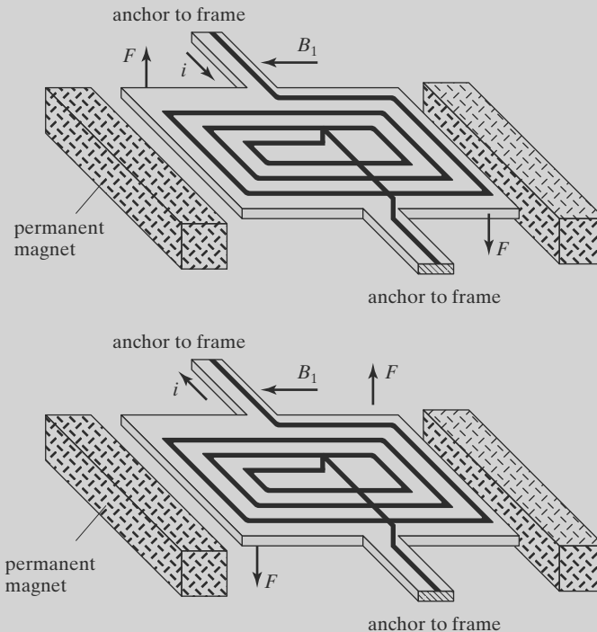
FIGURE 8.16 Diagram of a micro mirror.
