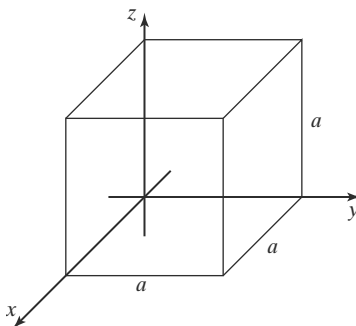
FIGURE 3.4 Cubic lattice.
