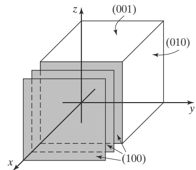
FIGURE 3.6 Equivalent planes.
