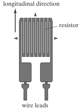
FIGURE 6.4 Serpentine-type coil strain sensors.
