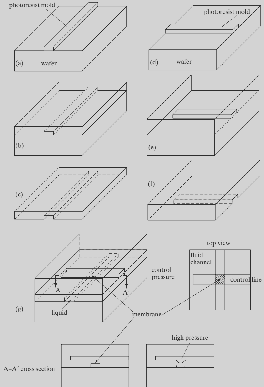
FIGURE 14.15 Pneumatic controlled PDMS valve.
