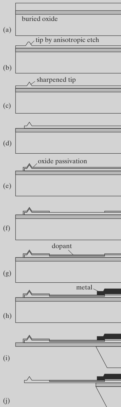
FIGURE 12.21 Fabrication of 1\ \mu\text{m} thick beams.
