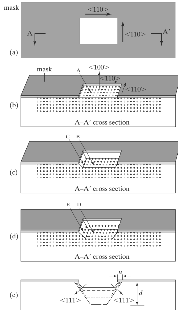
FIGURE 10.4 Etch profile evolution.
