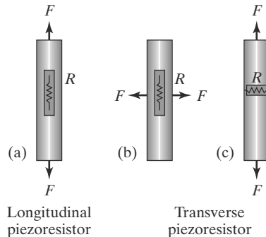
FIGURE 6.2 Longitudinal (a) and transverse gauge (b and c) factors.
