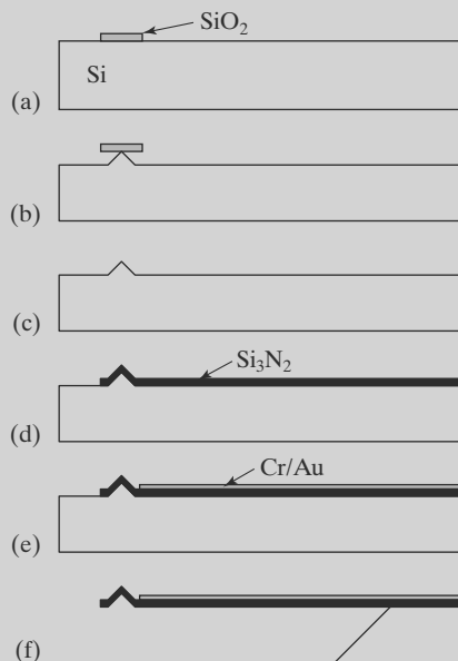
FIGURE 12.25 Microfabrication process for TA-DPN probes.
