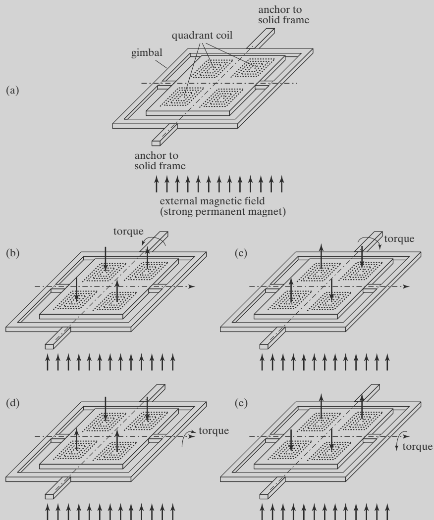
FIGURE 8.17 Optical micromirror capable of two-axes rotation.
