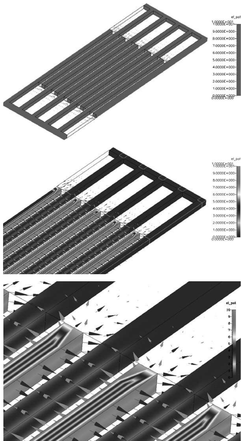
FIGURE 4.17 Distribution of electric field lines between two sets of fingers, with three levels of magnifications. The simulation is performed using software from CFDRC Corp.
