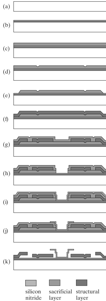
FIGURE 11.2 Micro motor fabrication.
