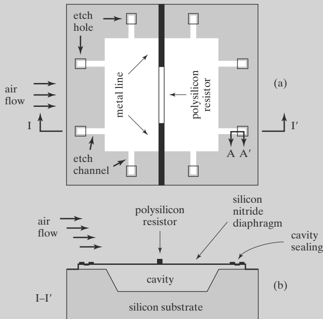
FIGURE 5.18 Schematic diagram of the thermal shear-stress sensor.
