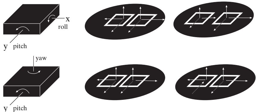
FIGURE 15.15 Candidate sensing- detection options for two axis gyros.
