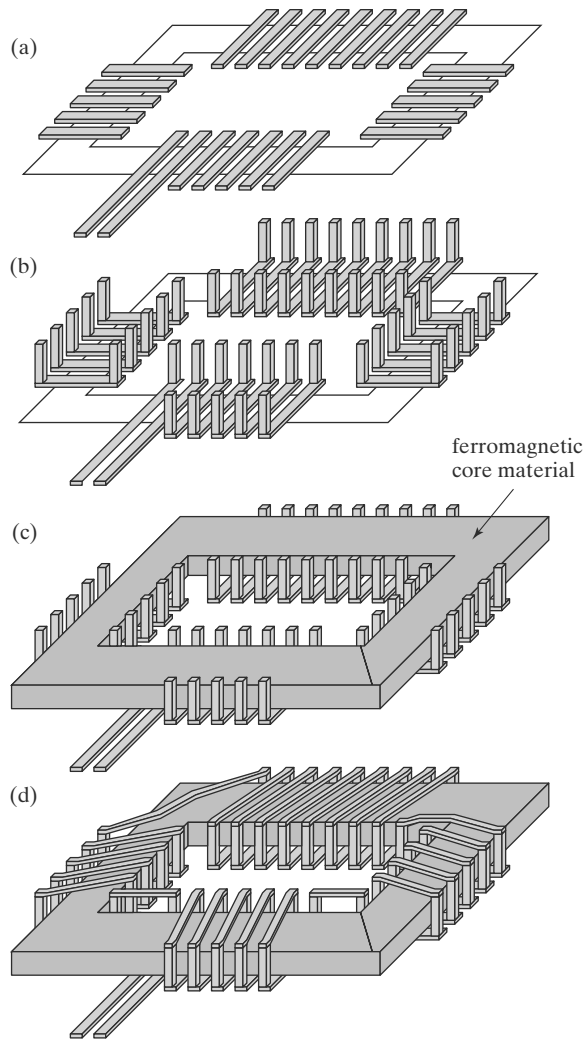
FIGURE 8.11 Fabrication of three-dimensional micro coil.
