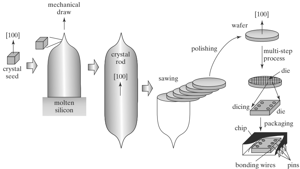
FIGURE 2.1 Wafer process steps.
