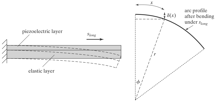
FIGURE 7.2 Bending of a piezoelectric bimorph.
