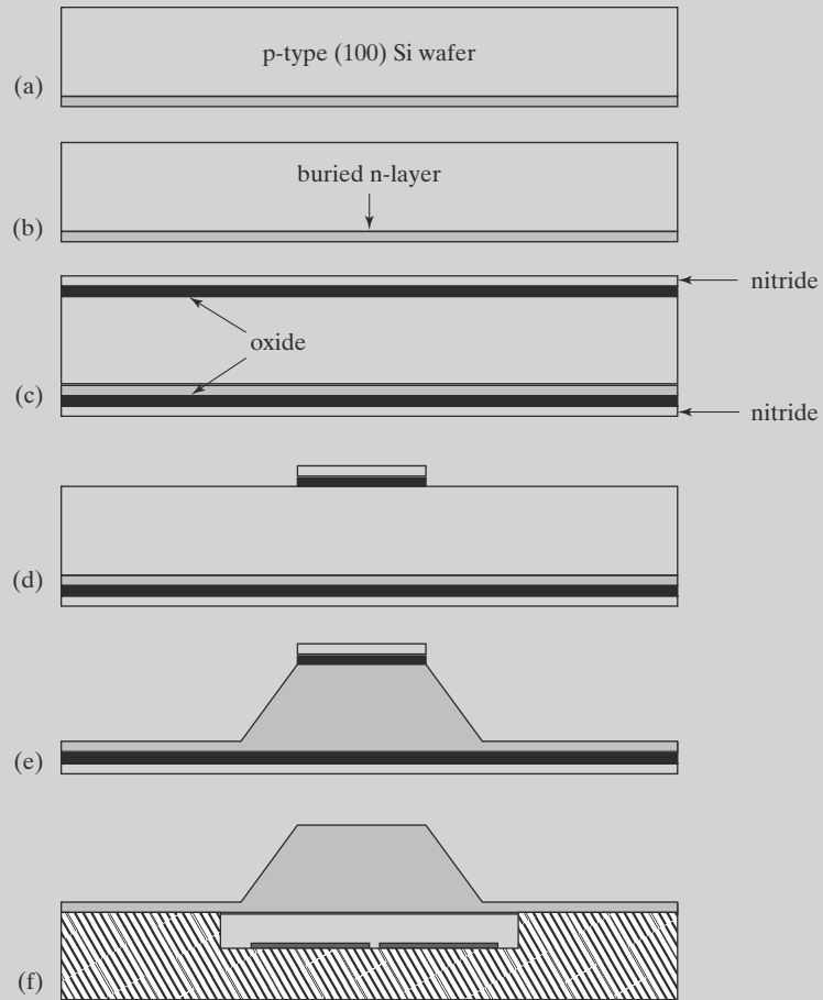
FIGURE 4.14 Fabrication process of tactile sensor.
