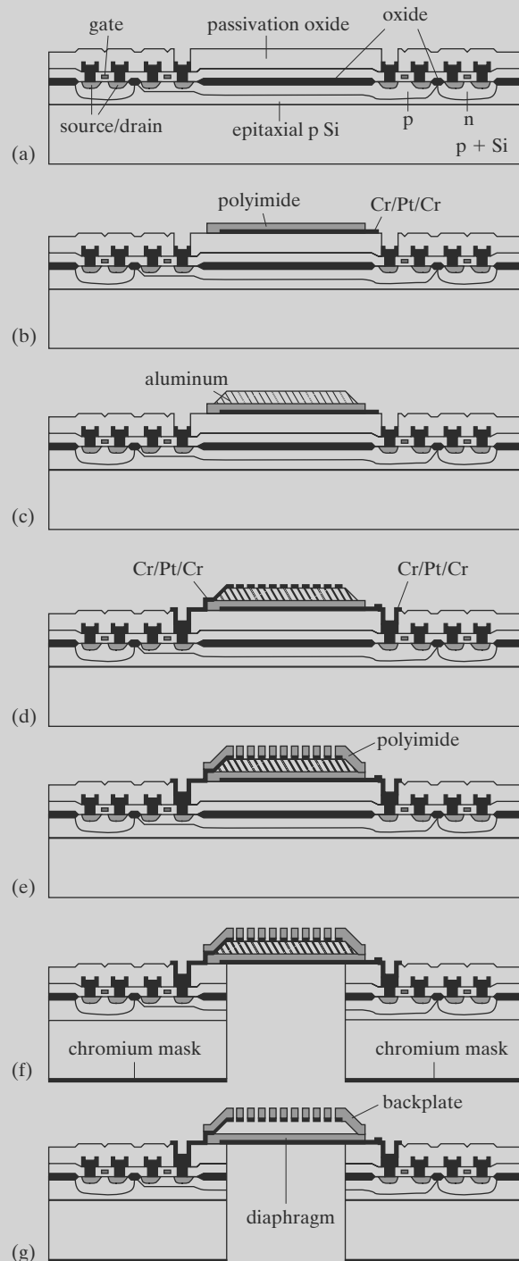
FIGURE 4.11 Fabrication process of condenser microphone.
