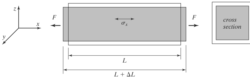
FIGURE 3.11 Longitudinal elongation of a bar under an applied normal stress.
