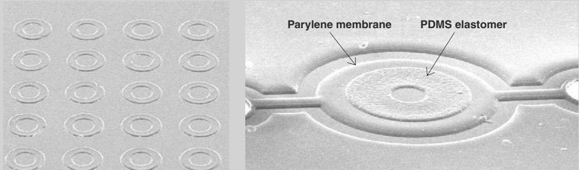
FIGURE 13.3 Micromachined PDMS O-rings.
