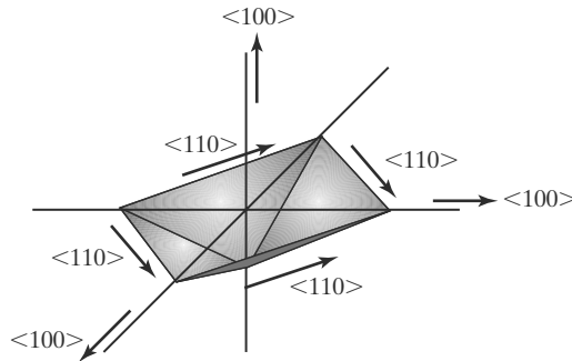
FIGURE 10.9 Perspective view of a suspended beam over an anisotropic etched cavity.
