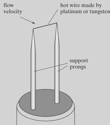
FIGURE 5.14 Schematic diagram of a conventional hot-wire anemometer.
