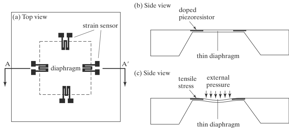
FIGURE 15.3 Pressure sensor.
