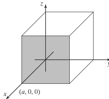
FIGURE 3.5 (100) plane.
