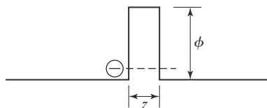
FIGURE 9.1 Electron tunneling phenomenon.
