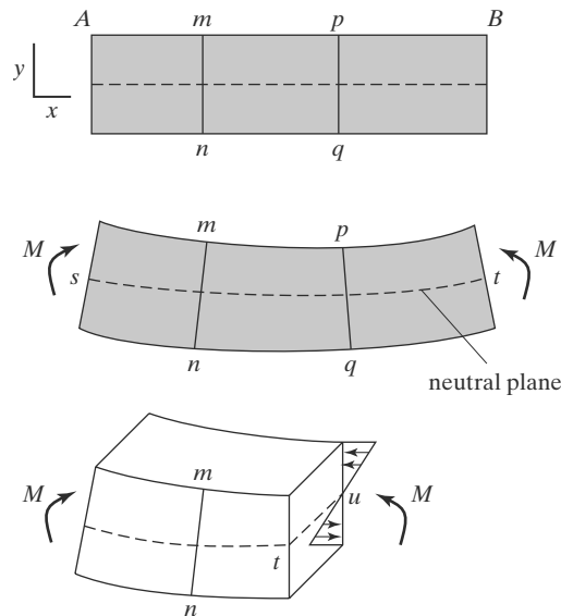
FIGURE 3.16 Bending of a segment of a beam under pure bending.
