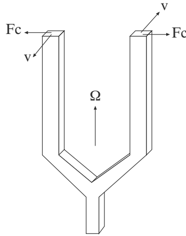
FIGURE 15.11 A tuning fork gyro.
