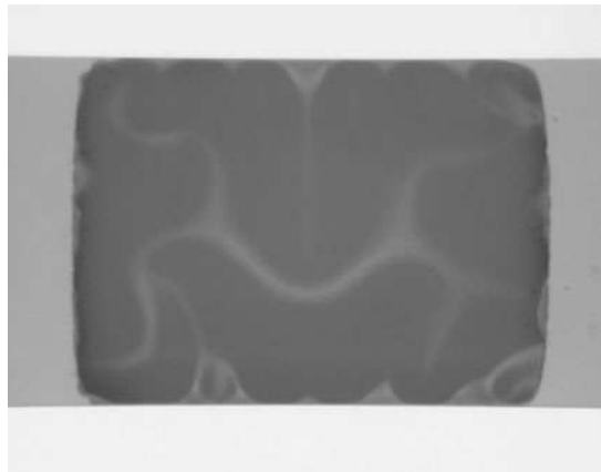
FIGURE 3.25 Cross section of a taunt membrane under tensile stress and a warped membrane under compressive stress. An optical micrograph of a warped membrane is shown.
