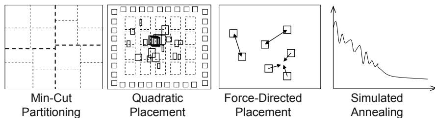
Fig. 4.6 Common techniques for global placement.
