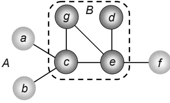
Fig. 2.3 A 2-way partitioning of the circuit in Fig. 2.2. A contains nodes a, b and f . B contains nodes c, d, e and g . Edges (a, c) , (b, c) and (e, f) are cut. Edges (c, e) , (c, g) , (d, e) and (e, g) are not cut.
