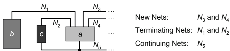
Fig. 3.13 Classification of nets based on the partially-constructed linear ordering.
