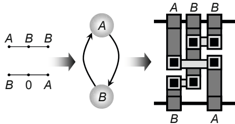
Fig. 6.9 A channel routing problem (left), its VCG with a cycle or conflict (center), and a possible solution using net splitting and an additional third track (right).
