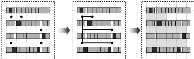
Fig. 5.16 Assignment of each segment of the Steiner tree generated for the net from Fig. 5.15 (left and center). The routing regions affected are shaded in light gray (right).
