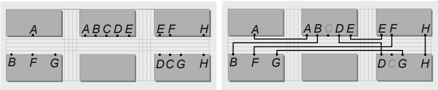
Fig. 5.10 A gate-array design with channel height = 4 (left). If all nets are routed with their shortest paths, the full netlist is unroutable. In one possible routing, net C remains unrouted (right).
