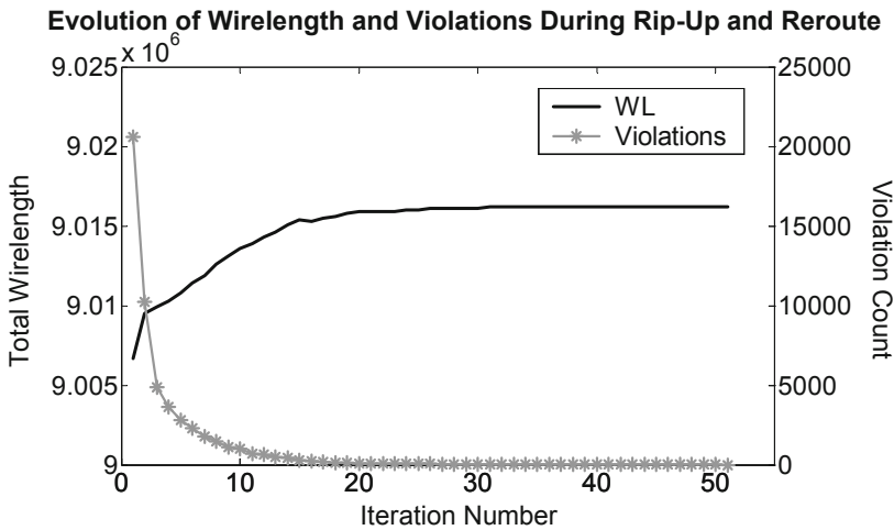
Fig. 5.23 Progression of wirelength and violation count during the rip-up and reroute stage.
