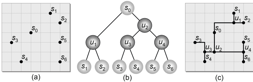
Fig. 7.8 (a) A clock tree routing instance. (b) Connection topology. (c) Embedding.
