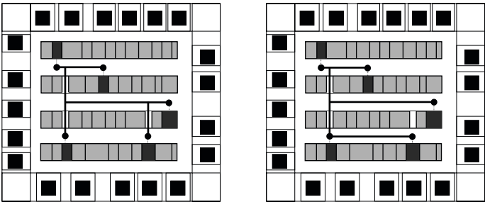
Fig. 5.9 Two different rectilinear Steiner tree solutions for routing of a five-pin net. The solution on the left has the least wirelength, while the solution on the right uses the fewest vertical segments.
