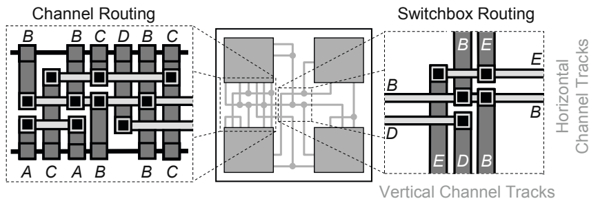
Fig. 6.1 Example of two-layer channel and switchbox routing. The pins of each net A-D are all positioned perpendicular to the channel. Each layer has a preferred direction – one layer has only horizontal tracks and one layer has only vertical tracks. Vias are used if routing a net requires both horizontal and vertical tracks.
