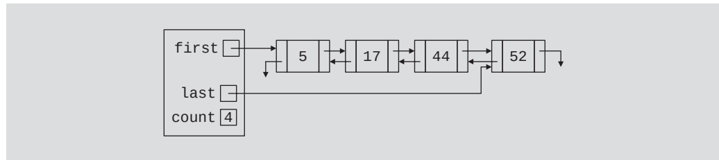
FIGURE 5-30 Doubly linked list before deleting 17
