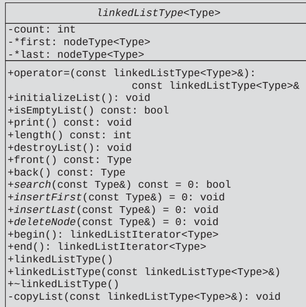
FIGURE 5-19 UML class diagram of the class linkedListType
