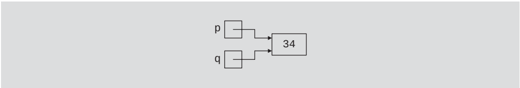
FIGURE 3-8 Pointers p and q and the memory space to which they point after the execution of the statement in Line 10
