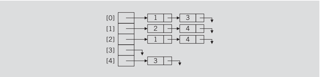
FIGURE 12-5 Adjacency list of graph G_2 of Figure 12-4
