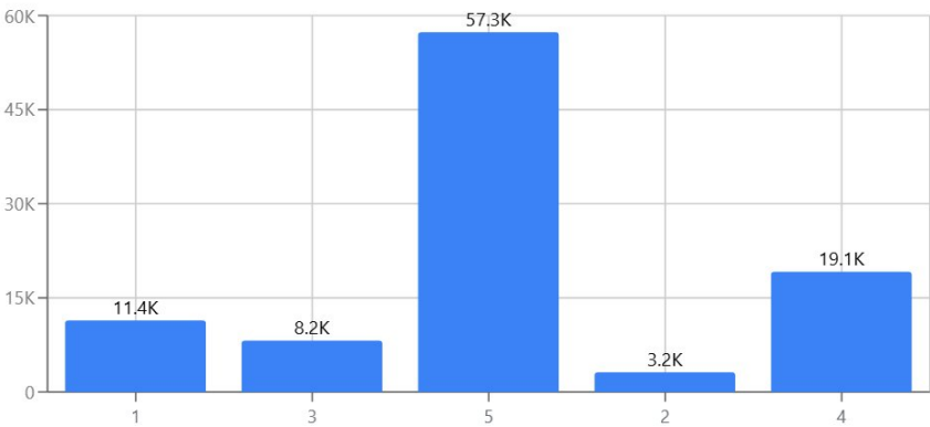
Review score
