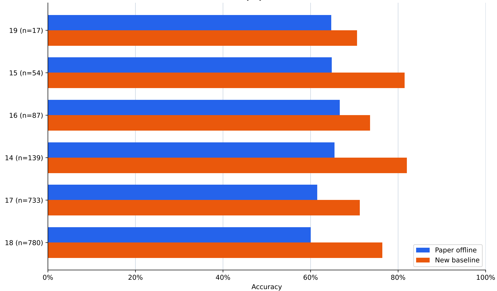
Accuracy by 3GPP release
