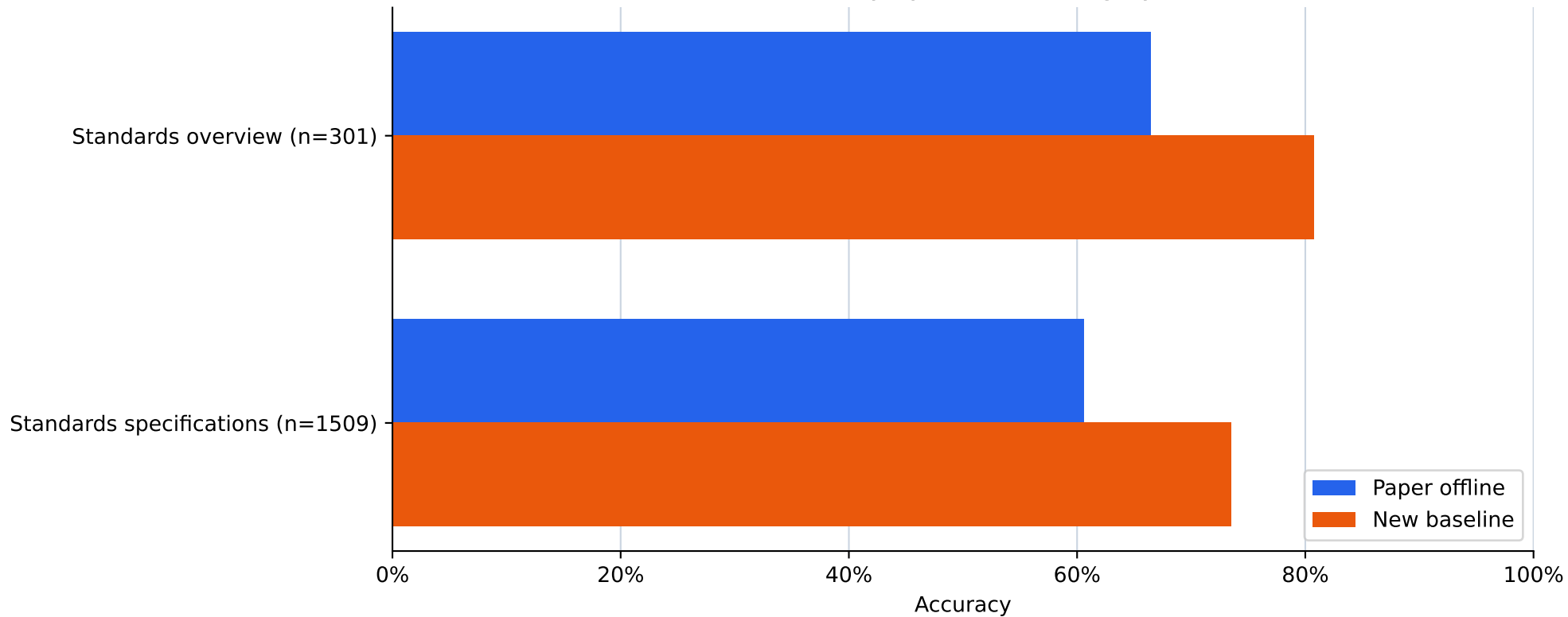
Accuracy by TeleQnA category
