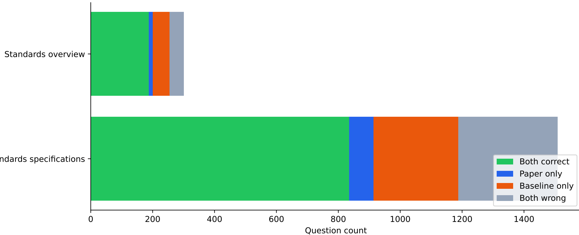
Where each run succeeds or fails, by category
