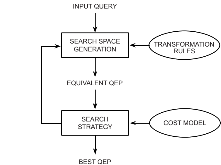
Fig. 8.1 Query Optimization Process
