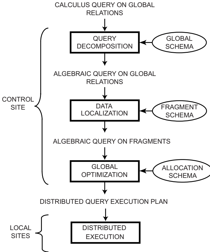
Fig. 6.3 Generic Layering Scheme for Distributed Query Processing
