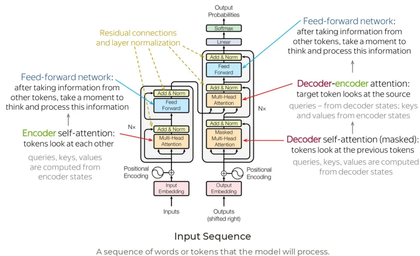
FIGURE 1 – Architecture Transformer et limites attentionnelles
