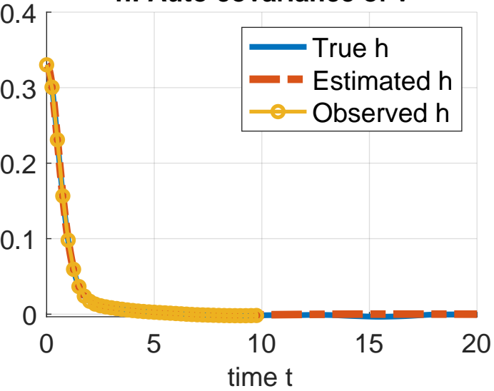
h: Auto covariance of v
