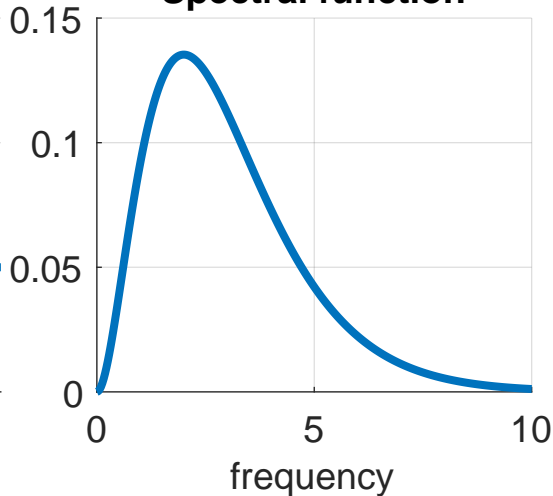
Spectral function
