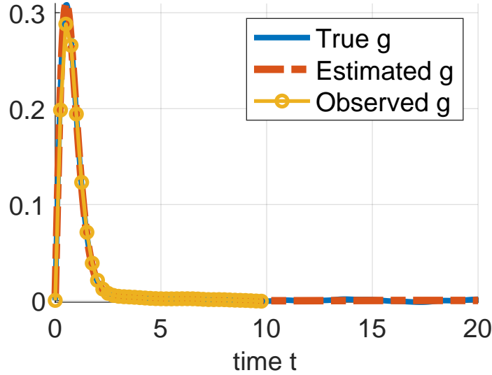
g: g = -h'
