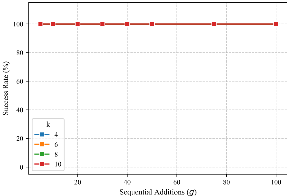
Test 2: Success Rate vs. Sequential Additions
