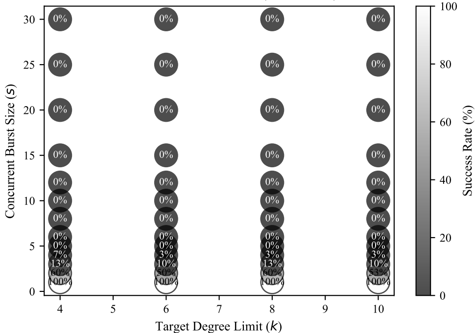
Test 3: Bubble Chart of k vs S (Size = Trials)
