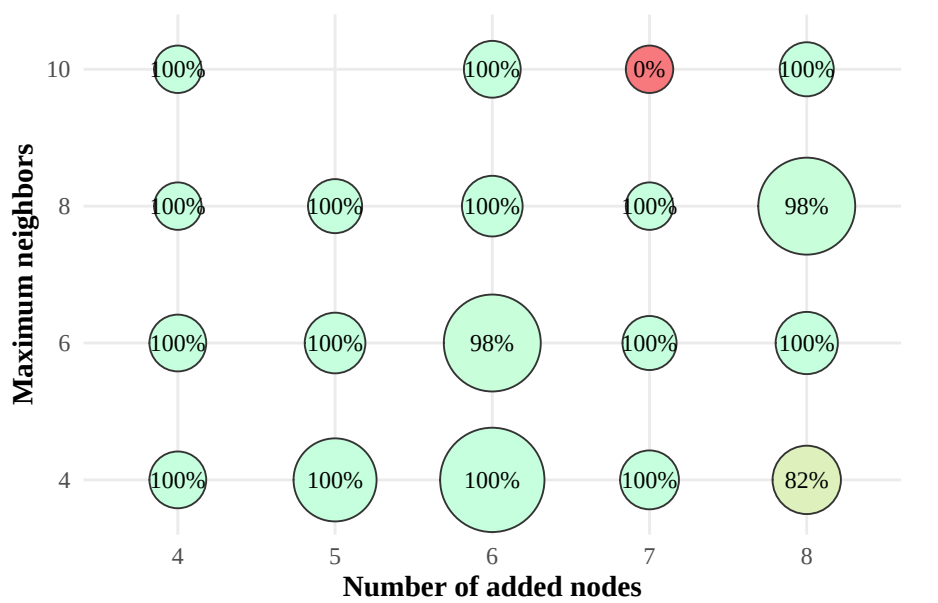
Phase 4: Final Success Rate by Added Nodes and Neighbor Limit
