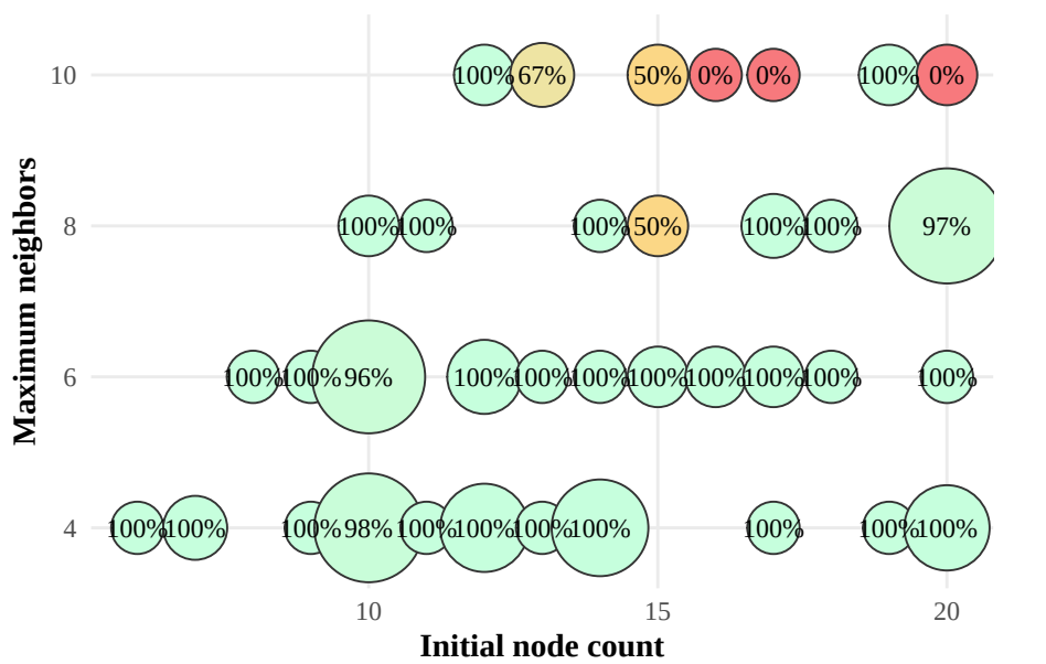
Phase 3: Final Success Rate by Network Size and Neighbor Limit
