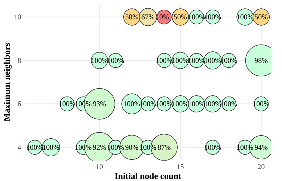
Phase 1: Final Success Rate by Network Size and Neighbor Limit
