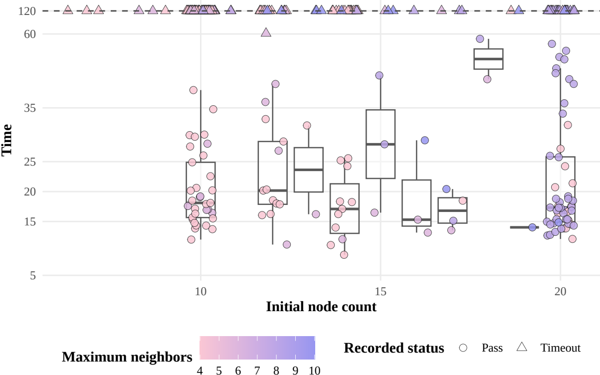
Phase 1: Execution Time by Initial Node Count and Neighbor Limit
