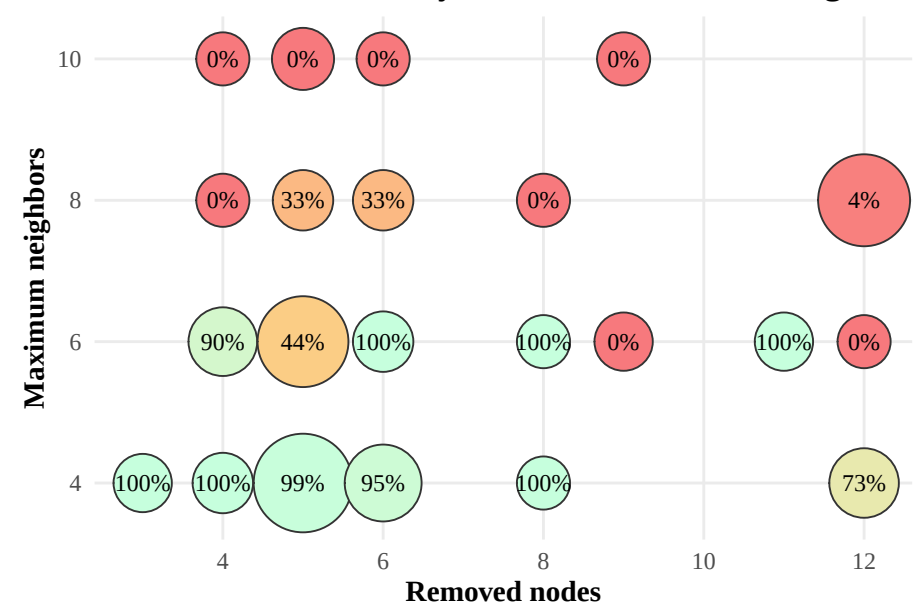
Phase 5: Final Success Rate by Removed Nodes and Neighbor Limit
