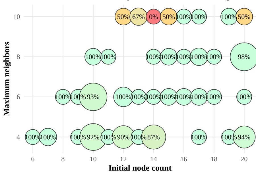
Phase 1: Final Success Rate by Network Size and Neighbor Limit
