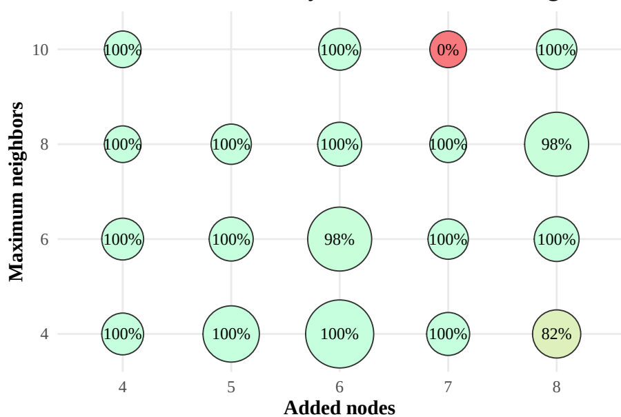
Phase 4: Final Success Rate by Added Nodes and Neighbor Limit
