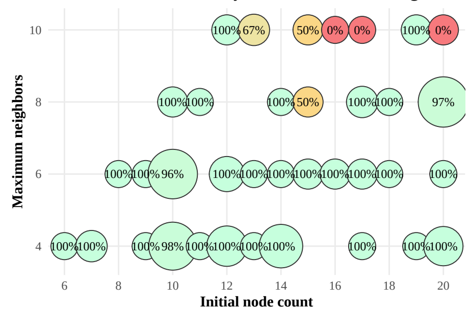
Phase 3: Final Success Rate by Network Size and Neighbor Limit
