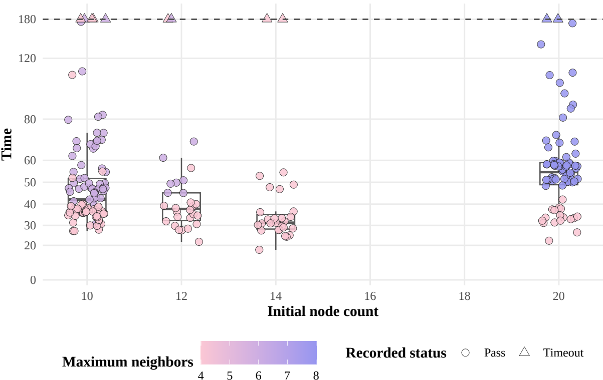
Phase 3: Execution Time by Initial Node Count and Neighbor Limit
