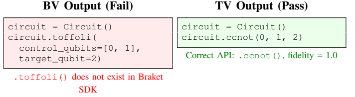
Fig. 5. Haiku on the Toffoli circuit: BV uses a nonexistent API, while TV’s analysis leads to the correct call—an example of CoT helping near the capability boundary.
