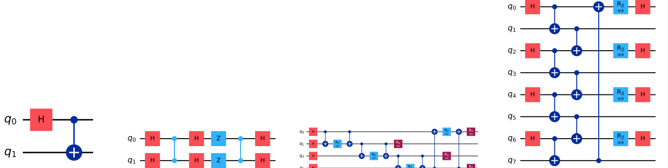
Fig. 2. Representative circuits spanning the difficulty spectrum. Notably, the 8-qubit consensus circuit (d) passes with perfect fidelity due to its regular repeating structure, while the 4-qubit QAOA (c) fails for multiple models due to parallel gate layers—demonstrating that structural regularity, not qubit count, determines AI comprehension success.
