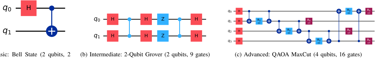
Fig. 2. Representative circuit diagrams from each difficulty level, generated using Qiskit’s matplotlib drawer. Complexity increases from left to right in qubit count, gate count, and structural depth.
