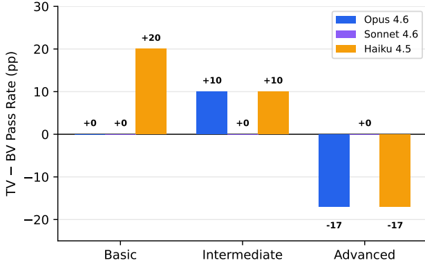
Fig. 3. TV–BV pass rate difference by model and difficulty. Opus and Haiku show a reversal from positive to negative; Sonnet is entirely unaffected.
