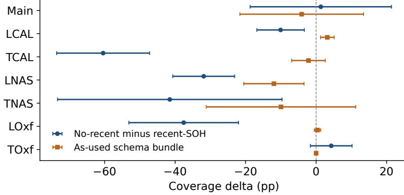
Figure 2: Per-task recent-label and as-used schema-bundle coverage deltas (percentage points) with Bonferroni-corrected normal intervals. Recent-label deltas are large and negative in several tasks; bundle deltas are smaller, with LCAL and LNAS meeting the coverage flag. The endpoint-wide negative-control gate fails in LCAL and TCAL. The dashed line marks zero.
