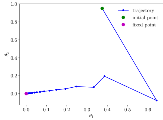
(b) Damped iteration ( \alpha = 0.7 )
