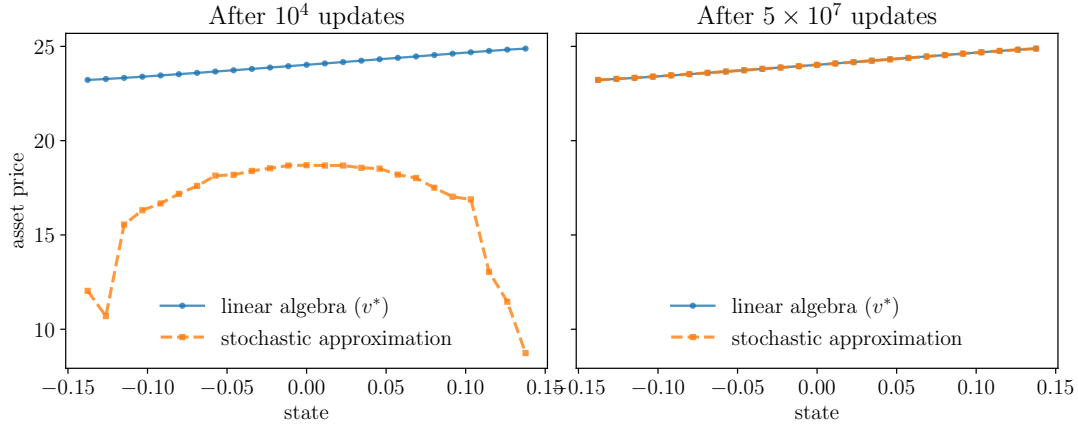
Figure 9.5: Sequential stochastic approximation vs. linear algebra for asset pricing: partial convergence (left) and near-full convergence (right)
