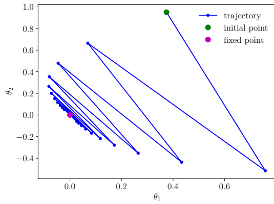
(a) Standard iteration
