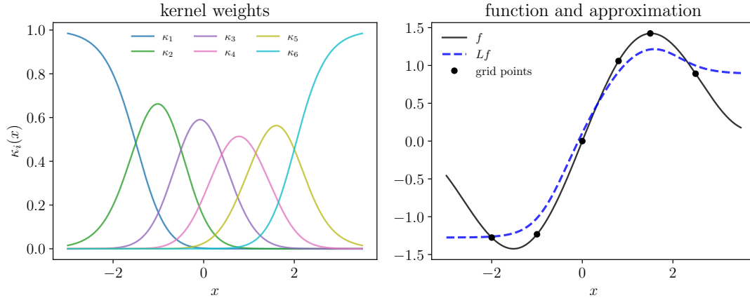
Figure 9.1: Gaussian kernel averager: kernel weights (left) and function approximation (right)
