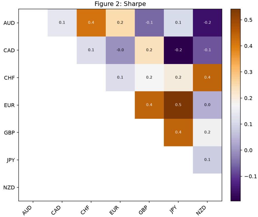
Figure 2: Heatmap of annualized Sharpe ratios by unordered pair ( z^* = 1 , EG-filtered).
