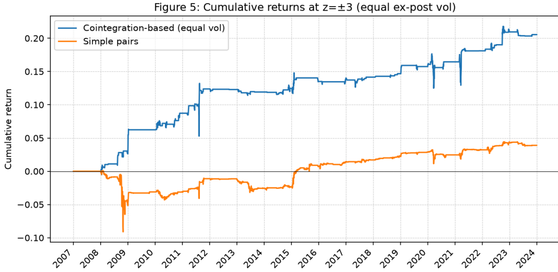
Figure 5: Cumulative returns at z^* = \pm 3 (equal ex-post vol; visuals only).
