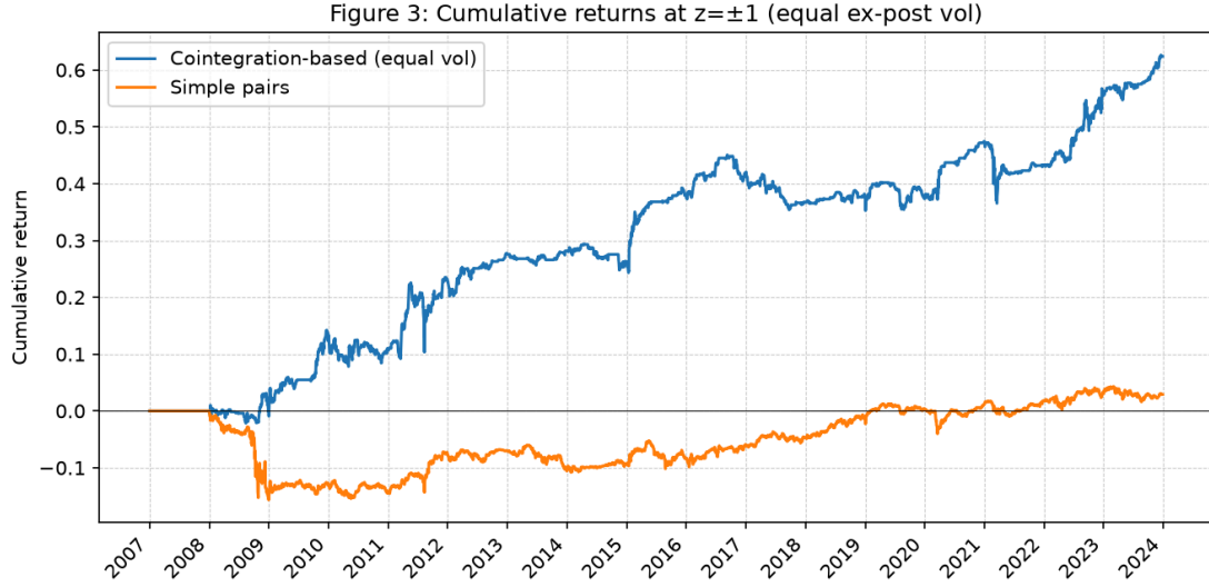
Figure 3: Cumulative returns at z^* = \pm 1 (equal ex-post vol; visuals only).
