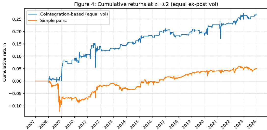
Figure 4: Cumulative returns at z^* = \pm 2 (equal ex-post vol; visuals only).
