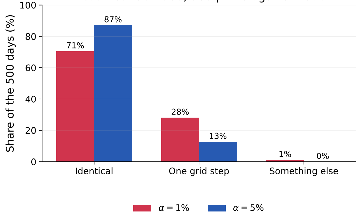
Measured: S&amp;P 500, 500 paths against 2000
