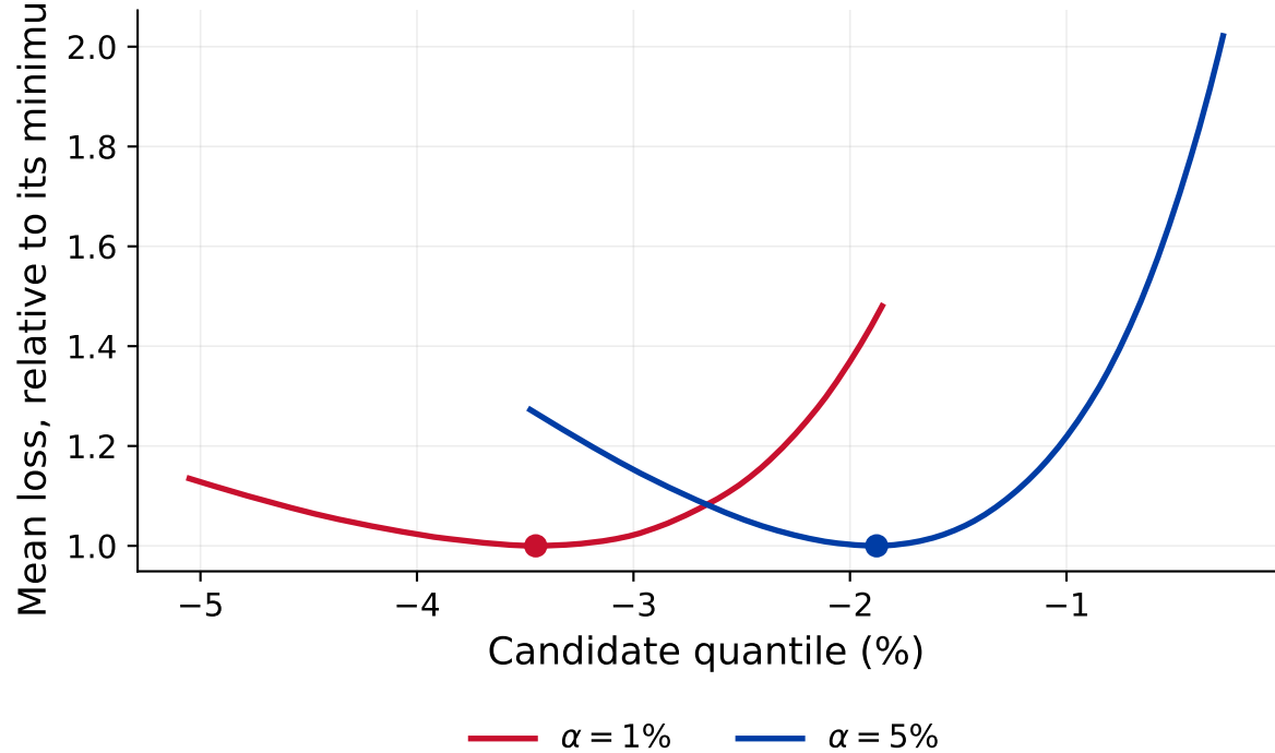
Minimised at the truth, and flat around it at 1%
