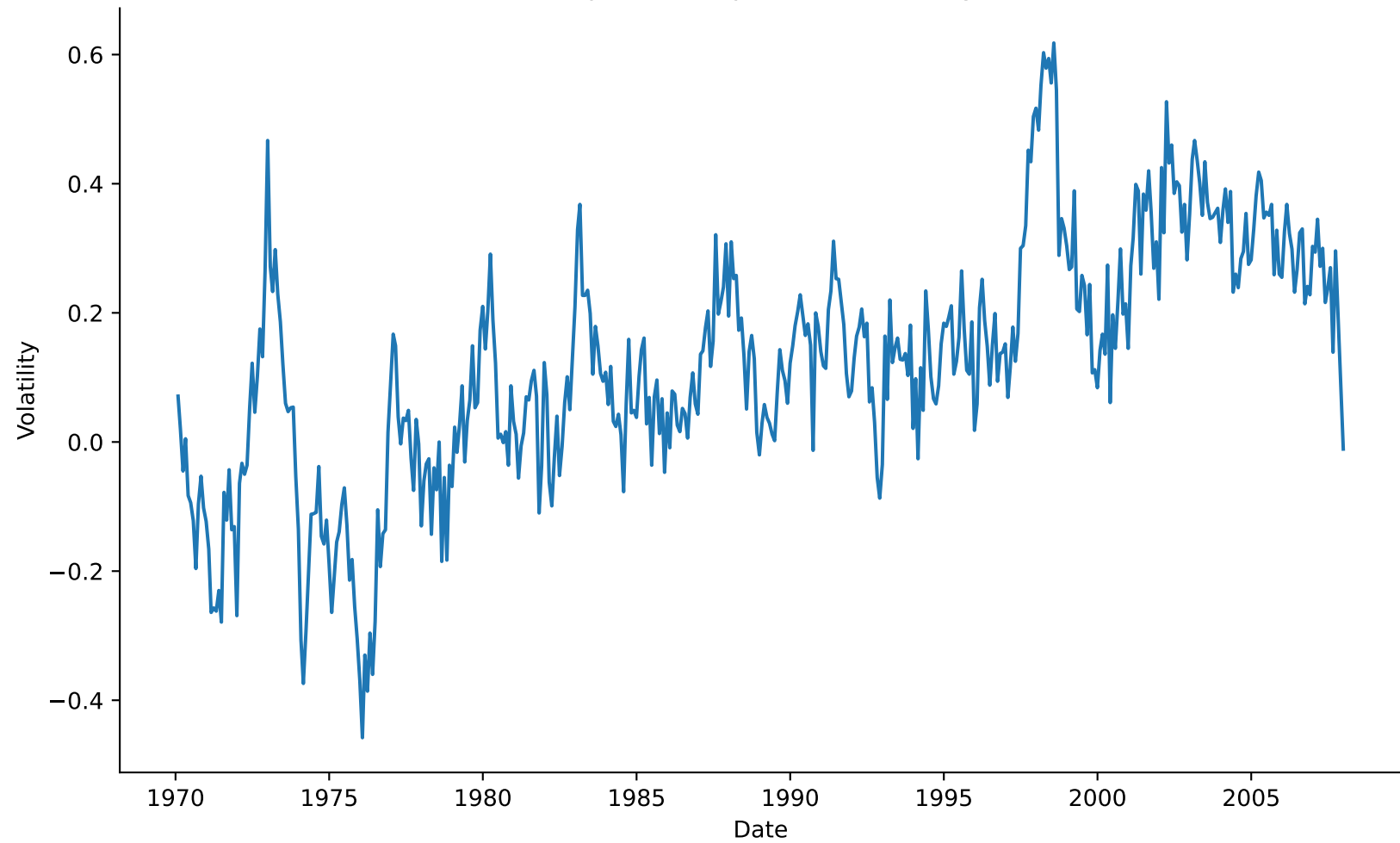
Southern Hemisphere Temperature Volatility - Sub-series
