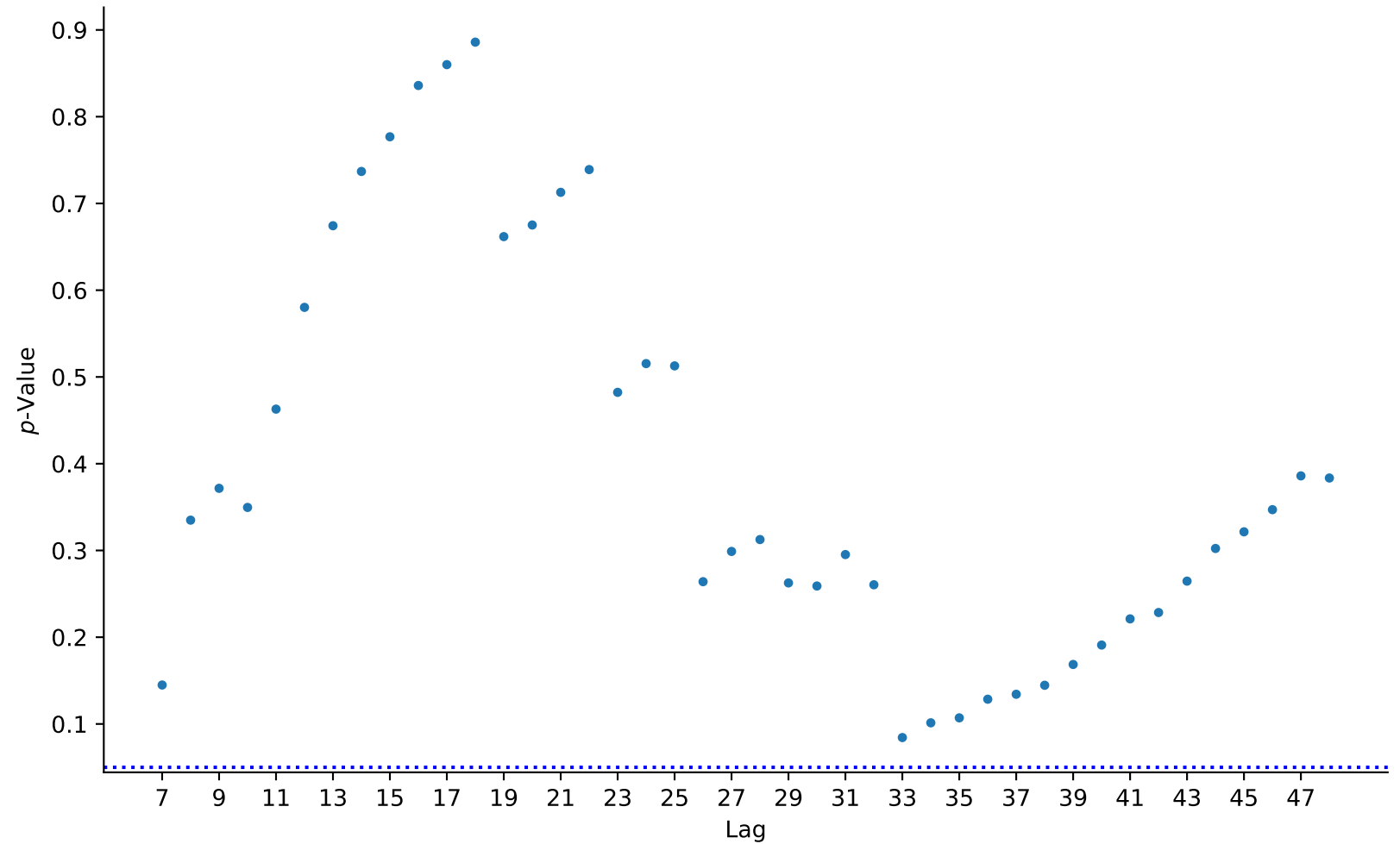
Ljung-Box p-values: SARIMA(2,1,[2,4])(0,1,2)12
