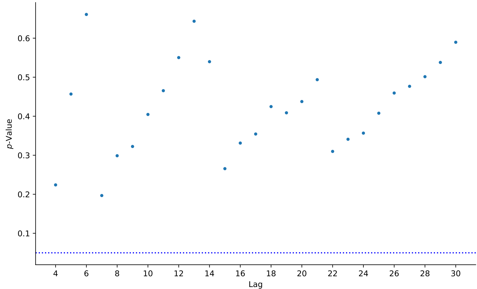
Ljung-Box p-values: ARMA(2,[4]) on HSR residuals
