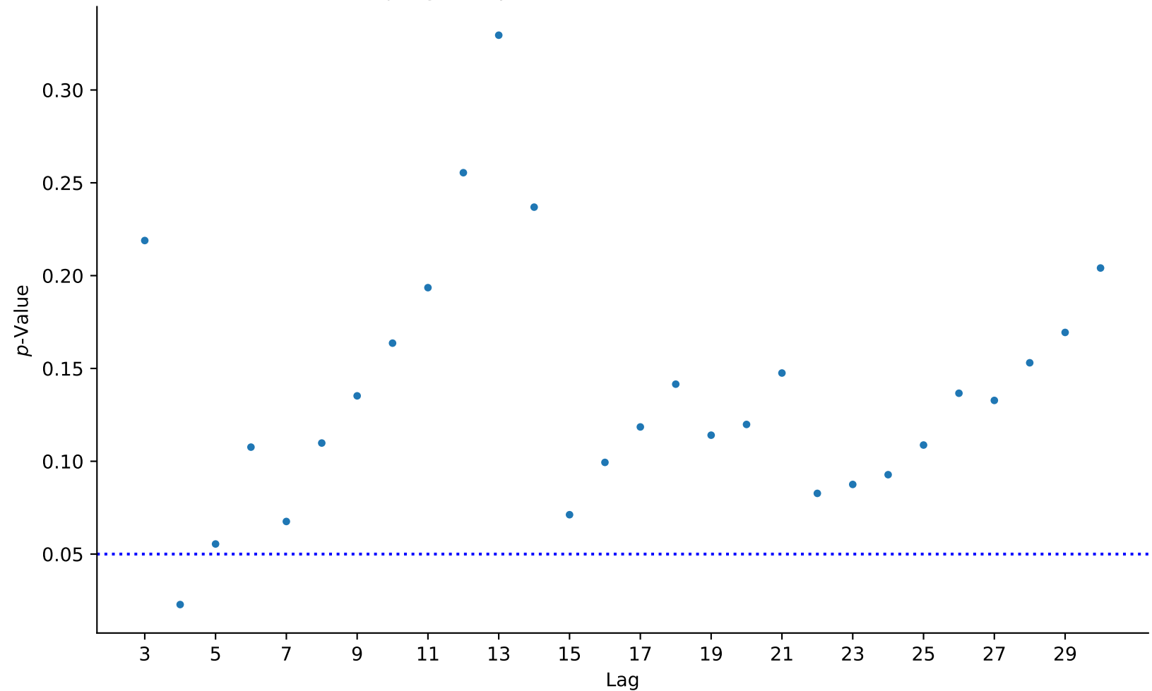
Ljung-Box p-values: AR(2) on HSR residuals
