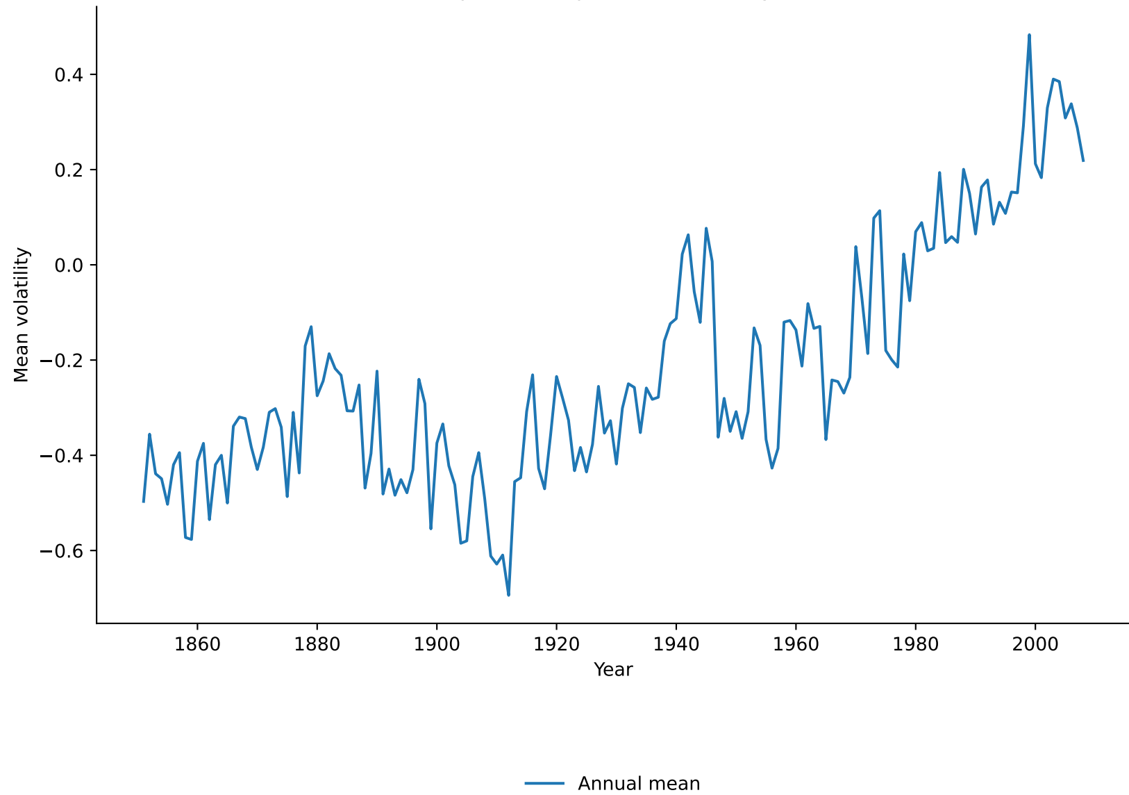
Southern Hemisphere Temperature Volatility - Annual Mean
