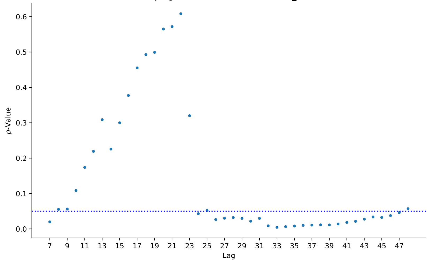
Ljung-Box P-values: (0,0,5)(0,1,1)_12
