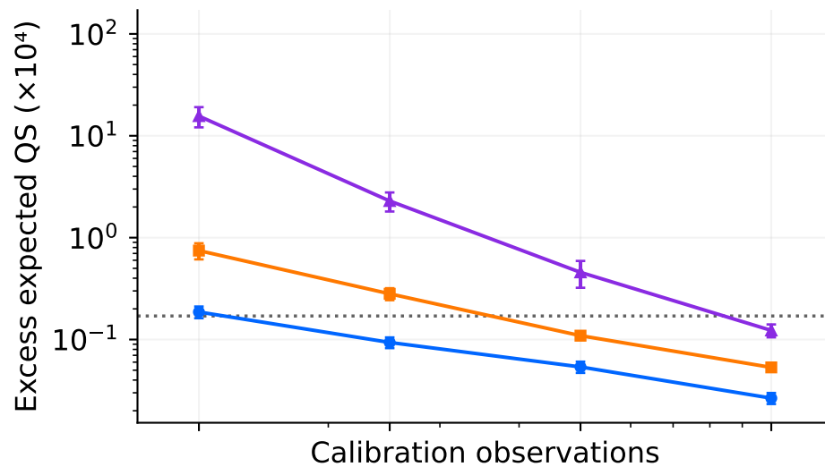
(c) Student-t(5): constant distortion
