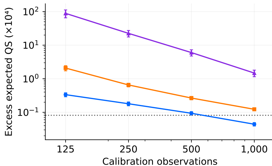
(c) Student-t(5): constant distortion
