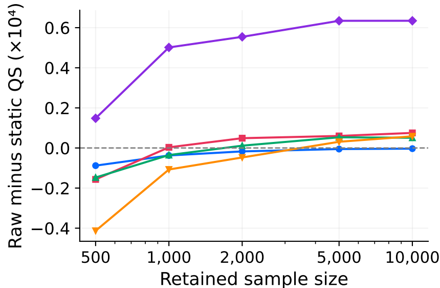
(b) Gain in Quantile Score
