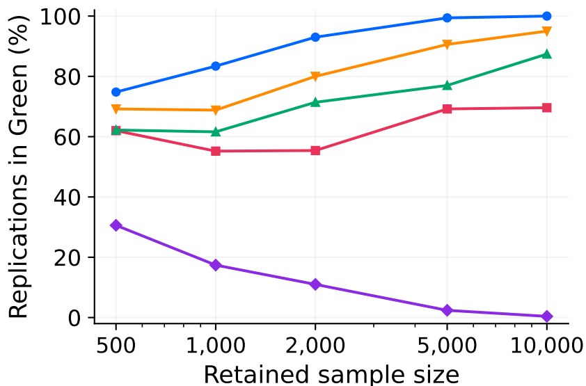
(c) Raw forecasts in Green
