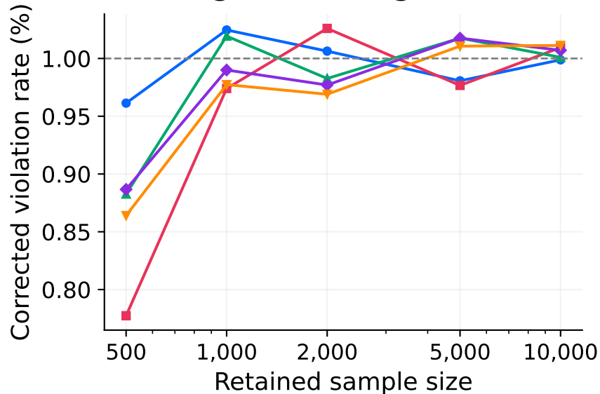
(a) Marginal coverage
