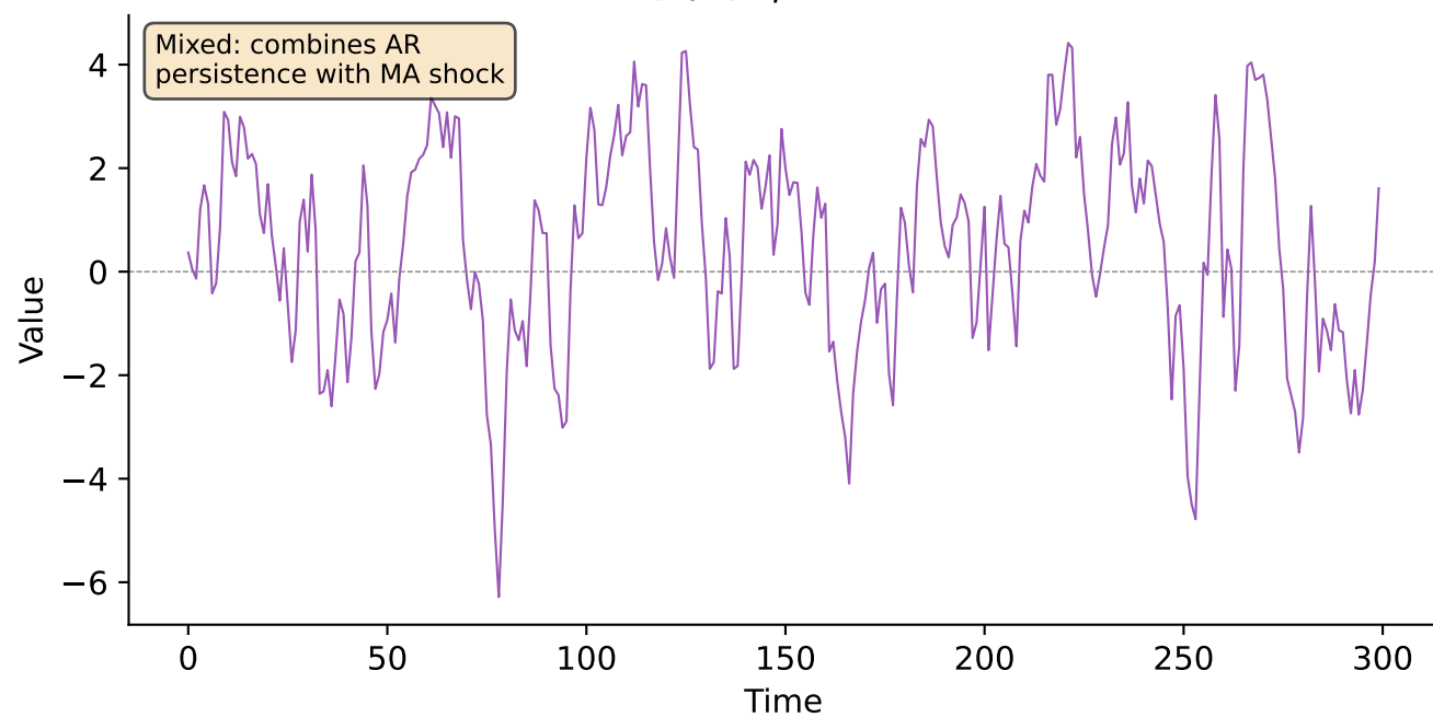
ARMA(1,1) \phi = 0.7, \theta = 0.5
