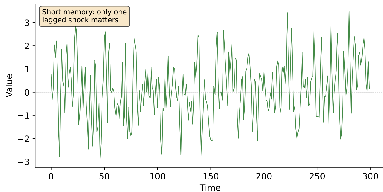
MA(1) \theta = 0.8
