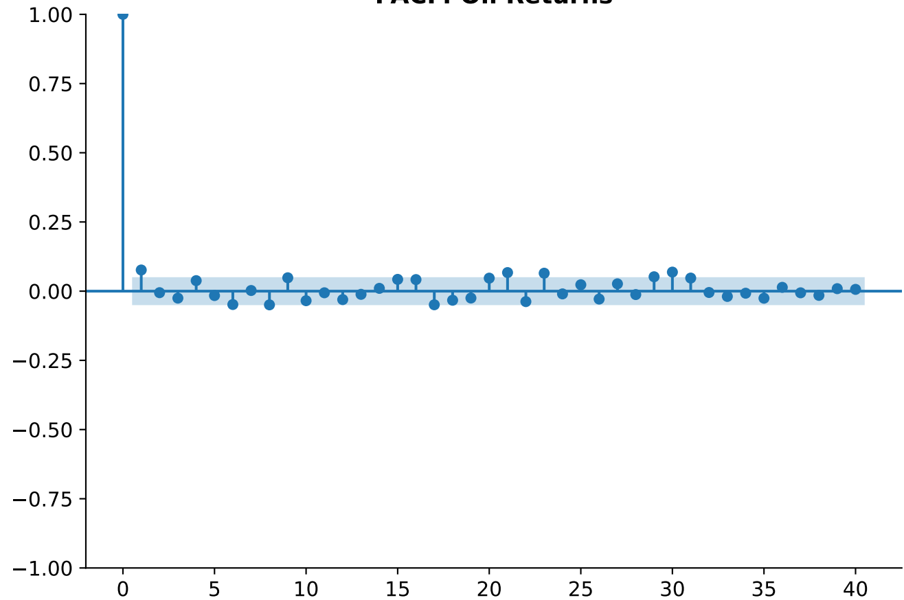
PACF: Oil Returns
