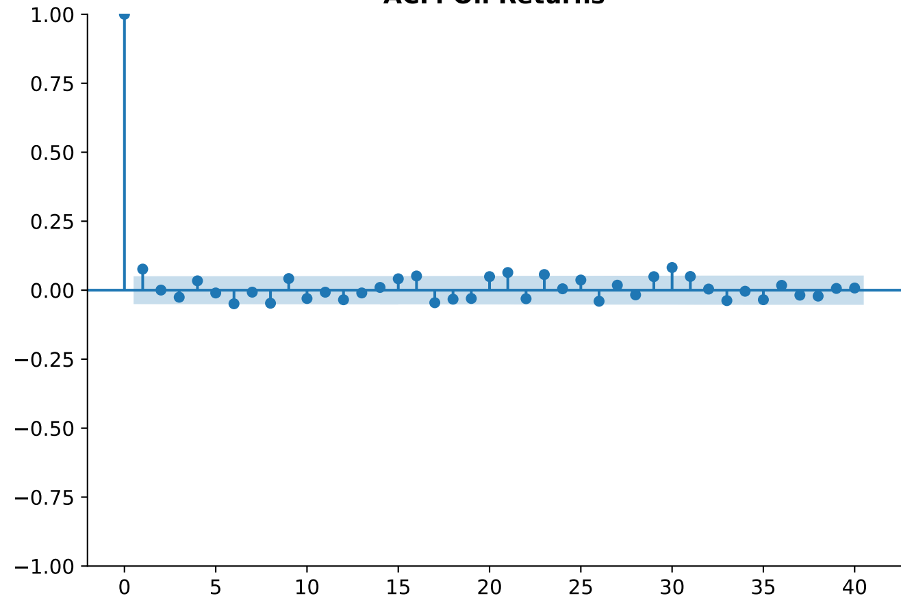
ACF: Oil Returns
