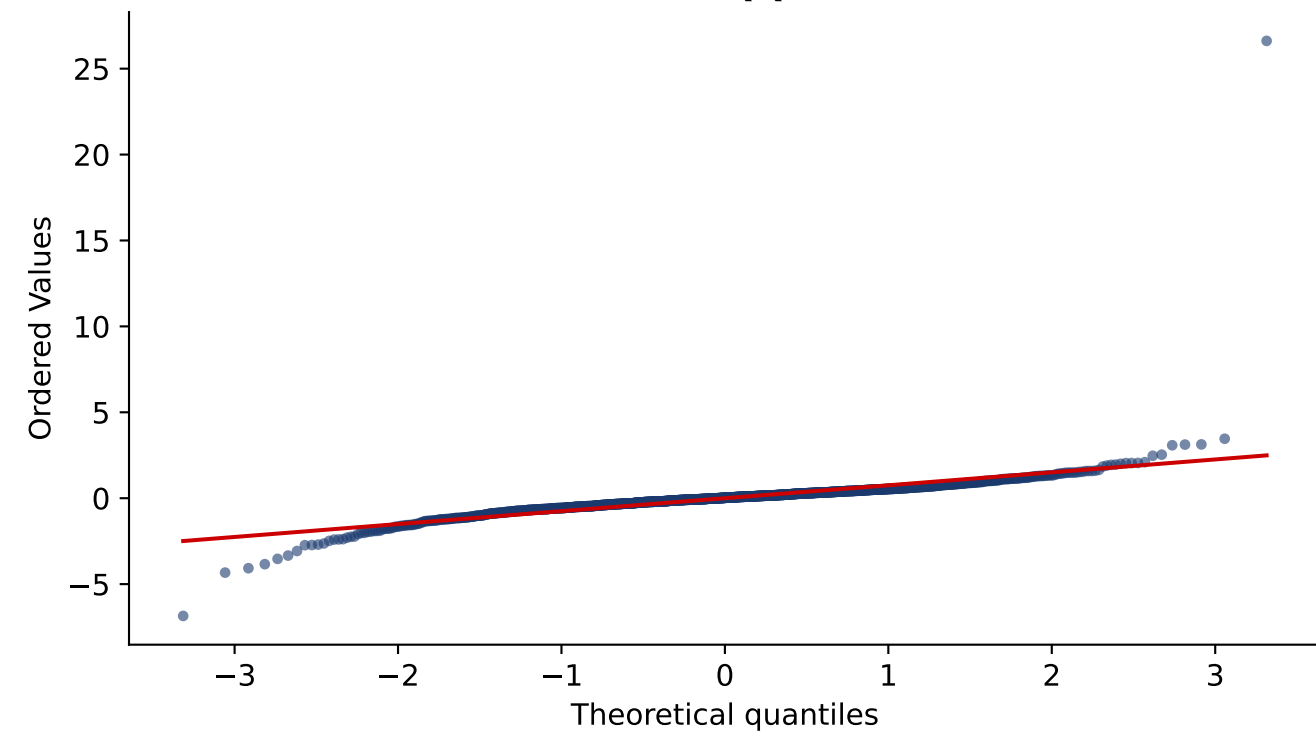
Normal QQ-Plot
