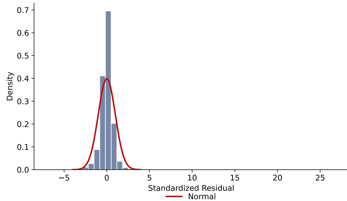
Residual Distribution
