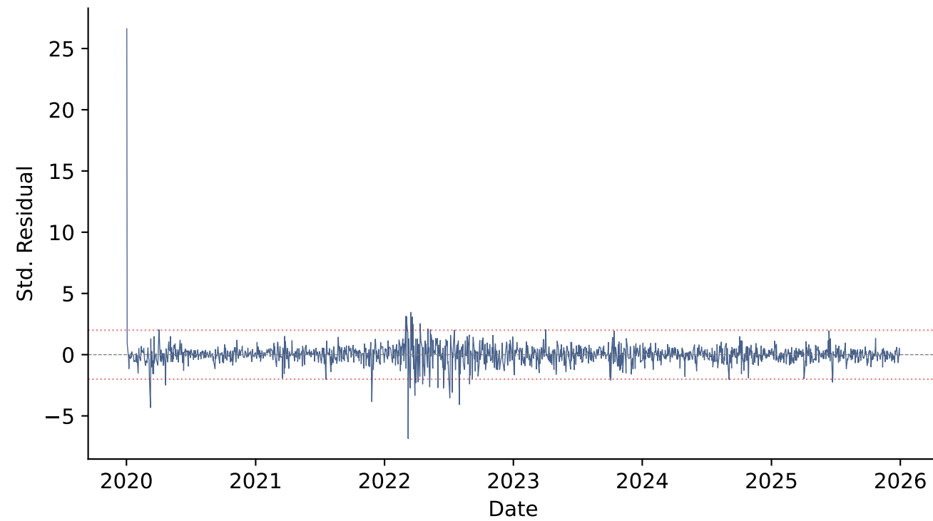
Standardized Residuals
