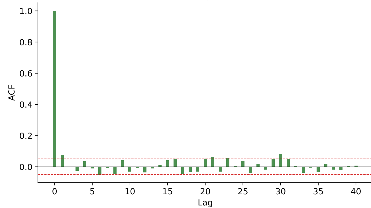
ACF of Log Returns
