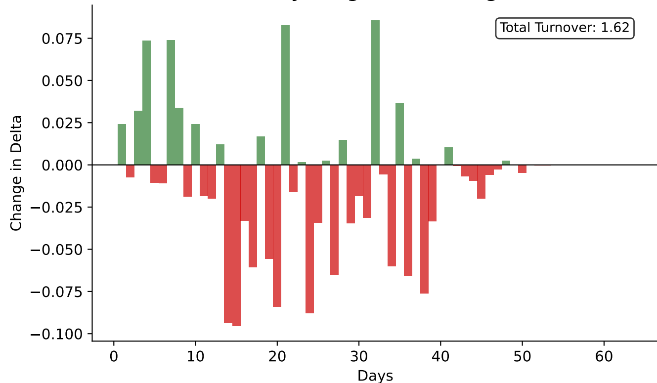
Daily Hedge Rebalancing
