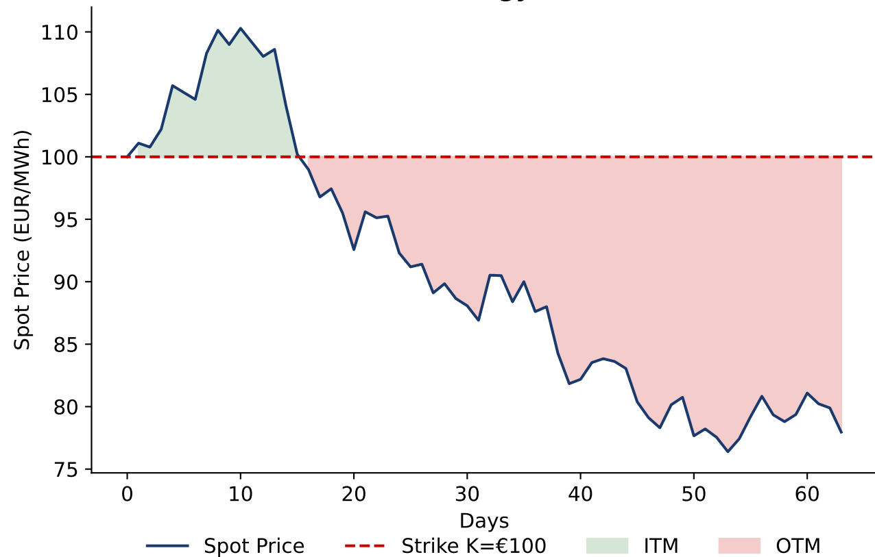
Simulated Energy Price Path
