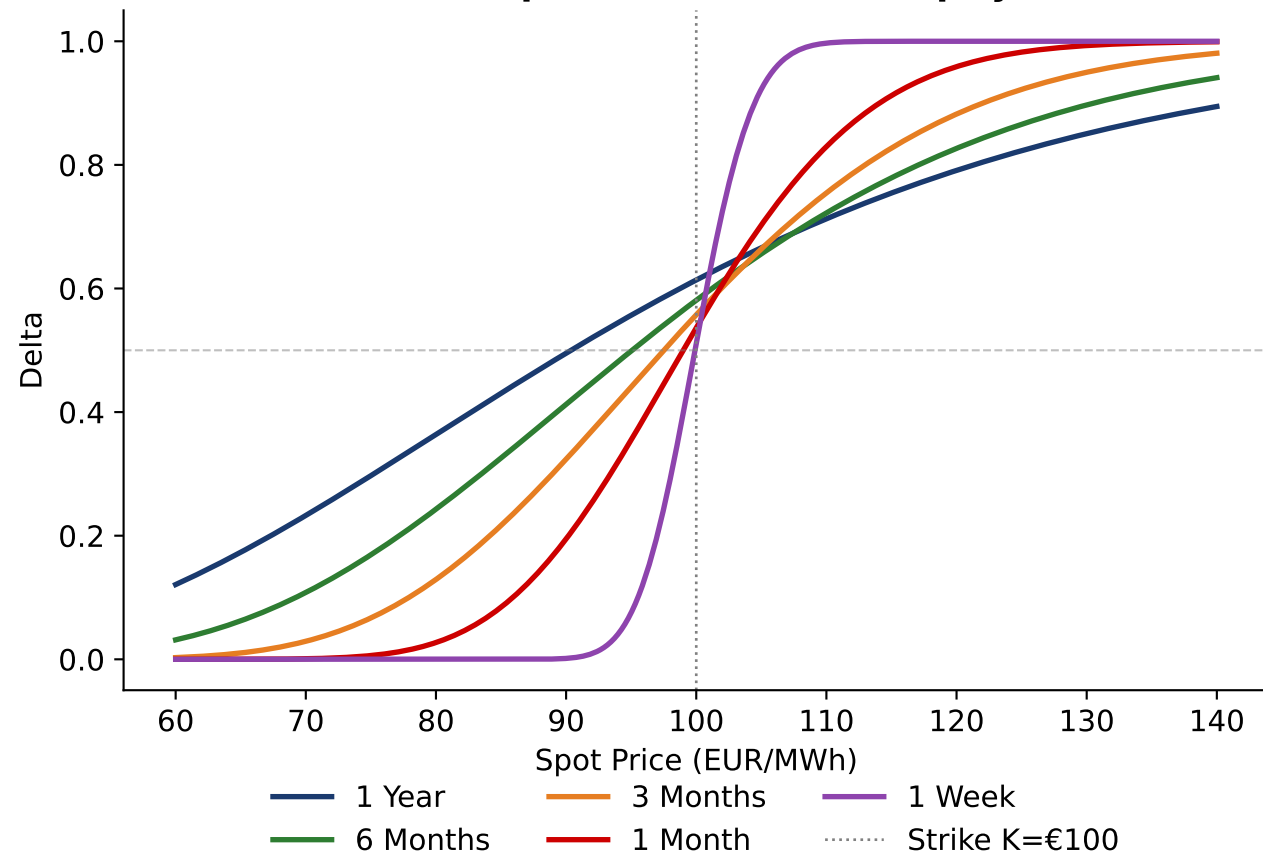
Call Delta vs Spot Price (Time to Expiry Effect)
