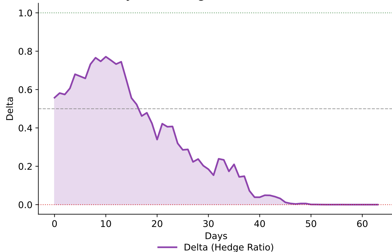
Dynamic Hedge Ratio Over Time
