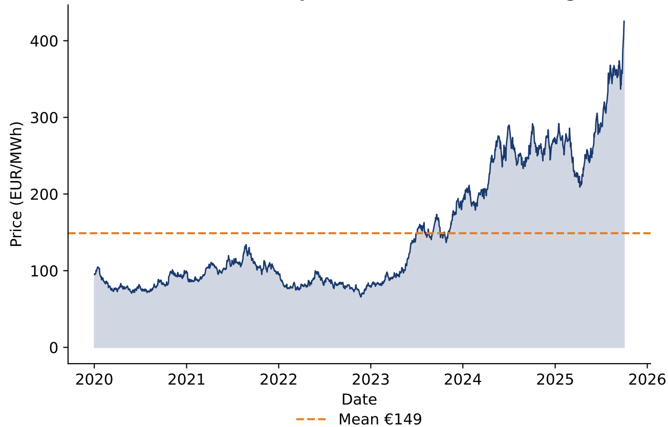
Simulated Gas Spot Prices (Mean-Reverting)
