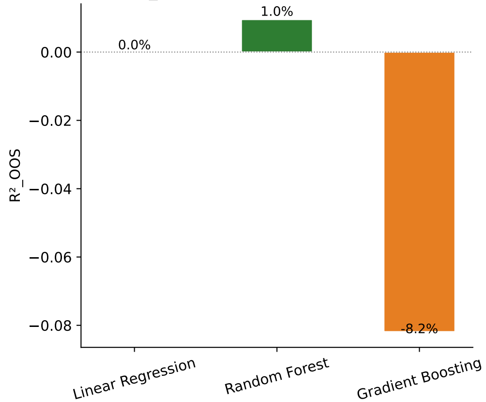
R 2 _OOS vs Naive (higher is better)
