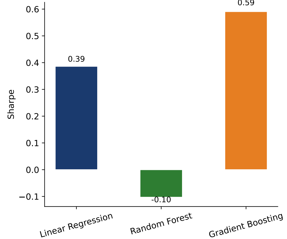
Sharpe Ratio (higher is better)
