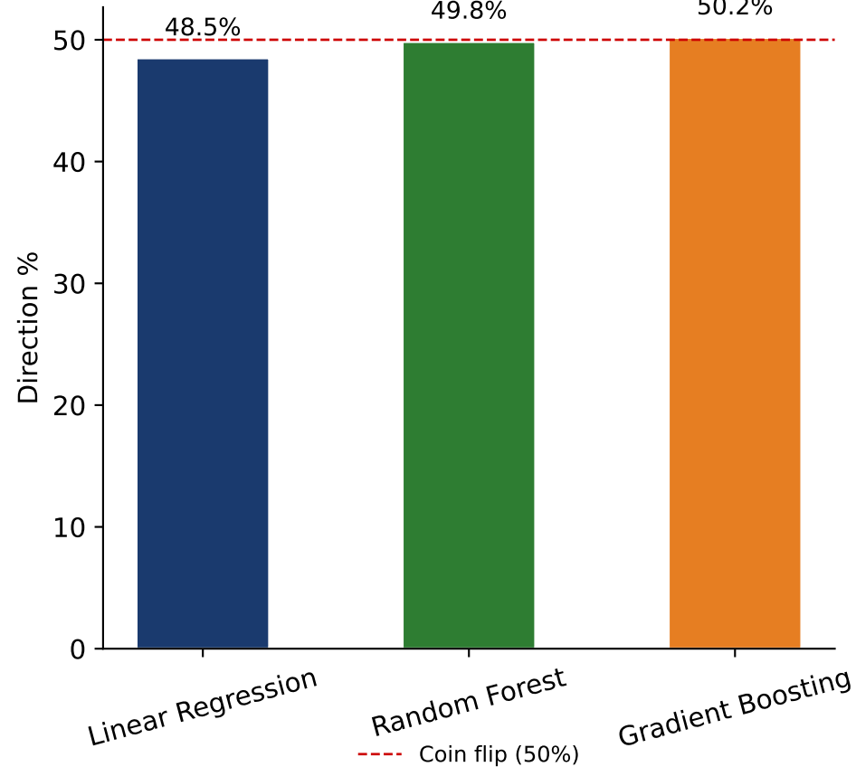
Direction Accuracy % (higher is better)
