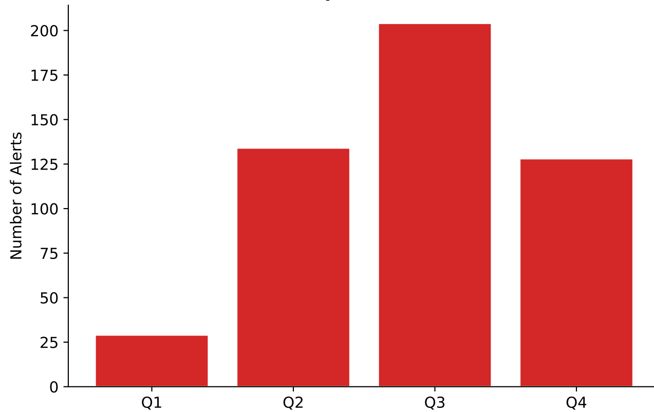
Concept Drift Alerts
