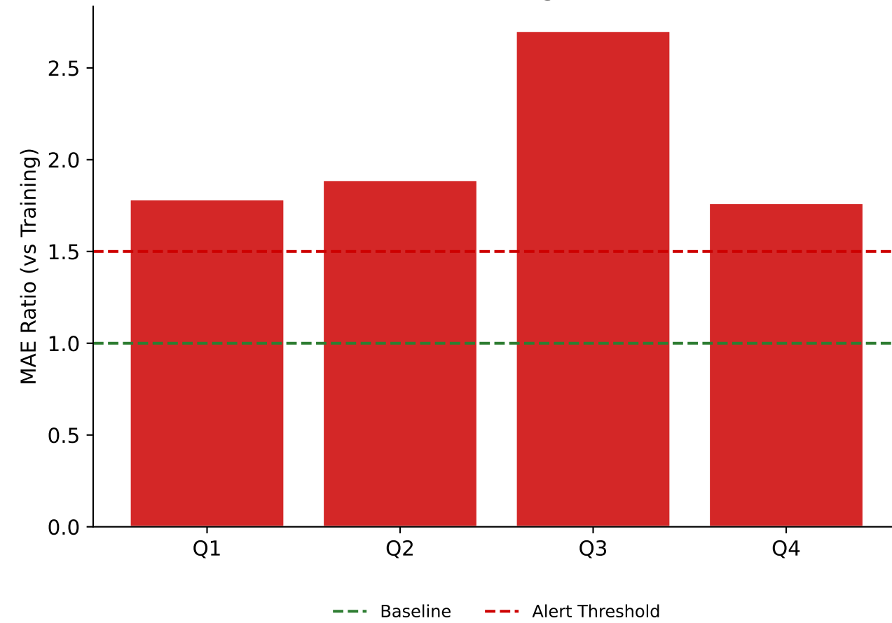
Concept Drift Alerts
