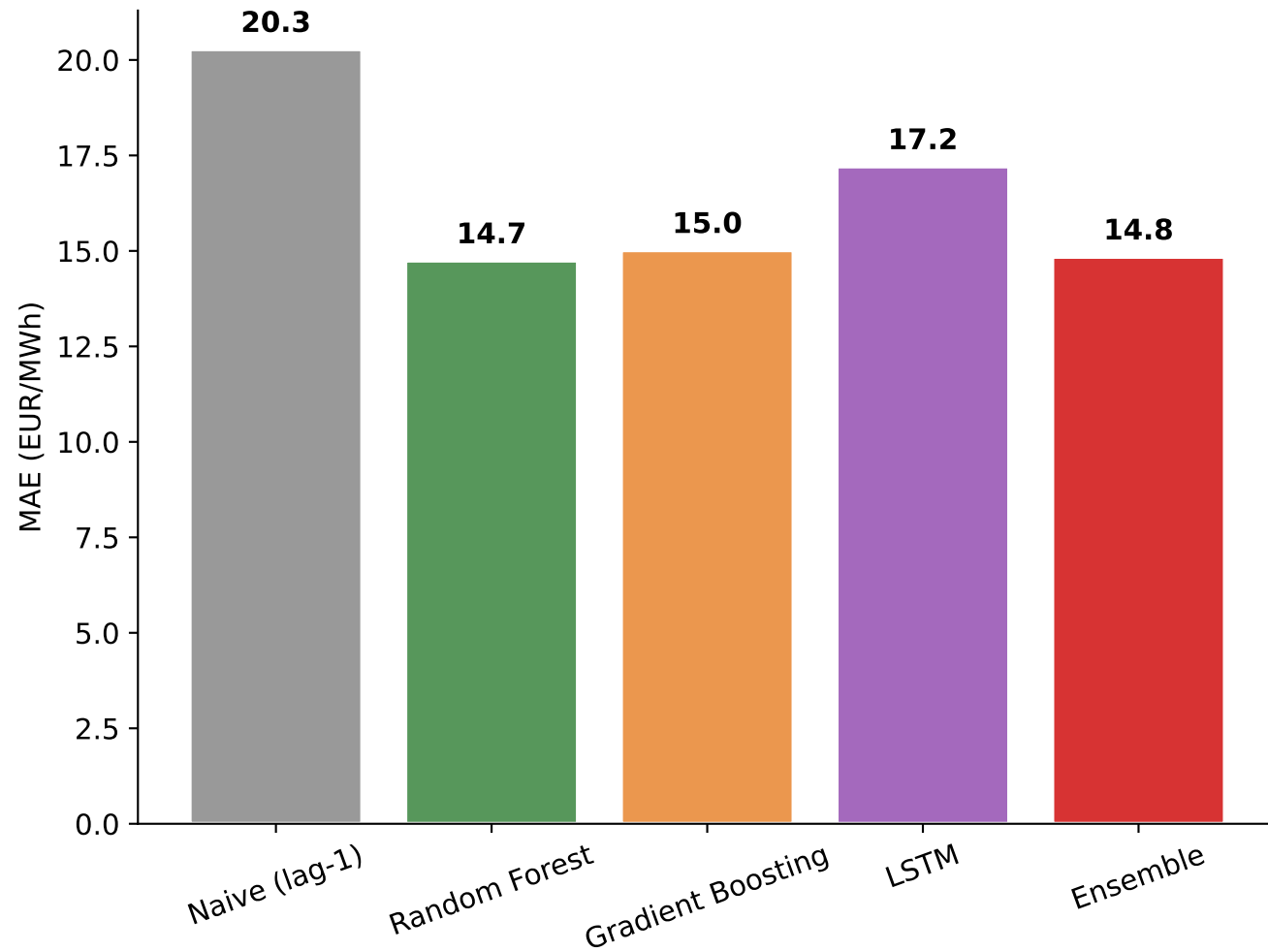
(A) Mean Absolute Error
