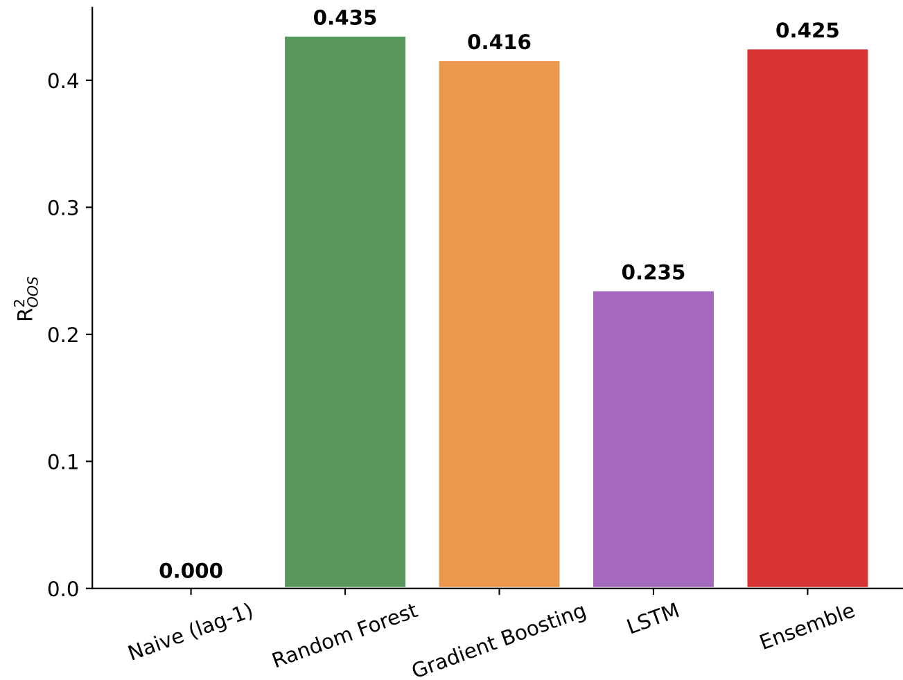
(B) Coefficient of Determination
